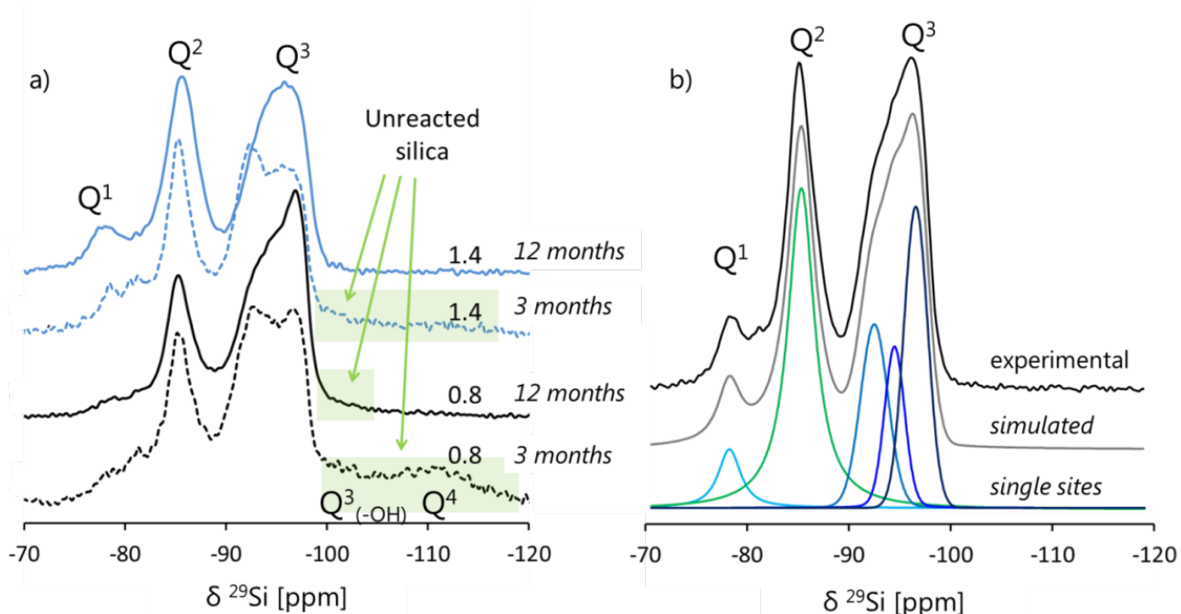
Figure 11: a) ^{29}\text{Si} MAS NMR spectra with assignments of single sites of M-S-H samples ( \text{Mg}/\text{Si}=0.8 and 1.4 ) after 3 and 12 months, the shaded regions assign unreacted silica species, b) example of the deconvolution (sample \text{Mg}/\text{Si}=1.0 , after 12 months) of the indicated single sites listed in Table 9.
