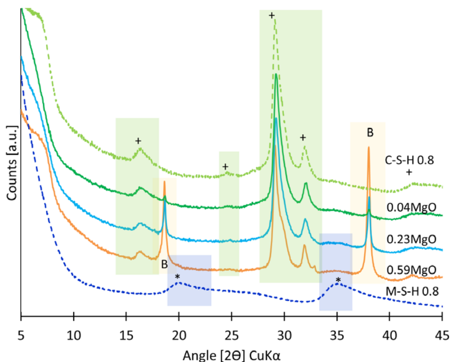
Figure 51: XRD patterns of C-S-H samples where MgO has been added: 0.04MgO, 0.23MgO and 0.59MgO after 1 year of curing at 20°C, patterns of M-S-H 0.8 and C-S-H 0.8 shown as references (B=brucite (Mg(OH) 2 ), +=C-S-H, *= M-S-H).
