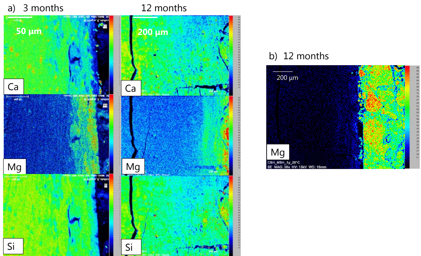
Figure 71: a) EDS elemental mapping of the C-S-H near the interface (zoom A as detailed in Figure 70) and b) magnesium enrichment in C-S-H compared to the M-S-H disk (colors were normalized to the lowest and the highest content).
