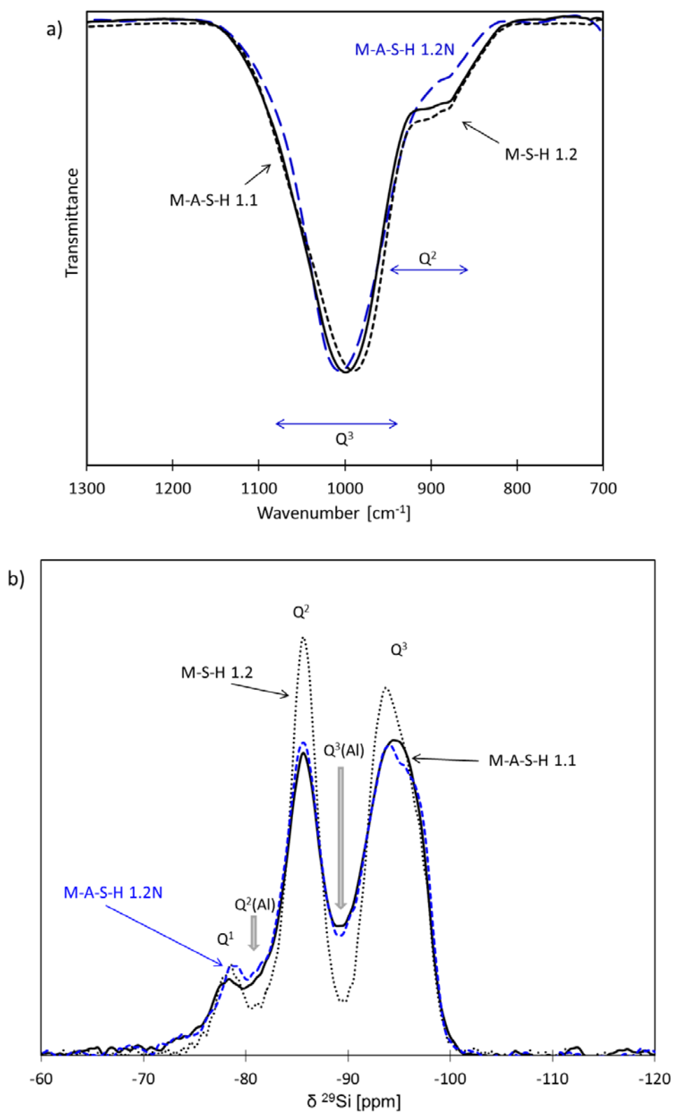
Figure 94: a) FTIR and b) ^{29}\text{Si} MAS NMR spectra of the samples from M-A-S-H and M-A-S-H N with initial \text{Mg}/\text{Si}=1.1 -1-2 and \text{Al}/\text{Si} = 0.1 cured 1 year at 50^\circ\text{C} .
