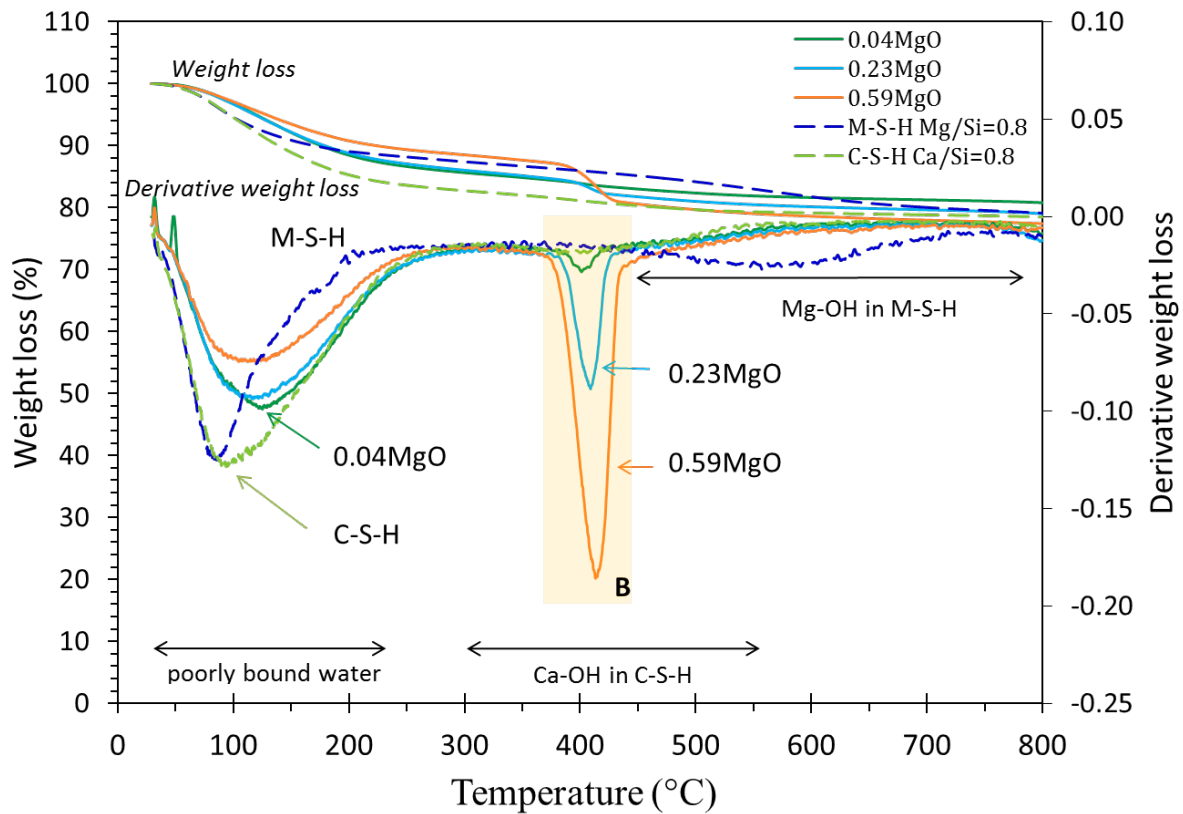
Figure 52: Thermogravimetric analysis of C-S-H samples where MgO has been added: 0.04MgO, 0.23MgO and 0.59MgO after 1 year of curing at 20°C, patterns of M-S-H 0.8 and C-S-H 0.8 shown as references. B=brucite ( Mg(OH)_2 ).
