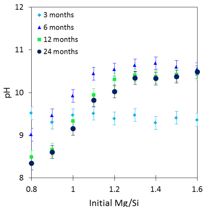
Figure 9: Evolution of pH values at 20°C over time as function of initial \text{Mg/Si} ratio (0.8-1.6).
