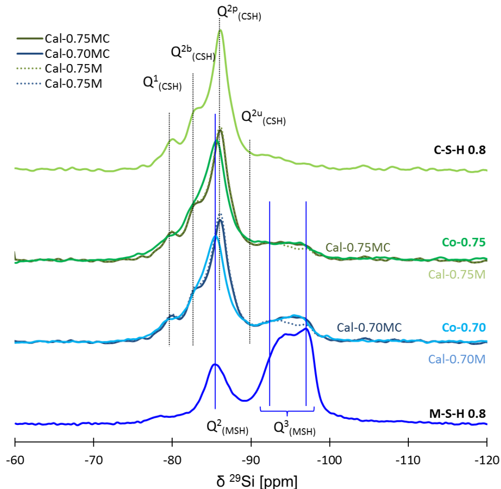
Figure 66: ^{29}\text{Si} MAS NMR spectra of Co-0.70 and Co-0.75 samples (1 year at 50^\circ\text{C} ) compared to spectra of C-S-H 0.8, M-S-H 0.8 and the calculated samples with M-S-H 0.8 (Cal-0.70M, Cal-0.75M) and with Co-0.05 (Cal-0.70MC, Cal-0.75MC).
