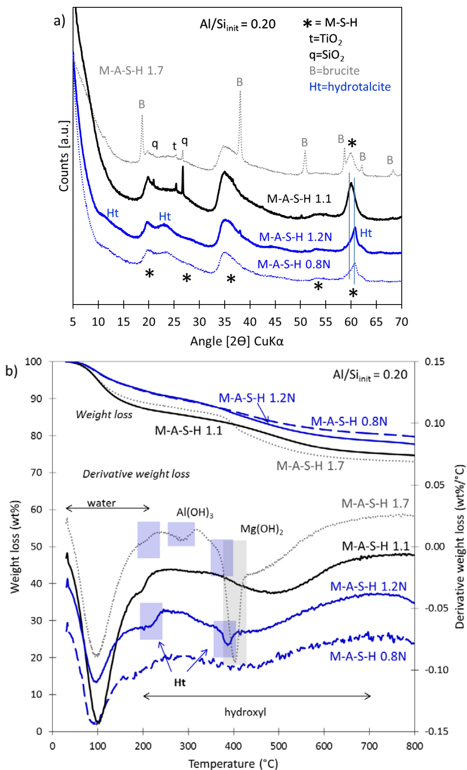
Figure 95: a) XRD patterns and b) TGA curves and derivatives associated with M-A-S-H samples with initial \text{Al/Si} = 0.20 cured 1 year at 50^\circ\text{C} .
