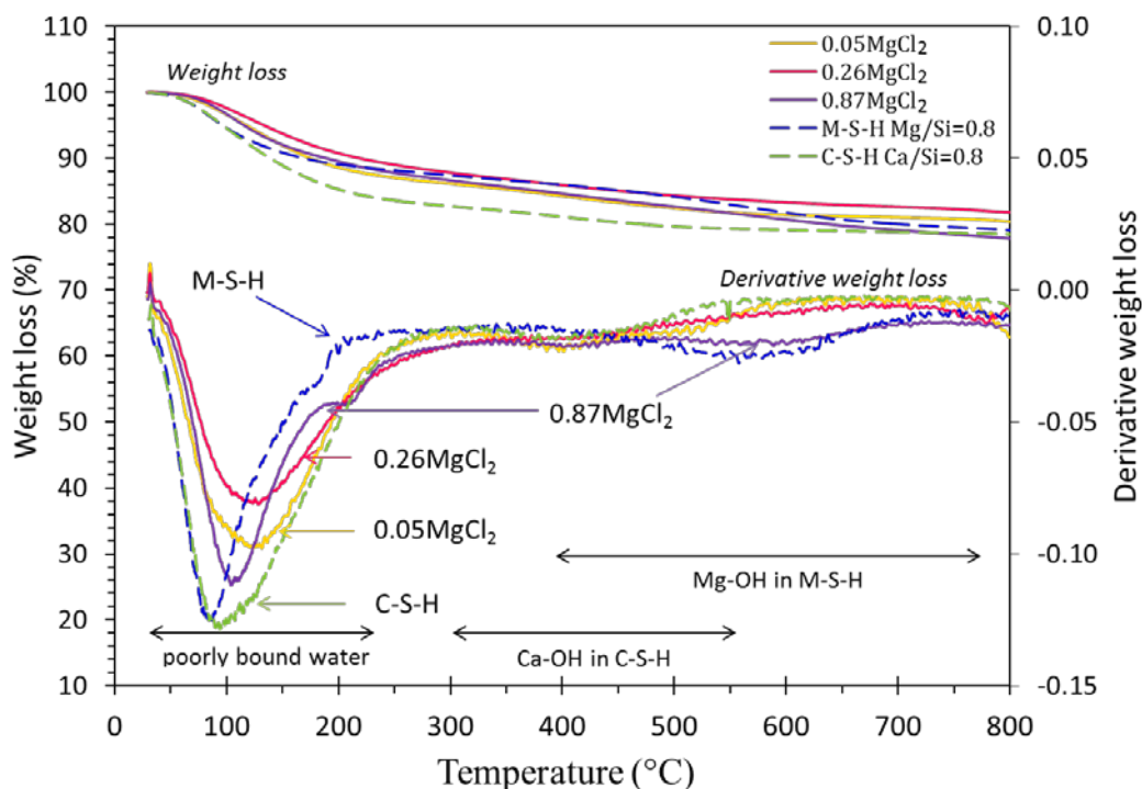
Figure 45: Thermogravimetric analysis (TGA) of C-S-H samples where \text{MgCl}_2 has been added: 0.05 \text{MgCl}_2 , 0.26 \text{MgCl}_2 and 0.87 \text{MgCl}_2 (solid lines) after 1 year of curing at 20 °C, TGA of M-S-H 0.8 and C-S-H 0.8 (dashed lines) are shown as references.
