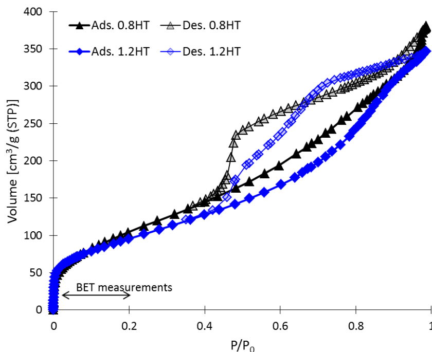
Figure 31: N_2 absorption-desorption isotherms of the hydrothermally treated M-S-H.
