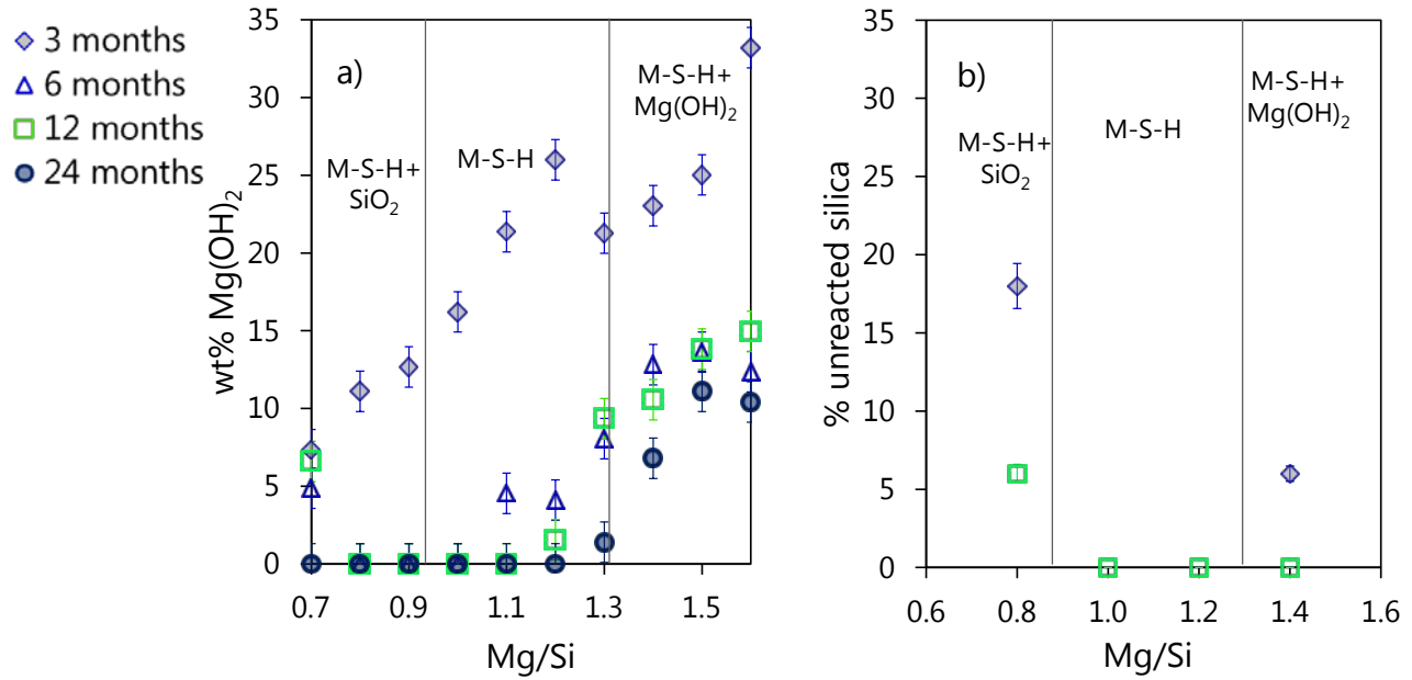
Figure 14 : Amount of a) brucite (from TGA) (wt.% of brucite normalized to 100g dry mass) and b) unreacted silica (from ^{29}\text{Si} MAS NMR) per total of silica in samples cured at 20^\circ\text{C} as a function of the initial \text{Mg/Si} and time. Vertical lines separate the area where i) silica + M-S-H, ii) M-S-H only and iii) M-S-H + brucite are present after long reaction times.
