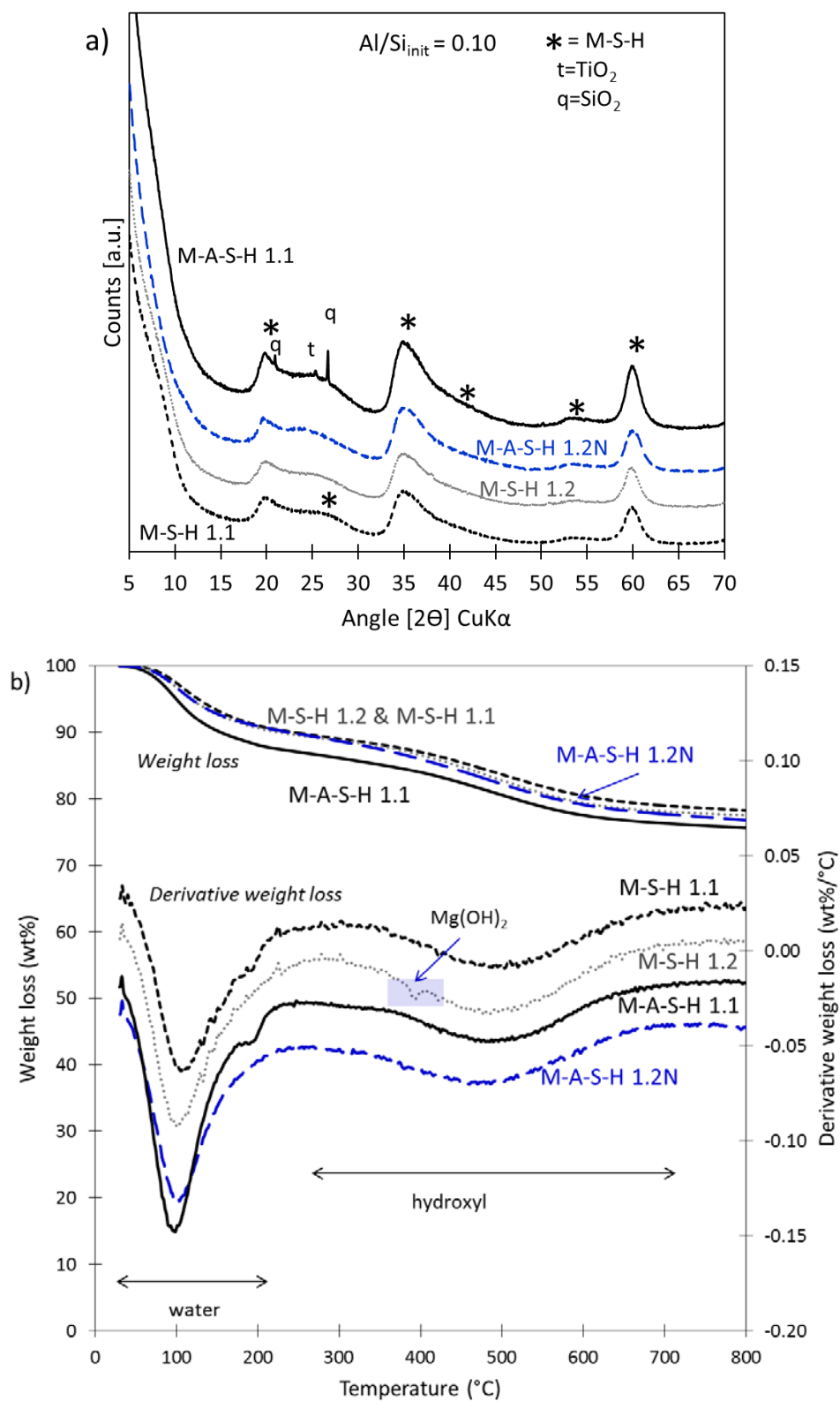
Figure 93: a) XRD patterns and b) TGA of the samples from M-A-S-H and M-A-S-H N with initial \text{Mg/Si}=1.1\text{-}1.2 and \text{Al/Si} = 0.1 cured 1 year at 50^\circ\text{C} .
