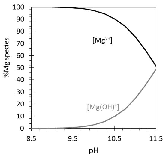
Figure 44: Distribution of magnesium speciation ( \text{Mg}_{\text{tot}} = 100 \text{ mol/l} ) in solution at 20°C as a function of the pH.
