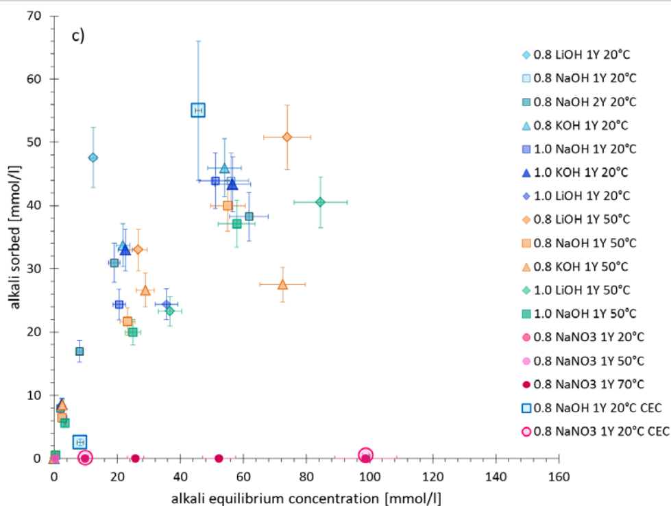
Figure 92: Alkalis uptake in M-S-H (Mg/Si=0.8 and Mg/Si=1.0) as a function of a) the initial alkali concentration (measured); b) the alkali concentration at equilibrium (measured) c) sorption isotherms, the results for LiOH, NaOH, KOH were calculated from mass balance (indirect method), the results for NaNO 3 were calculated from dissolution (direct method).
