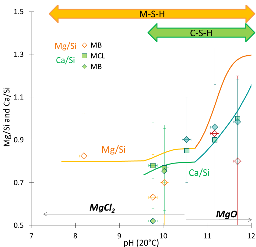
Figure 56: Evolution of atomic ratios calculated by GEMS and comparison with the ratios obtained experimentally (from MCL ^{29}\text{Si} MAS NMR, Table 3 & Table 7), and from MB, mass balance (Table 24 & Table 27)).
