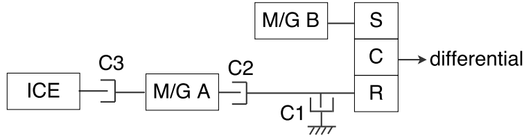
Fig. 2.12 – General Motors Range Extender (GM RE) hybrid powertrain with the 2ET50 transaxle [5]
