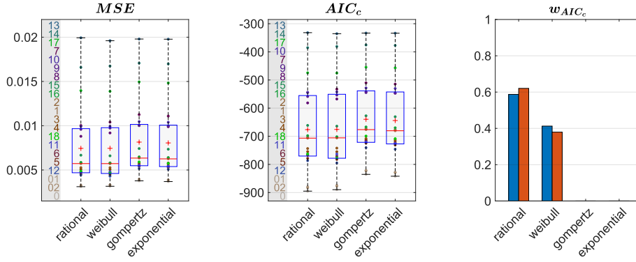
Figure 5.6: Goodness of fits for each candidate to model the ouputed scaling factors averaged in the 3 directions. Boxplots are performed along the ROIs, ROI IDs are displayed on the left. Akaike weights are computed on mean (blue) and median (red) AIC_c
