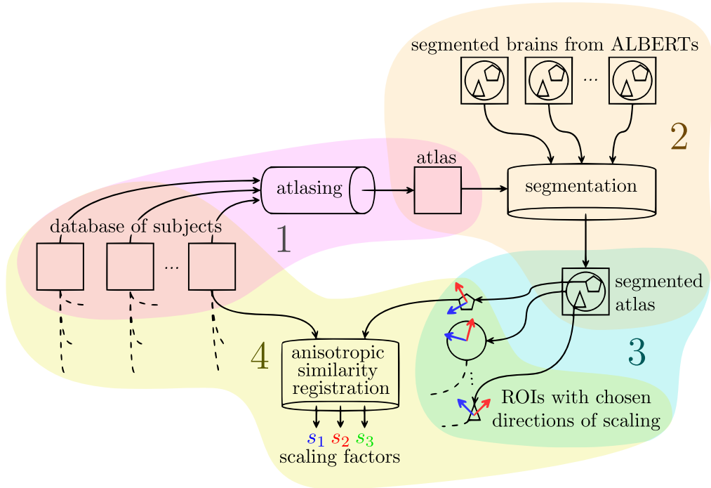
Figure 5.3: Pipeline for the extraction of scaling factors of a database of subjects using anisotropic similarity registration onto an atlas based on them as common reference image.
