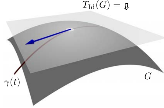
Figure 2.3: A Lie groupe: G , its tangent space at identity (associated Lie algebra): \mathfrak{g} , and a one-parameter subgroup on G : \gamma .
