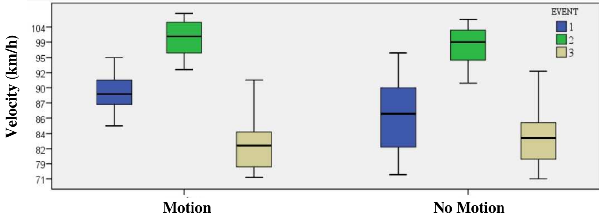
Figure 50. Velocity during each event at condition with ACC OFF
