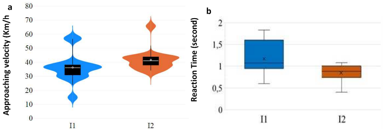
Figure 6.a Driver's approaching velocity ( V_{TB} ); b Driver reaction time (RT)
