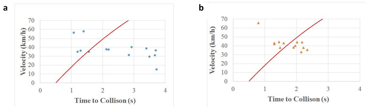
Figure 7.a TTC versus velocity at via Azzurra (I1); 4.b TTC and velocity at via Mainoldi (I2)
