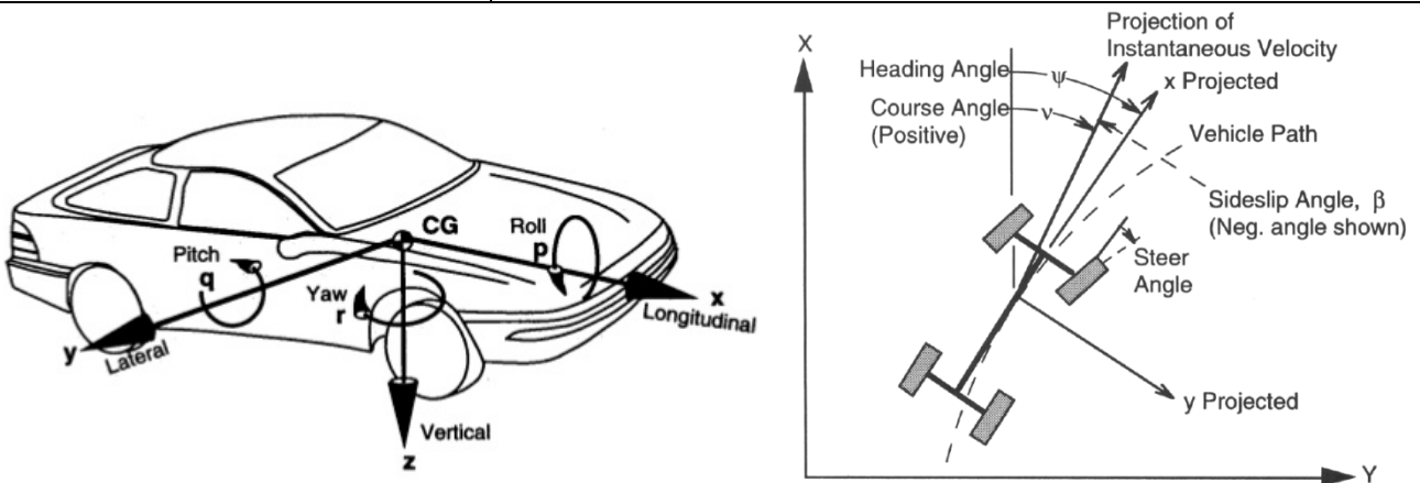
Figure 8.a. Vehicle Fixed Coordinate System; b. Earth Fixed Coordinate System.
