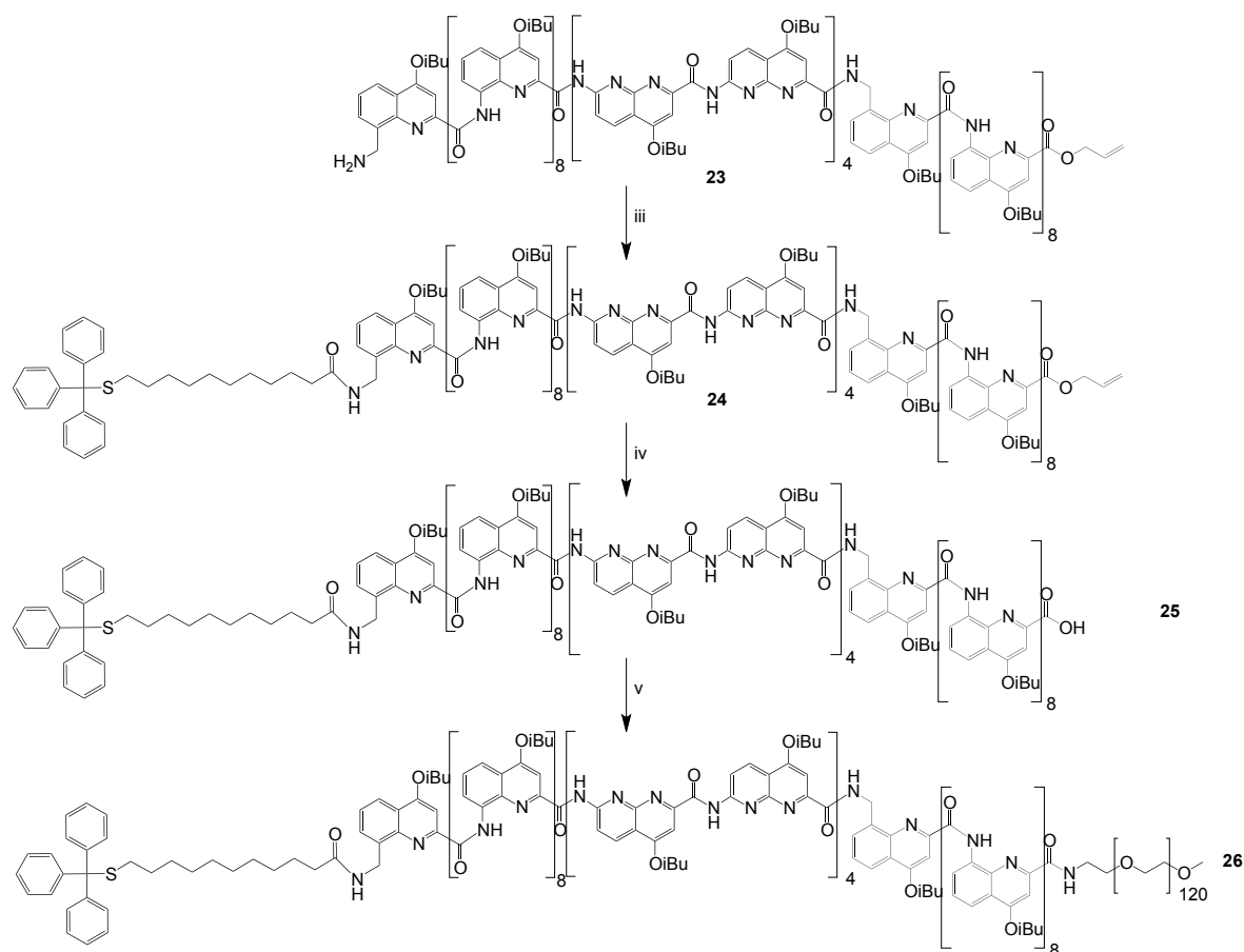
Scheme 7: Representation of the synthesis of the functionalization of the extremities of Tr-S- m QQ 8 -N 8 - m QQ 8 -PEG iii) Trityl-S-(CH 2 ) 10 -COOH, DIEA, PyBOP, CHCl 3 , RT; iv) Pd(PPh 3 ) 4 , PhSiH 3 , degassed CH 2 Cl 2 , RT; v) H 2 N-PEG-OMe, DIEA, PyBOP, CHCl 3 , RT. The reaction molar yields could not be measured.
