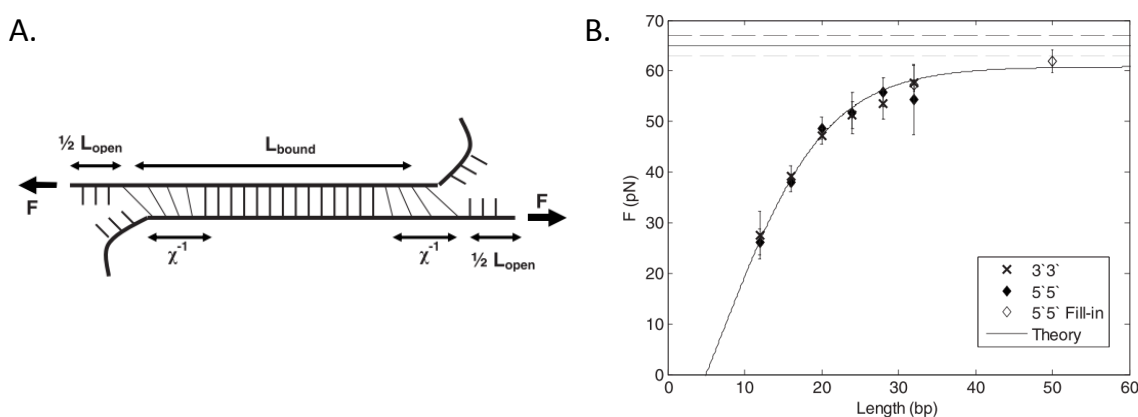
Figure 1.34 (A) Schematic of a 3'3' pulling experiment and localization of the bp ( X^l ) affected by the shear force. (B) Plot of the shear force as a function of the bp number. Adapted from reference 150.
