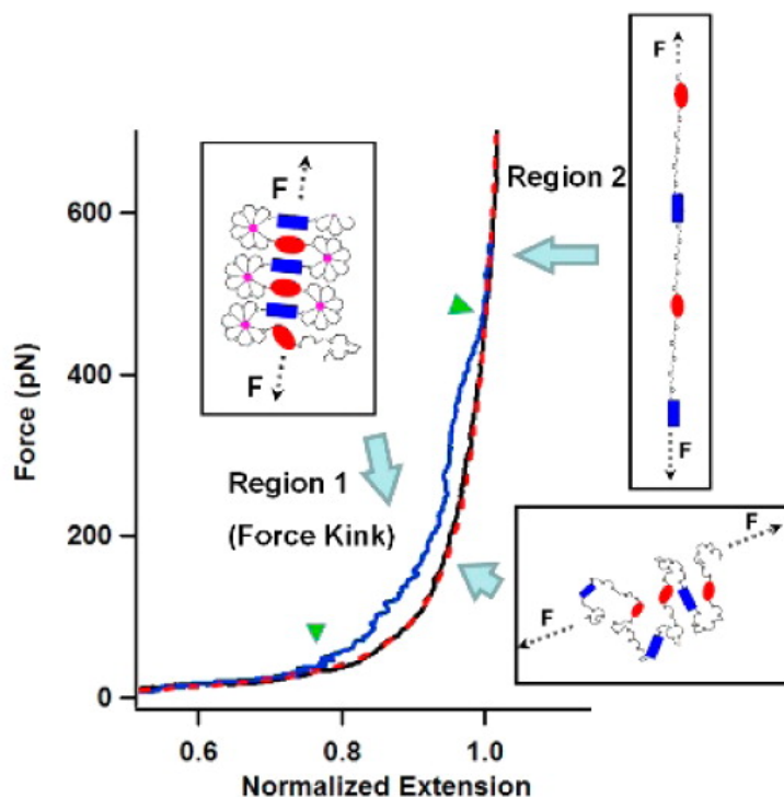
Figure 4.2 Normalized force-extension curves (normalization force: 500 pN) for the donor (dialkoxynaphthalene)–acceptor (pyromellitic dianhydride) foldamer (DA) in DMSO (black colour) and in KSCN saturated solution (solvent: methanol/chloroform = 1:1, v/v) (blue colour). The red dotted line is the fitting curve of the freely coiled chains, using the WLC model with a parameter of l_p = 3.6 \text{ \AA} and L_c = 1.08 . In the frames, schematics of the conformation of the DA foldamer are illustrated for different steps of an unfolding experiment. Reproduced from reference 10.
