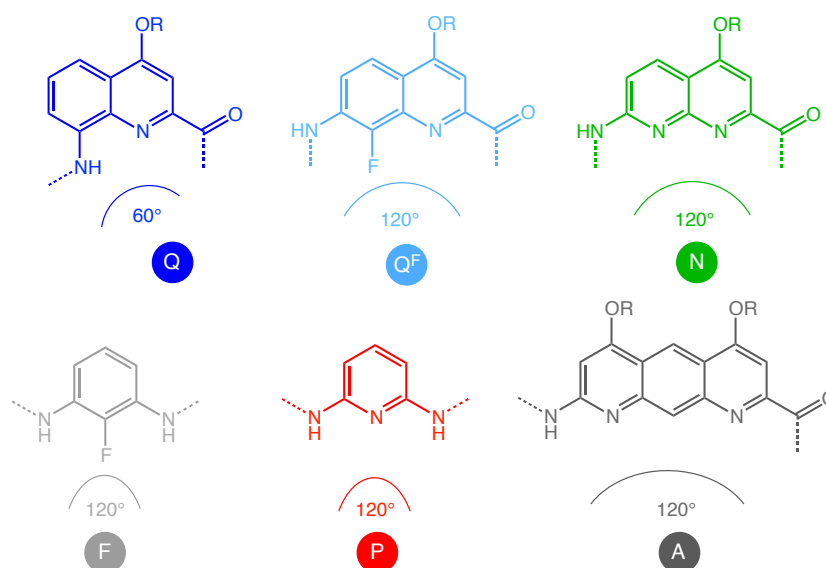
Figure 1.14 Chemical structures of some units used in aromatic oligoamide foldamers: Q (8-amino-2-quinolinecarboxylic acid), Q F (7-amino-8-fluoro-2-quinolinecarboxylic acid), N (7-amino-8-naphtyridinecarboxylic acid), F (2,6-fluorobenzene-diamine), P (2,6-pyridine-diamine), A (1,8-diazaanthracene). The lateral chain R can be replaced by hydrophobic or hydrophilic chemical function to change the solubility.
