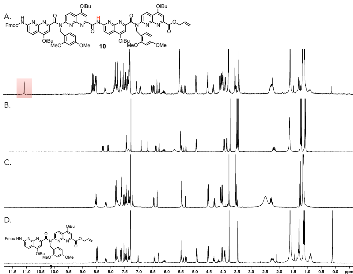
Figure 5.6 ^1\text{H} NMR spectra of (A) pure tetramer: Fmoc-[N(DMB)N] 2 -Allyl 10 , (B) Fmoc-deprotected-N 2 acid: H 2 N-N(DMB)N-Allyl 9a , (C) Allyl-ester-deprotected N 2 amine: Fmoc-N(DMB)N-COOH 9b , (D) dimer DMB-protected N 2 : Fmoc-N(DMB)N-Allyl 9 . The characteristic aromatic amide proton is highlighted in red.
