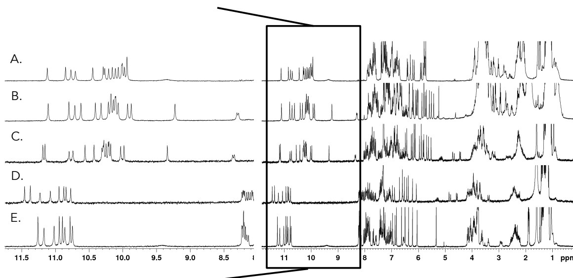
Figure 5.11 1 H NMR in CDCl 3 of (A) Tr-S-R-mQQ 16 -PEG, synthesized by Dr. Xuesong Li for this thesis. (B) Tr-S-R-mQQ 8 -mQQ 8 -PEG 34 . (C) Boc-mQQ 8 -mQQ 8 -Allyl (D) NH 2 -mQQ 8 -Allyl (E) Boc-mQQ 8 -COOH.
