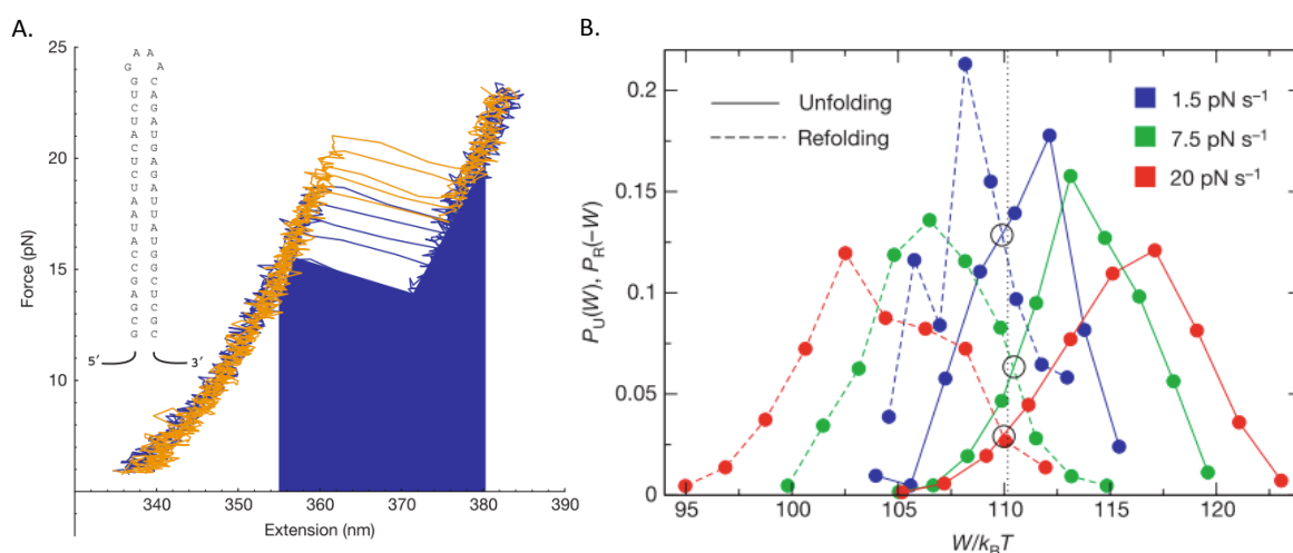
Figure 3.14 (A) Pulling (blue) and relaxing (orange) force curves of the RNA hairpin. The blue area corresponds to the work measurement ( W=F \cdot d ). The RNA sequence is shown as an inset. (B) Work distributions for RNA unfolding ( P_U -continuous lines) and refolding ( P_R -dashed lines) at three loading rates. The distributions of the different loading rates cross at the similar work value of 110 k_B T . Reproduced from reference 13.
