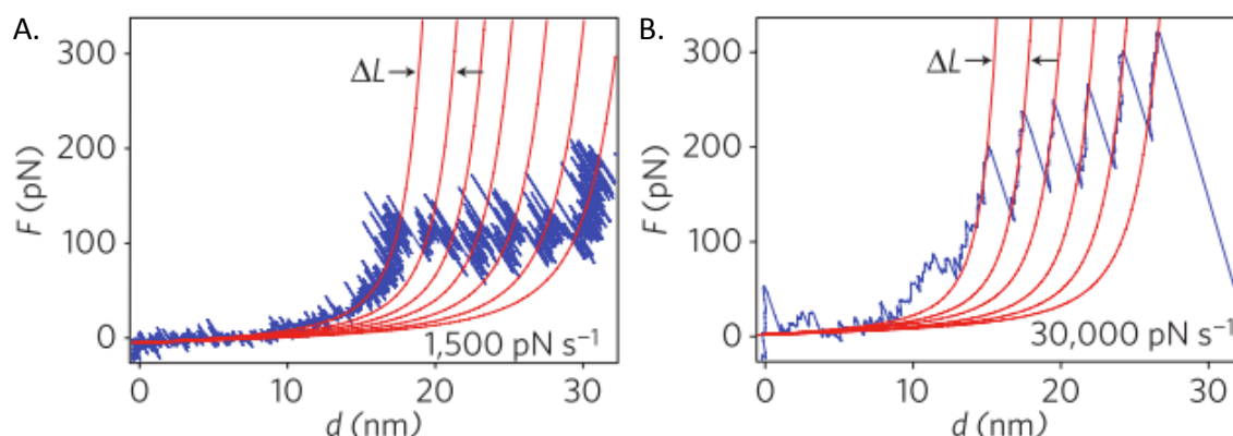
Figure 2.10 Force-distance curves of pulling experiments on oligo calix[4]arene at two different loading rates (a) 1500 pN.s -1 and (b) 30000 pN.s -1 . Adapted from reference 27.
