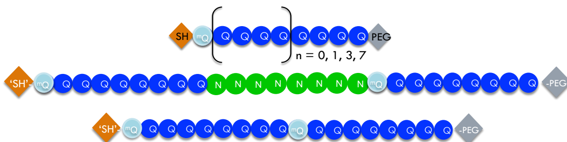
Figure 5.3: Schematic representation of (Top) Tr-S- m QQ 4n -PEG previously studied foldamers, made up of quinoline units. (centre) Tr-S-R- m QQ 8 -N 8 - m QQ 8 -PEG: new foldamer, made up of a triblock of quinoline-, naphthyridine-, quinoline-blocks; (bottom) Tr-S-R- m QQ 8 - m QQ 8 -PEG: new quinoline-based foldamer with the insertion of one amino-methyl quinoline unit in-between two Q 8 . Each foldamer is designed specifically to be adapted to SMFS experiments: addition of a thiol group at one end and a PEG chain as tether at the other end. The light blue m Q represents an amino-methyl-quinoline unit, the blue Q represents a quinoline unit, the green N represents a naphthyridine unit.
