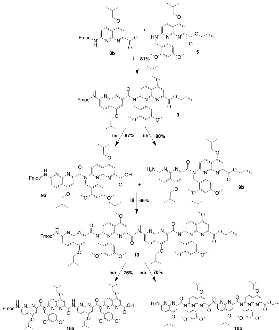
Scheme 3: Representation of the synthesis of tetramer (N(DMB)N) 4 amine 10b and tetramer (N(DMB)N) 4 acid 10a from monomer acid chloride 8 and amine 5 : i) CHCl 3 , DIEA, 0°C then RT. iiia) & ivia) DBU, CHCl 3 , RT. iiib) & ivb) Pd(PPh 3 ) 4 , PhSiH 3 , CH 2 Cl 2 , RT. iiib) PyBOP, DIEA, CHCl 3 , RT. The reaction molar yields (in percentage) are provided at the reaction arrows.
