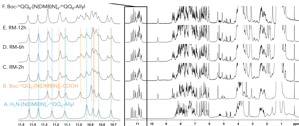
Figure 5.8 {}^1\text{H} NMR spectra in \text{CDCl}_3 of starting reagents (A) \text{H}_2\text{N-[N(DMB)N]}_2\text{-}{}^m\text{QQ}_8\text{-Allyl} 21 & (B) Boc- {}^m\text{QQ}_8\text{-[N(DMB)N]}_2\text{-COOH} 19 ; reaction mixture after (C) 2h, (D) 6h, (E) 12h and (F) purified coupling product Boc- {}^m\text{QQ}_8\text{-[N(DMB)N]}_4\text{-}{}^m\text{QQ}_8\text{-Allyl} 22 . The inset represents the zoom of the aromatic amide protons; the orange and blue dashed lines indicate the reactants.
