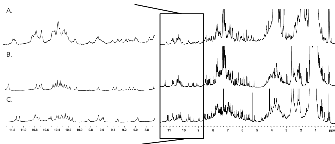
Figure 5.10 1 H NMR in CDCl 3 of (A) Tr-S-R-mQQ 8 -N 8 -mQQ 8 -PEG, (B) Tr-S-R-mQQ 8 -N 8 -mQQ 8 -COOH and (C) Tr-S-R-mQQ 8 -N 8 -mQQ 8 -Allyl. The downfield area of the NMR spectra is zoomed in the inset.
