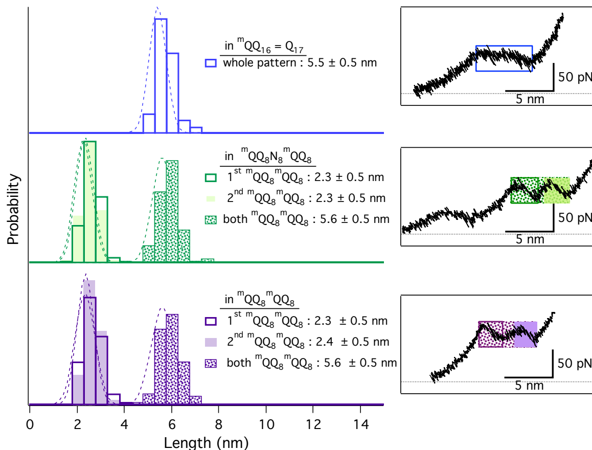
Figure 6.5 Histograms and Gaussian fits of the lengths of different parts of the specific unfolding pattern of the diblock ^m\text{QQ}_8\text{N}_8^m\text{QQ}_8 , the triblock ^m\text{QQ}_8^m\text{QQ}_8 and the monoblock \text{Q}_{17} (measurement from hybrid surface). The different parts are explicitly shown on the force-distance curves on the right.
