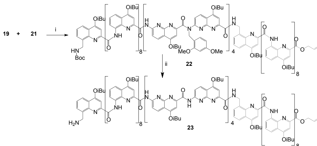
Scheme 6: Representation of the synthesis of {}^m\text{QQ}_8\text{-N}_8\text{-}{}^m\text{QQ}_8 amine 23 from \text{N(DMB)N}_2\text{-}{}^m\text{QQ}_8 amine 21 and \text{N(DMB)N}_2\text{-}{}^m\text{QQ}_8 acid 19 . The yield could not be calculated because of too small amounts.
