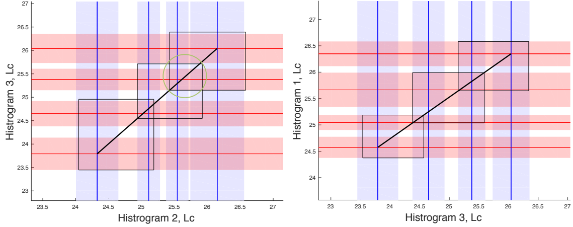
Figure S 5 Cross-superposition of 3 L_c evolution histograms (2x2) of 9-foldamers. Plain red and blue lines represent the mean L_c values of the Gaussian fits of the histograms. Transparent red and blue zones represent the band given by a standard deviation around the mean L_c of the position of the intermediate state. Both shown diagonal rectangles are always between 2 intermediate states.
