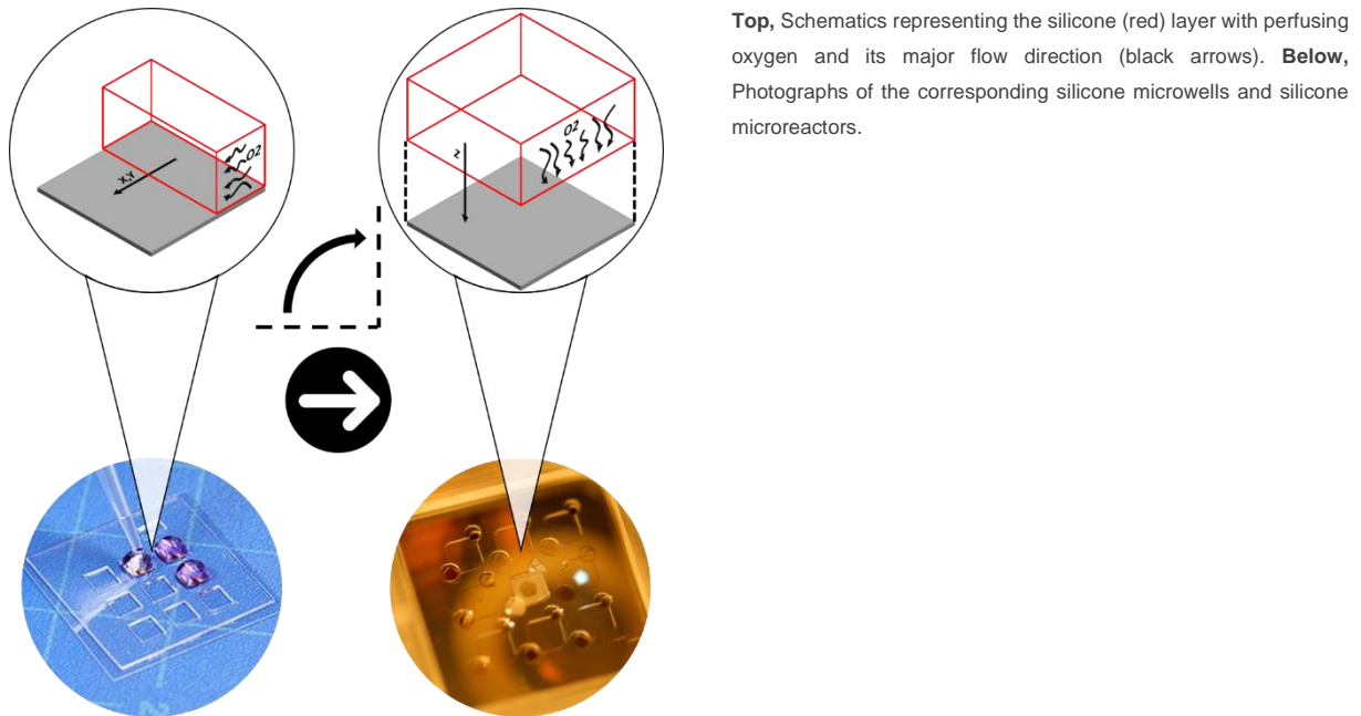
Figure 27 | From wells to microreactors.
