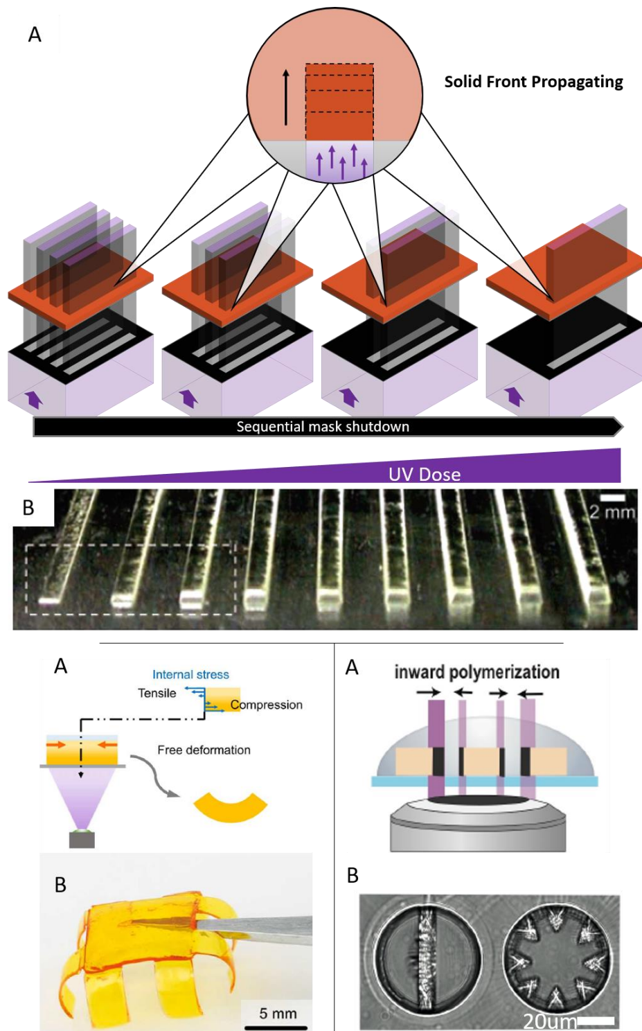
Figure 22 | Frontal photopolymerization.
