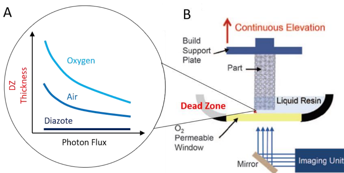
Figure 13 | Oxygen inhibited stereolithography.
