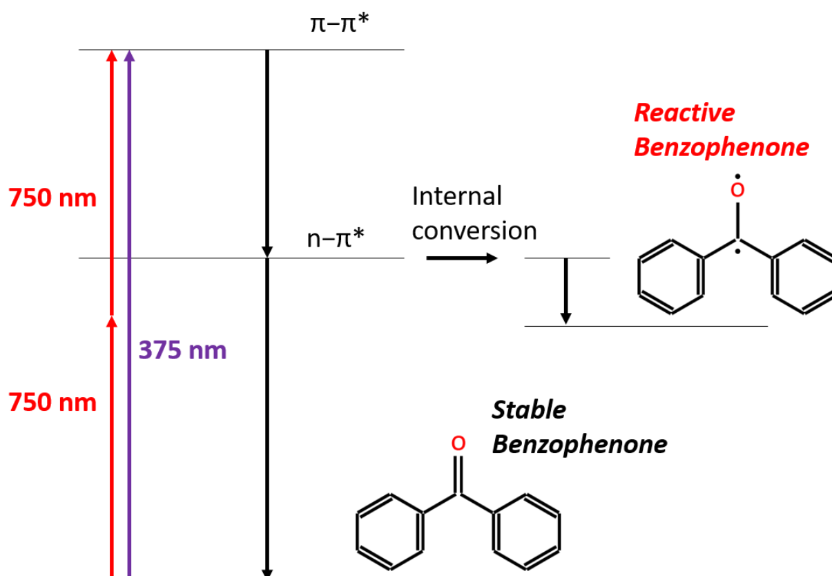
Figure 7 | Principles of light-matter interaction with the oversimplified example of benzophenone.
