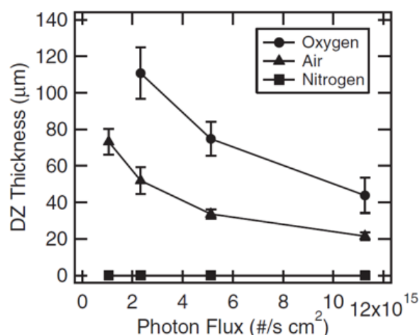
Figure 26 | Inhibition depends on oxygen concentration and photon flux.
