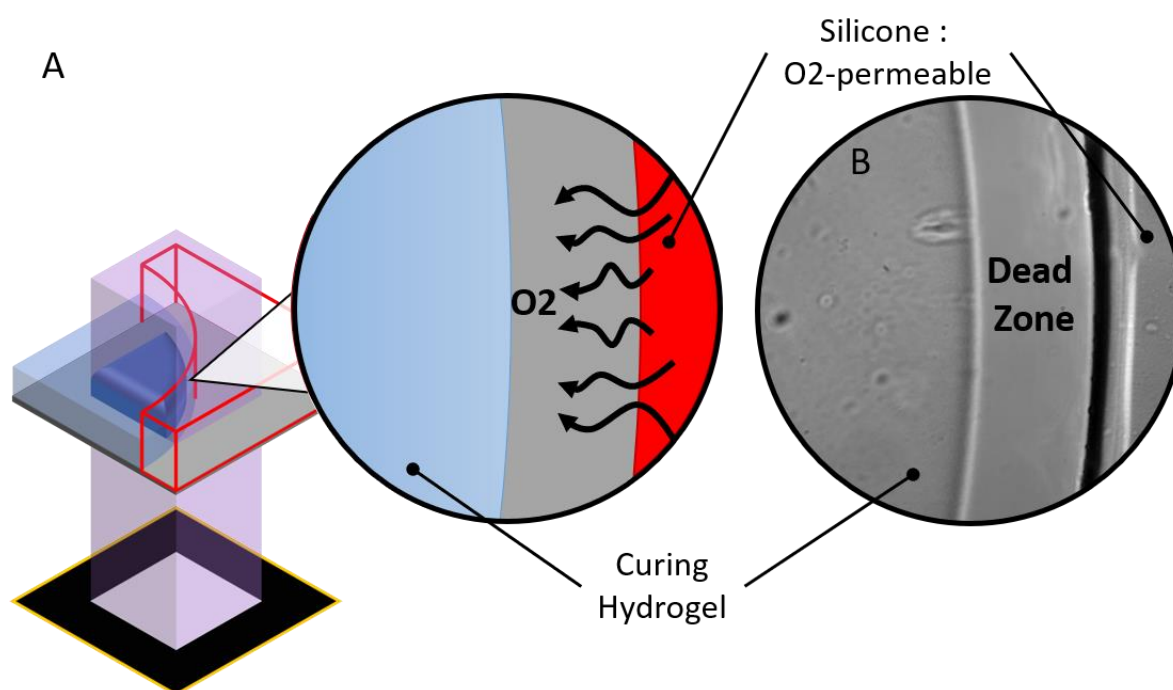
Figure 25 | Oxygen inhibition is easily observed near silicone.
