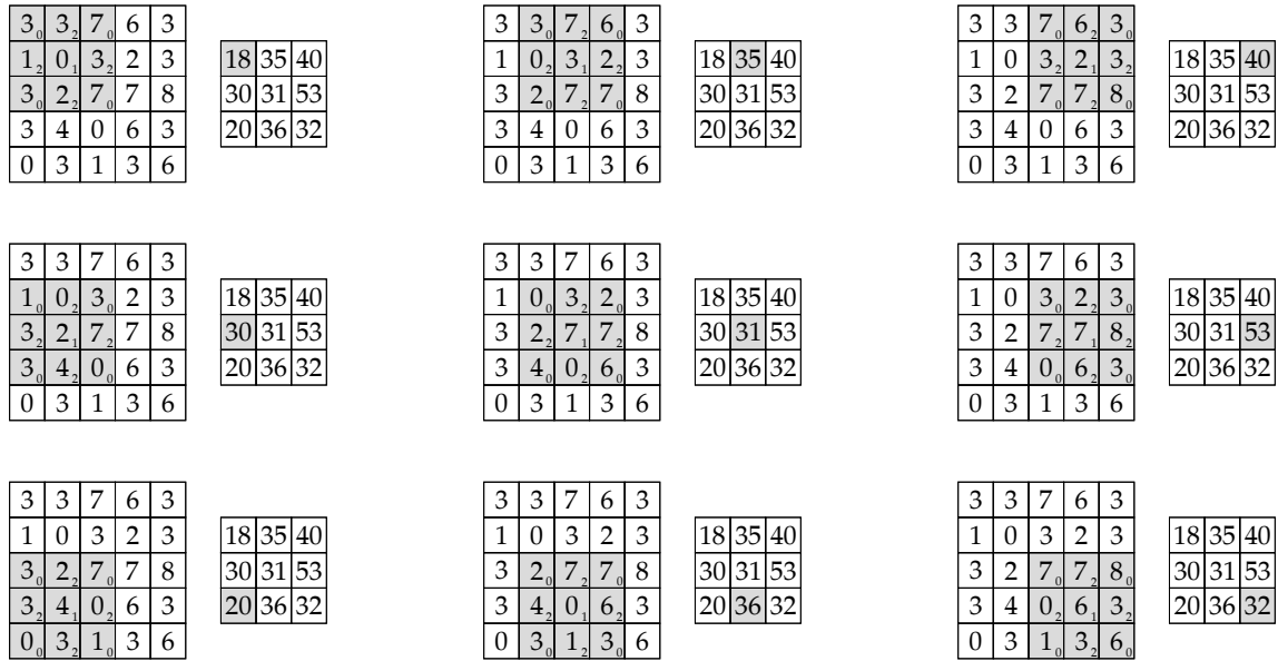
Figure 2.5: An example of the discrete convolution. The input feature map is a matrix of 5 \times 5 and a 3 \times 3 kernel. The shaded are superimposed on the input feature map denotes the neighborhood being processed and the shaded area over the output feature map denotes the output element at the current step.
