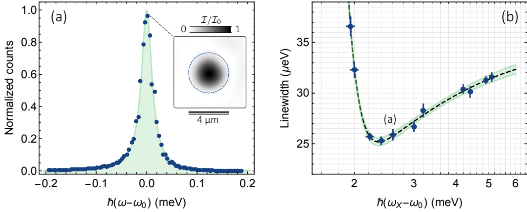
Figure 3.4: Scaling of the polariton linewidth: (a) Typical transmission spectrum of a circular micropillar with a 2.0 \mu\text{m} radius measured by resonant spectroscopy. Inset: emission profile at resonance ( \omega_0 ), here \hbar(\omega_x - \omega_0) = 2.60(5) \text{ meV} , the fit is a lorentian profile yielding the polariton linewidth \Gamma = 25.9(5) \mu\text{eV} . (b) Scaling of the measured polariton linewidth as a function of the detuning of the resonance with respect to the exciton transition (symbols). The dashed line is a fit with Eq. (3.1), the shaded areas correspond to the 95% confidence level of the fit.
