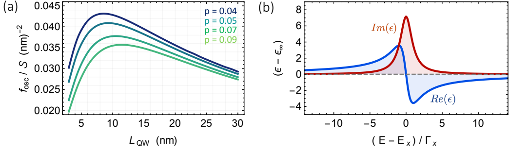
Figure 2.8: QW optical response (a) Oscillator strength per unit area of a shallow \text{In}_p\text{Ga}_{1-p}\text{As} QW as a function of the well thickness. (b) Excitonic contribution to the static dielectric function of a 15 nm QW with a 5% In fraction. Here, E_x and \Gamma_x are the exciton energy and homogeneous linewidth, respectively.
