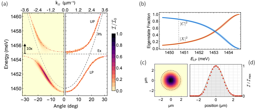
Figure 5.3: Eigenstate fraction and mode volume: (a) Energy and angle resolved photoluminescence of a square 120 \times 120 \mu\text{m} unetched portion of the sample (left) and corresponding fit with the polariton dispersion relation (right). (b) Eigenstate fraction as a function of the lower polariton energy, deduced from the fit of panel (a). (c) Measured emission pattern |u(\mathbf{r})|^2 of the lowest energy ( E_0 = 1450.61(1) meV) discrete mode of a 2 \mu\text{m} radius micropillar. (d) Cuts through the x and y axes of the measured mode profile (c) are compared with the predictions of a finite element model of the micropillar (cf. Sec. 2.4.1), allow extracting the modal area \mathcal{A} \approx 6.0 \mu\text{m}^2 .
