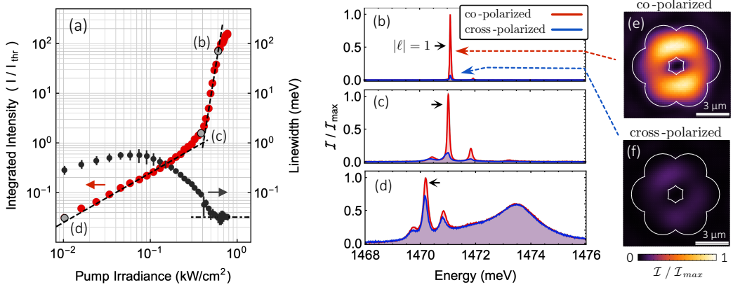
Figure 4.7: M1 microlaser. (a) Integrated output intensity and linewidth of the |\ell| = 1 emission measured as a function of incident pump power; the lasing threshold is at P_{\text{thr}} \sim 0.4 \text{ kW}/\text{cm}^2 . Dashed lines: I-P curve power law fits; Dot-dashed line: spectrometer resolution. (b-d) Polarization and energy resolved emission spectra under \sigma_+ polarized pump above (b), at (c) and below (d) the lasing threshold. Red and blue curves correspond to (\sigma_+) co- and (\sigma_-) cross-polarized emission with respect to the polarization of the pump. (e,f) Co- and cross-polarized real space images of the emission under a \sigma_+ polarized pump without any spectral filtering.
