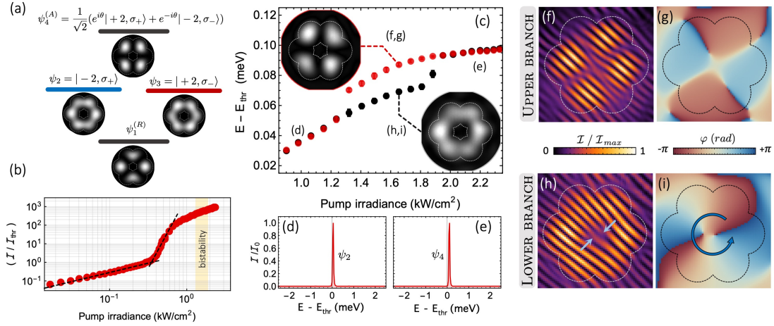
Figure 4.12: OAM bistability - data. (a) Illustration of the modes in the M2 lasing manifold ( |\ell| = 2 ) fine structure. The calculated the emission patterns for each mode is filtered in the H polarization basis. (b) Measured I-P curve, no hysteretic behaviour can be appreciated in the intensity. (c) Energy of the emission peak as a function of excitation power, when the power is ramped up (black dots) and down (red dots). The insets show real space images of the beam below and above the bistability. (d,e) Normalized emission spectra for P = (1.0, 2.2) kWcm -2 , respectively. (f,h) self-interferometry patterns and (g,i) corresponding phase maps measured in the (f,g) lower and (h,i) upper branches of the bistability, for the same pump power. All images are taken with a horizontal polarization filtering.
