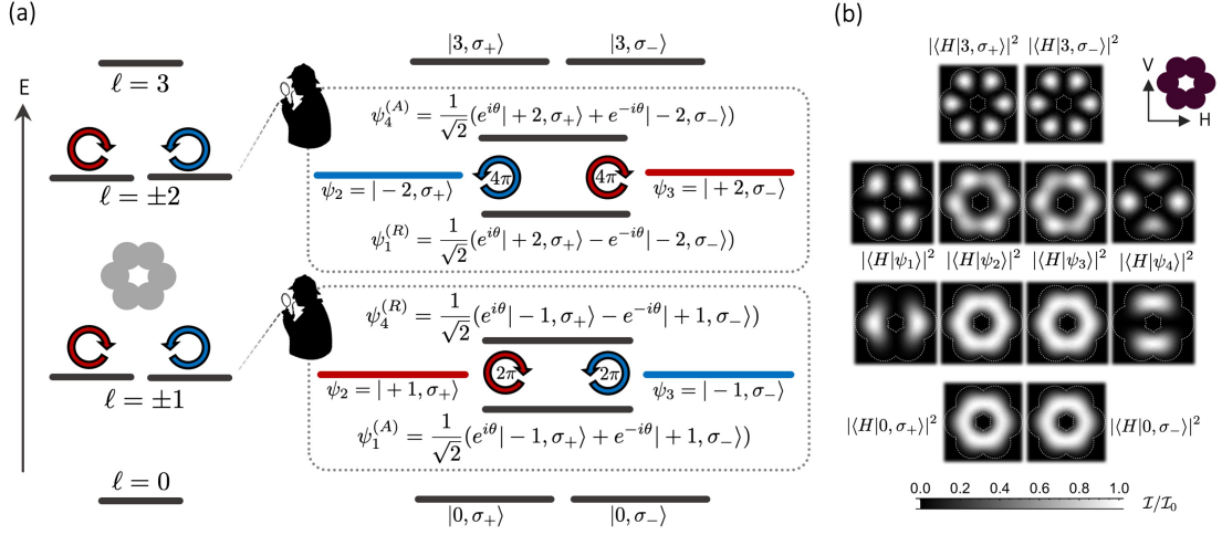
Figure 4.4: Fine structure modes: (a) Schematic illustration of the energy ladder for N = 6 both for the scalar model and when including a finite spin-orbit coupling \Delta t . Each level eigenmode is classified according to a SAM-OAM basis decomposition. (b) Normalized spatial intensity patterns obtained by finite element methods upon projecting the electric field along the x axis (H), see App. 2.6 for details. In the V polarization basis all the patterns remain unchanged, except for \psi_{1,4}(\ell) satisfying the relation |\langle H|\psi_{(1,4)}\rangle| = |\langle V|\psi_{(4,1)}\rangle| .
