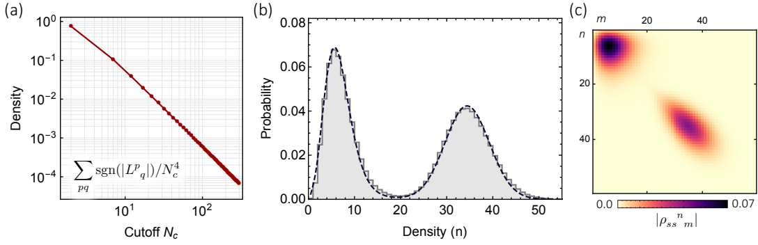
Figure 3.8: Diagonalization of the Liouvillian: (a) Density of the sparse matrix L representing the Liouvillian in the superspace |n\rangle \otimes |m\rangle basis as a function of the Fock basis cutoff N_c ( \dim(L) = N_c^4 ). (b) Comparison of the number density distribution obtained with the TWA (gray bars) and from the diagonal elements of the steady state density matrix \rho_{ss} , that is the \lambda = 0 eigenvector of L (dashed line). Parameters are the same as in Fig. 3.7. (c) Absolute value of the \rho_{ss}^n_m entries.
