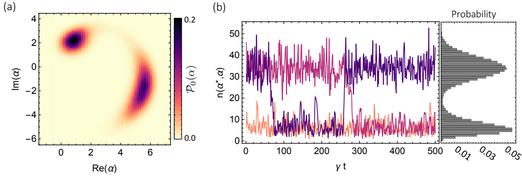
Figure 3.7: Truncated Wigner approximation: (a) Phase-portrait of \mathcal{P}_0(\alpha, \alpha^*) describing a single Kerr resonator for the same parameters of Fig. 3.6-(b). To reconstruct P_0 we simulated 10^3 trajectories using Eq. (3.13), each one elapsing 10^4\gamma^{-1} , with a 10^{-2}\gamma^{-1} discretization (Euler–Maruyama scheme). Recalling the Markovianity of the trajectories for \delta t\gamma \gg 1 , one can assume ergodicity and obtain 10^6 independent values of \alpha , then binned as function of their real and imaginary part. (b) Examples of the stochastic evolution of the number density operator in a phase-space representation ( n = \alpha^*\alpha - 1/2 ). The frequency histogram of n shows bimodality underpinning the existence of mean-field bistable fixed-points, which are actually metastable due to quantum-activated switching between the two attractors in phase-space (see the abrupt jumps in the trajectories) [225, 226, 227].
