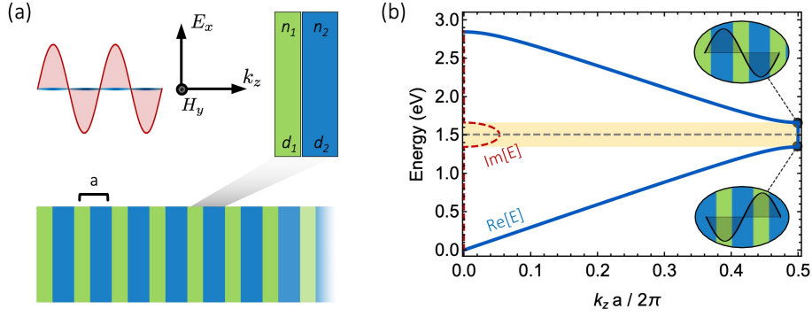
Figure 2.1: 1D Photonic Crystals (a) A transverse electromagnetic (TEM) wave propagates in a material with a periodic dielectric constant along the z axis. The structure period is a and is composed by alternating layers of thickness d_{1,2} and refractive index n_{1,2} . (b) Photonic band structure for quarter wave stacks ( d_1 n_1 = d_2 n_2 = \lambda_0/4 ) with n_1 = 1.0 , n_2 = 1.5 , and hc/\lambda_0 = 1.5 eV. The insets show the electric field profile at the two band edges.
