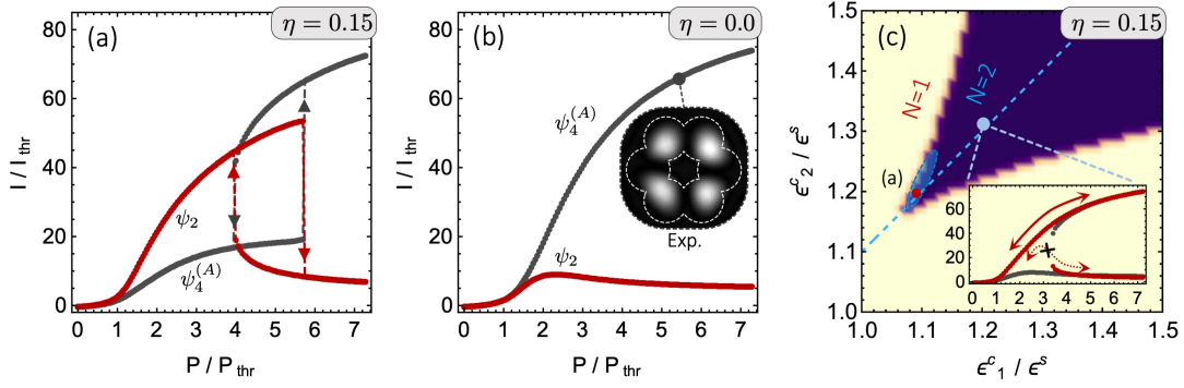
Figure 4.13: OAM bistability - model. (a) Calculated intensity of the photonic modes \psi_2 and \psi_4 under a (a) circularly and (b) linearly polarized excitation. Under a circular excitation, a bistability region can be observed, the arrows indicating the scanning history. Simulation parameters: g_0 = 0.55 \mu\text{s}^{-1} , \epsilon_{1,2}^s = \epsilon^s = 5.0 \cdot 10^{-5} , \epsilon_1^c/\epsilon^s = 1.09 , \epsilon_1^c/\epsilon^s = 1.20 , \beta\Gamma_r = 1.05 \text{ ps}^{-1} , \Gamma_c = 4\Gamma_r = 25 \text{ ps}^{-1} . (c) Number of stable steady-state solutions for P = 5P_{\text{thr}} in the cross saturation parameter space; panel (a) corresponds to the red dot. The elliptic shaded area encompasses the region where modal hysteresis can be observed for an adiabatic power ramp. Outside of it, two solutions exist but one of them can be followed continuously explored for any pump power. The other one can thus be reached only with an appropriate non-adiabatic pump protocol [218], see the inset for an example.
