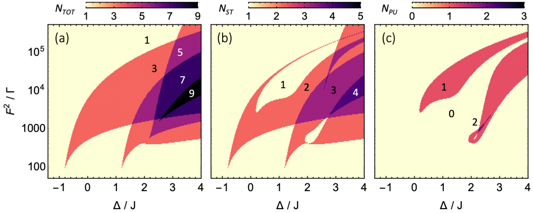
Figure 5.1: Phase diagram of the CKRs: (a) Total number of steady state solutions as a function of the drive detuning \Delta and power F^2/\Gamma . (b) Number of stable solutions; bistability occurs for \Delta > -J + \sqrt{3}/2\Gamma , multistability for \Delta/J > 1.56 . (c) Number of parametrically unstable solutions, N \geq 1 if \Delta > \Gamma . Single mode unstable solutions can be deduced subtracting panel (b,c) to panel (a). Other parameters: U/\Gamma = 0.01 and J/\gamma = 5 .
