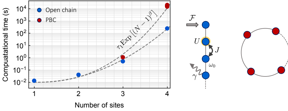
Figure 3.5: Searching for the MF steady state - a heavy toll: Scaling of the single-core computational time spent to find a complete set of steady-state solutions for Eq. (3.4) as a function of the number N of resonators in the lattice. Nearest-neighbor hopping only is considered both in the case of an open chain (blue markers) and imposing periodic boundary conditions (red markers). If \tau_1 is the single resonator time, the scaling with N has the empirical form shown in the inset. The exponent \beta is 2.1(1) and 2.4(1) for the open and periodic boundaries, respectively. For each value of N we simulated 5 different values of \mathcal{F}_1 \sim \sqrt{\Delta/\gamma U} , that is deep in the multistable portion of parameter space. We consider identical resonators with (\Delta, J) = 3\gamma and U/\gamma = 10^{-2} . For the computation we used a customized homotopy method implemented using the libraries of Mathematica running on 3.2 GHz processor.
