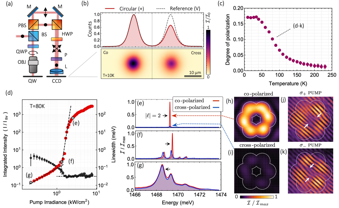
Figure 4.11: Probing the temperature robustness of the scheme. (a) Schematic of the degree of polarization measurement apparatus (details in the main text). (b) Example of the detected signal under a circular ( \sigma_+ ) excitation at 10K; left and right sides of the panel correspond to the co- and cross-circularly polarized components of the QW emission, respectively. Top: normalized vertical binning of the image, the dashed line shows the corresponding profile acquired under a linear excitation (V). (c) Measured degree of circular polarizations as a function of temperature; error bars correspond to two standard deviations. (d-k) Characterization of the M2 device at 80K. (d) Intensity and linewidth dependence with pump power under a \sigma_+ excitation. (e-g) Polarization resolved emission above, at and below the lasing threshold ( P_{\text{thr}} \approx 1.1 \text{ kWcm}^{-2} ), respectively. (h-i) Co- and cross-circularly polarized emission pattern in the lasing regime corresponding to (e). (j,i) Interferograms under a \sigma_+ and \sigma_- polarized excitation, respectively. The inversion in the pitchfork dislocations between panel (j) and (k) signals that the 4\pi vortex helicity is switched.
