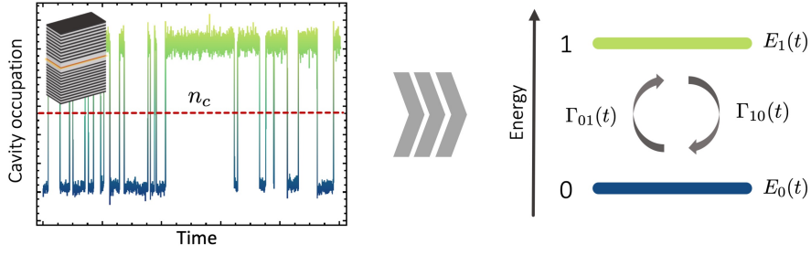
Figure 6.7: Mapping proposal: A threshold value of the cavity occupation ( n_c ) is used to digitize the photodiode signal as a function of time. The dark (bright) metastable states are identified with the \sigma = 0 ( \sigma = 1 ) states of the bit with energy E_0 ( E_1 ). The contact with a bath results in random bit flip events 0 \rightarrow 1 ( 1 \rightarrow 0 ) with a rate \Gamma_{01} ( \Gamma_{10} ).
