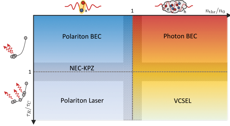
Figure 2.12: Microcavity stimulated emission phenomenology under non resonant pumping. Two order parameters rule the diagram: (1) the ratio between the bosonic stimulation threshold n_{thr} and exciton dissociation density n_0 and (2) the ratio between the relaxation time of excitations \tau_R and their lifetime \tau_C . Gray areas around n_{thr}/n_0 \sim 1 and \tau_R/\tau_C \sim 1 display a non-universal, hybrid phenomenology.
