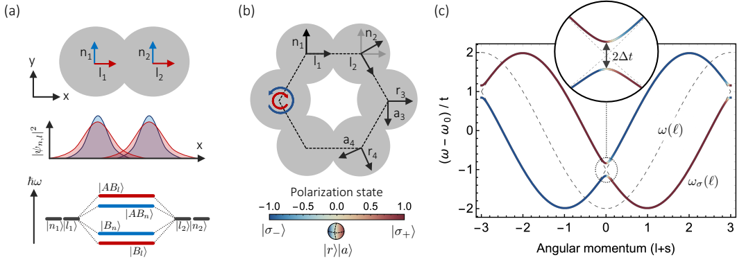
Figure 4.3: Analog spin-orbit coupling: (a) The modes linearly polarized along x ( \vec{l}_{1,2} basis) have a larger coupling than the ones polarized along y ( \vec{n}_{1,2} basis). In a tight-binding picture this corresponds to a larger overlap integral t_l \sim \langle l_1 | l_2 \rangle > t_n , where |\psi^i\rangle are the bare pillar modes. This results in a splitting of the bonding (B) and anti-bonding (AB) modes in the level hybridization diagram. In benzene photonic molecules, as the link direction \vec{l}_i changes from pillar to pillar this creates an azimuthally varying birefringent axis for the linearly polarized photons (c), corresponding to an analog spin (polarization) orbit coupling [187]. (d) The eigenmodes of a ring arrangement of microcavities can be classified based on the total angular momentum J = \ell + \sigma , and follow the dispersion relation \omega_\sigma(\ell) (here N = 6 , details in the main text). When introducing a finite polarization splitting \Delta t = (t_l - t_n) > 0 , the modes written in a circular polarization basis \sigma = \pm 1 (SAM) hybridize at j = 0, 3 , lifting the degeneracy of the |\ell| = 1, 2 multiplets.
