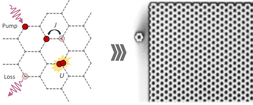
Figure 2.16: A photonic platform for analog simulation: (Left) schematic representation of a honeycomb lattice for interacting bosons subject to pump and losses. (Right) SEM image of the corresponding analog implementation with coupled microcavities, image adapted from [190].
