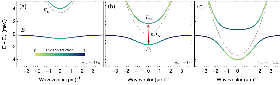
Figure 2.10: Polariton dispersion relation (a,b,c) The upper and lower polariton branches E_{u,l} are plotted against in-plane wavevector for three representative values of exciton-cavity detuning: \delta_{cx} = \Omega_R (a), \delta_{cx} = 0 (b) and \delta_{cx} = -\Omega_R (c). The exciton fraction dependence on momentum is color-coded in each branch. Dashed lines correspond to the bare cavity ( E_c ) and exciton ( E_x ) dispersion relations, in all the plots \hbar\Omega_R = 3.36 meV.
