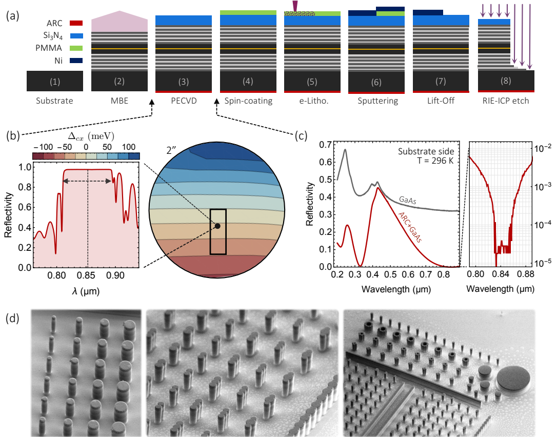
Figure 3.1: Sample fabrication: (a) Flow diagram of the sample fabrication (details in the main text). (b) Reflectivity spectra obtained by Fourier-transform infrared spectroscopy (FTIR) are used to map the cavity resonance across the two inch diameter planar heterostructure. Provided the energy of the exciton transition is known, this allows to derive an exciton-photon detuning map \Delta_{cx} . Accordingly, a small piece of the wafer is selected for steps (3-8) of the fabrication (Black rectangle). (c) Reflectivity spectrum of the GaAs substrate before and after the anti reflective coating (ARC) deposition in step (3). The central wavelength of the ARC can be tuned with the layer thickness. (d) Representative SEM images of the microstructures fabricated with the process (1-8).
