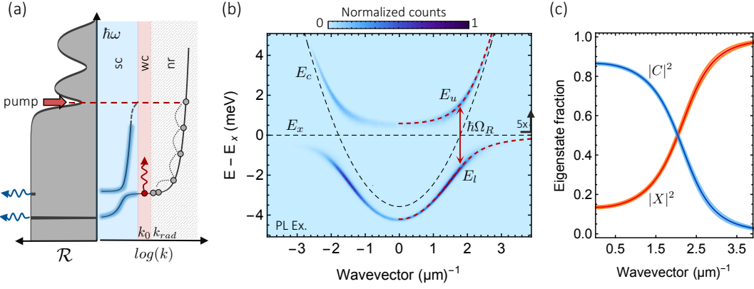
Figure 2.11: Photoluminescence experiment (a) Schematic representation of the off-resonant excitation scheme. The shaded gray profile is the microcavity reflectivity \mathcal{R} profile plotted against energy. The right part of the panel presents the polariton dispersion, wavevectors are log-scaled. (b) Measured angle-resolved photoluminescence. Dashed red lines represent a joint best fit of the polariton dispersion relations to the data E_{u,l} , dashed gray lines trace the corresponding bare cavity ( E_c ) and exciton ( E_x ) ones. For E > E_x intensities are multiplied by a factor five. (c) Light-matter contents as a function of in-plane momentum for the lower polariton branch. Shaded areas correspond to the 95% confidence intervals.
