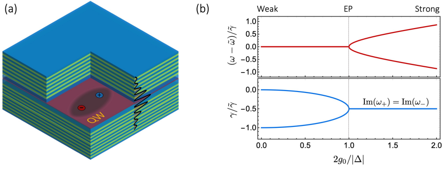
Figure 2.9: Light-matter coupling in semiconductor microcavities (a) Schematic representation of a semiconductor microcavity embedding a QW at the antinode of the optical field. (b) Real and imaginary part of the eigenvalues of the coupled oscillator model as a function of the coupling strength g_0 . The oscillator parameters are \omega_1/\omega_2 = 1 , \gamma_1/\omega_1 = 10^{-3} and \gamma_2 = 0 . Here \tilde{\omega} is the average complex frequency of the bare resonator modes and \tilde{\Delta} is their complex detuning.
