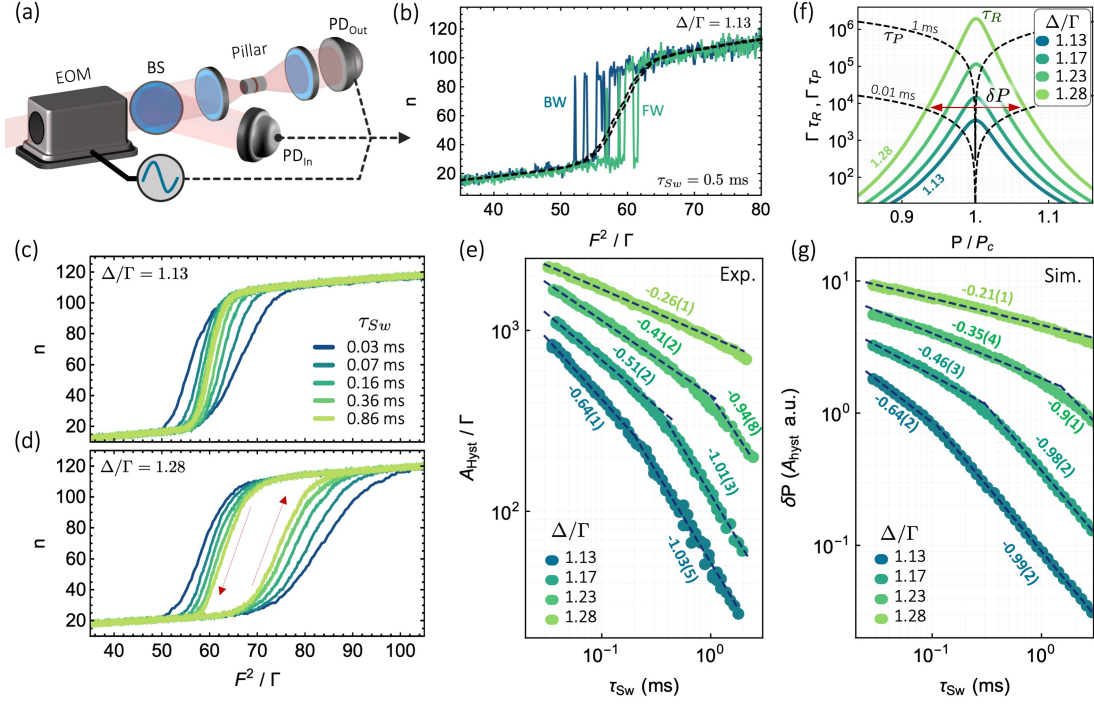
Figure 6.5: Dynamical Hysteresis: (a) Sketch of the experimental setup. (b) Example of single-shot (solid lines) and averaged (dashed line) trajectories of the cavity occupation ( n ) as a function of the input power ( F^2/\Gamma ). Here, the power is modulated with the EOM following a triangle-wave with period \tau_{Sw} = 0.5 ms. FW (BW) refers to the trajectory associated to an increasing (decreasing) side of the power ramp. (c,d) Hysteresis cycles obtained averaging over 10^3 trajectories as a function of the modulation period \tau_{Sw} for two detuning values (see the inset). (e) Measured average hysteresis area as a function of the modulation period. Different colors correspond to different detuning values (see the inset). Dashed lines are power law fits whose exponents are reported along with 2\sigma confidence intervals. (f) Calculation of the relaxation ( \tau_R , solid lines) and modulation ( \tau_P , dashed lines) timescales: the intersection of \tau_R with \tau_P determines the non-adiabatic power region \delta P proportional to the hysteresis area (see main text). (g) Scaling of the calculated \delta P with \tau_{Sw} for the same parameters of the experiments. Dashed lines are power-law fits.
