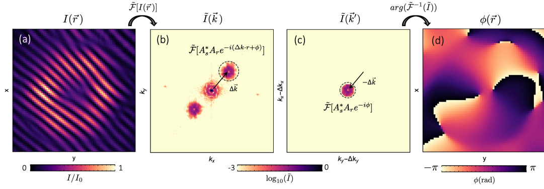
Figure 4.14: Retrieving the wavefront phase: (a)-Typical interference pattern for the |-2, \sigma_+\rangle mode, produced by interfering the emission and reference arm with an in-plane wavevector difference \Delta \mathbf{k} . (b) Log-scale absolute value of the CCD image fast Fourier transform (FFT). (c) After a rigid translation of the FFT by -\Delta \mathbf{k} we apply a radial low-pass filter. (d) Real space image of the emission phase \phi(r) , obtained as the argument of the inverse FFT.
