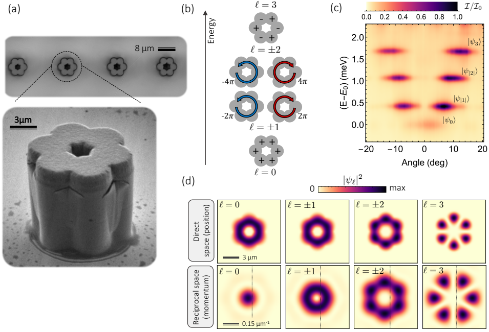
Figure 4.2: Benzene photonic molecules: (a) Top view optical microscopy and detail of the side view (SEM) of a coupled array formed by six overlapping micropillars with R = 1.6 \mu\text{m} radius and variable inter-pillar distance. (b) Schematic representation of the scalar eigenmodes |\psi_\ell\rangle of the structure; the phase relation between pillars is indicated. (c) Energy and angle-resolved photoluminescence of the microstructure below the lasing threshold, presenting the four OAM manifolds \ell = (0, \pm 1, \pm 2, 3) , E_0 \approx 1470 \text{ meV} . For comparison, panel (d) shows finite elements calculation of the |\psi_\ell\rangle profile both in direct (position) and reciprocal (momentum) space (cf. App. 2.6). The dashed line corresponds to the position of the slit used for panel (c).
