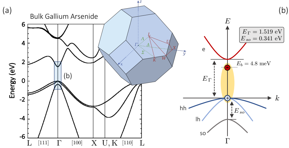
Figure 2.5: GaAs electronic properties (a) Bandstructure of bulk GaAs computed with a 30-band \mathbf{k} \cdot \mathbf{p} method, adapted from [87]. Inset: first Brillouin zone of a zincblende crystal. (b) Schematic representation of the conduction (e), heavy-hole (hh), light-hole (lh) and split-off (so) bands within a parabolic band approximation.
