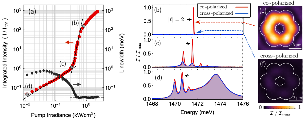
Figure 4.8: M2 microlaser. (a) Integrated output intensity and linewidth of the |\ell| = 2 emission measured as a function of incident pump power; the lasing threshold is at P_{\text{thr}} \sim 0.3 \text{ kW}/\text{cm}^2 . Dashed lines: I-P curve power law fits; Dot-dashed line: spectrometer resolution. (b-d) Polarization and energy resolved emission spectra under \sigma_+ polarized pump above (b), at (c) and below (d) the lasing threshold. Red and blue curves correspond to (\sigma_+) co- and (\sigma_-) cross-polarized emission with respect to the polarization of the pump. (e,f) Co- and cross-polarized real space images of the emission under a \sigma_+ polarized pump without any spectral filtering.
