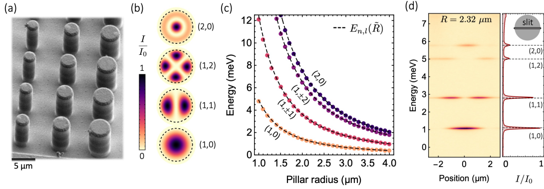
Figure 2.14: Micropillars: (a) SEM image of circular microcavities obtained by deep-etching a planar heterostructure. (b) Calculated intensity profile of the micropillar eigenmodes labeled by their principal and angular quantum numbers (n, l) . The dashed line represents the microstructure edge. (c) Finite element calculation of the energy of the lowest six eigenmodes as a function of the pillar radius (see App. 2.6 for details). Dashed lines are the predictions of Eq. (2.46) including the evanescent tails of the optical field ( \delta R \approx 0.05 \mu\text{m} ). (d) Spatially resolved PL spectrum measured on a pillar with nominal radius of R = 2.32 \mu\text{m} . Inset: position of the spectrometer slit; Dashed line: predictions of Eq. (2.46).
