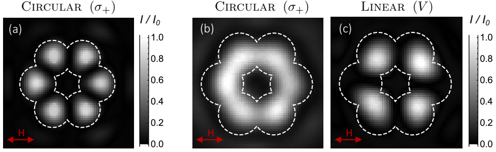
Figure 4.6: First hints: Imaging of the microlaser emission above the lasing threshold for a d = 2.6 \mu\text{m} (a) and d = 2.4 \mu\text{m} (b,c) microstructure. The pump polarization is circularly ( \sigma_+ ) polarized in (a,b) and vertically polarized in (c); all the three emission patterns were analyzed with a polarizer in the H basis (see arrow). These patterns can be directly compared with the calculations presented in Fig. 4.4-(b).
