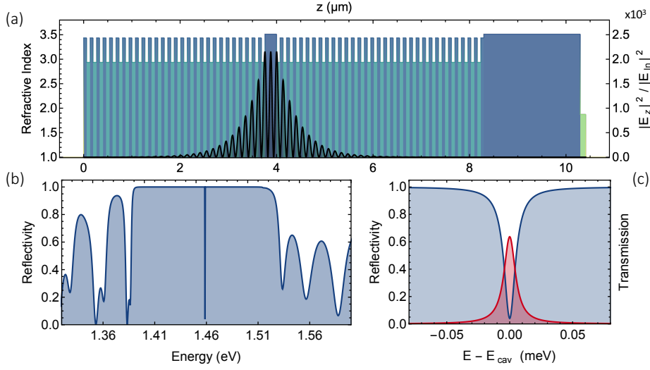
Figure 2.3: Fabry-Perot microcavity. (a) Refractive index profile for a \lambda Fabry-Perot cavity enclosed within two \text{Al}_{0.1}\text{Ga}_{0.9}\text{As}/\text{Al}_{0.95}\text{Ga}_{0.05}\text{As} DBRs with 28 (top) and 32 (bottom) pairs. The spacer and substrate are crystalline GaAs, the right-most greenish layer is a Silicon Oxynitride \lambda/4 anti-reflective coating. The cavity mode profile at resonance is traced in black. (b) Reflectivity spectrum of the cavity showing a pronounced dip at E_0 = 1.459 eV. (c) Reflectivity and transmission spectrum of the cavity mode.
