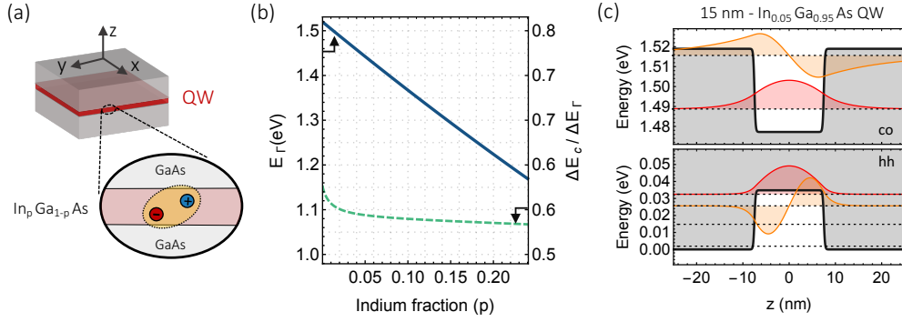
Figure 2.6: InGaAs Quantum Wells. (a) Graphic representation of a quantum well for electron and holes, formed by a few nanometer thick layer of a material embedded in a host semiconductor matrix characterized by a larger bandgap. (b) Dependence on the molar Indium fraction ( p ) of the bandgap ( E_\Gamma , solid line, from [89, 93]) and of the conduction band mismatch ( \Delta E_c , dashed line, from [94, 95, 96]) for a GaAs/InGaAs heterointerface. (c) Calculated energies (dotted lines) and envelope functions \chi_{e,h}(z) of electrons and heavy-holes (solid lines) along the growth axis z of a p = 0.05 heterostructure. Correspondingly, solid gray lines trace the conduction and valence band profile.
