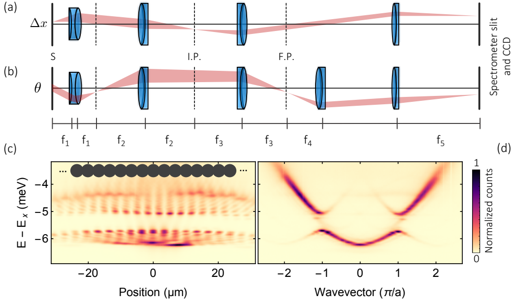
Figure 3.3: Imaging techniques: (a) Real space imaging: a point source in the sample plane (S) at a distance \Delta x from the optical axis is mapped to a point at a distance \Delta x' \approx (f_2 f_5)/(f_1 f_3) \Delta x in the spectrometer entrance slit. (b) Momentum space imaging: the sample emission at an angle \theta with respect to the optical axis is mapped to a point at a distance \Delta x' \approx (f_3 f_5 / f_2 f_4) f_1 \tan \theta in the spectrometer entrance slit. The intermediate image plane (I.P.) and Fourier plane (F.P.) can be used for filtering purposes. (c,d) Examples of position (c) and momentum (d) resolved emission spectra of a 1D lattice formed by circular micropillars with radius R = 2.0 \mu\text{m} and center-to-center distance a = 3.4 \mu\text{m} ; E_x \approx 1453.5 \text{ meV} is the exciton energy.
