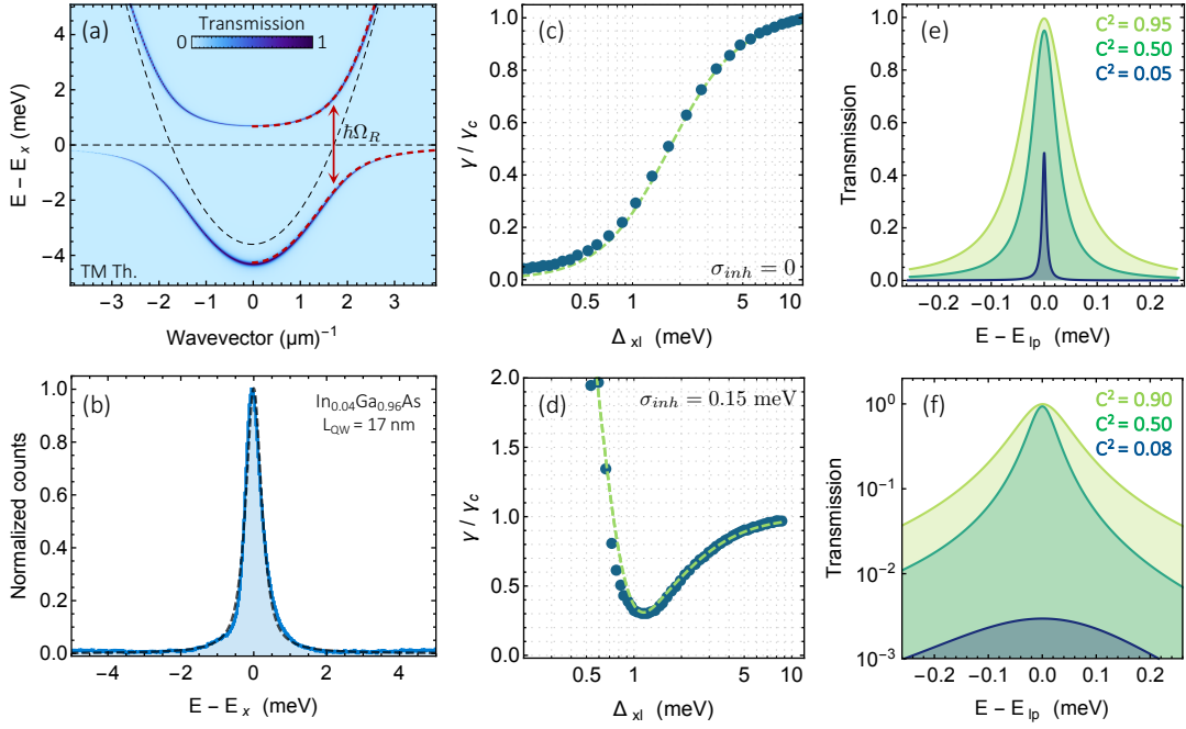
Figure 2.13: Scaling of the polariton linewidth (a) Transfer-matrix simulation of the microcavity transmission as a function of the incident in-plane wavevector and energy. Dashed line: nominal polariton dispersion relation [Eq. (2.31)]. (b) Typical PL spectrum of a shallow InGaAs QW, the dashed line is pseudo-Voigt profile fit. (c,d) Scaling of the polariton linewidth as a function of the exciton-lower polariton detuning \Delta_{xl} = (E_x - E_l) for a radiatively limited exciton transition (c), or including a gaussian inhomogeneous broadening (d). (e,f) Representative examples of transmission spectra corresponding to panels (c,d), respectively.
