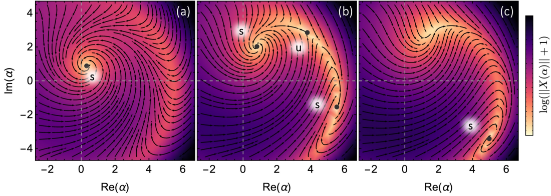
Figure 3.6: Phase-space portrait for one Kerr resonator: Streamlines showing the local direction of the vector field X = \dot{\alpha} describing the MF dynamics a single Kerr resonator [Eq. (3.3)] for \mathcal{F}^2/\gamma = (4, 18, 27) in panels (a,b,c) respectively. Other parameters are \Delta/\gamma = 1.5 , U/\gamma = 0.05 . Fixed-points ( X = 0 ) are indicated by circular markers: both stable (s) and unstable (u) ones can be observed, as clearly indicated by the absence (presence) of outward pointing streamlines. The colormap encodes the scaled log-norm of the vector field indicating the local magnitude of the \dot{\alpha} . Panel (b) evidences the optical bistability phenomenon [214, 216].
