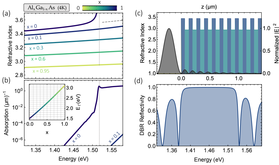
Figure 2.2: Distributed Bragg reflectors. (a) Refractive index at 4K as a function of the photon energy and Aluminum concentration x for \text{Al}_x\text{Ga}_{1-x}\text{As} alloys. (b) Corresponding absorption coefficients, the inset shows the \Gamma point energy gap as a function of Aluminum concentration. (c) Refractive index and mode profile for monochromatic light (1.46 eV) at normal incidence on a DBR with 20.5 \text{Al}_{0.1}\text{Ga}_{0.9}\text{As}/\text{Al}_{0.95}\text{Ga}_{0.05}\text{As} pairs. (d) Reflectivity profile of the DBR.
