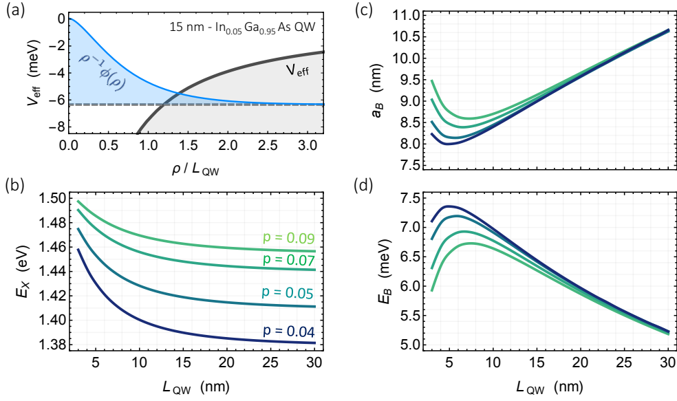
Figure 2.7: Shallow InGaAs QW properties. (a) The pseudo potential defined by Eq. (2.17) -in gray- is plotted together with the associated lowest energy radial eigenfunction \phi(\rho) (light-blue profile). Inset: QW parameters. (b,c,d) Show the calculated fundamental hh-exciton energy (b), Bohr radius (c) and binding energy (d) as a function of the QW thickness for four representative values of the In fraction, ranging from 0.04 to 0.09 and color-coded from blue to green. All the results correspond to the ten self-consistent iteration of the pseudo-potential algorithm.
