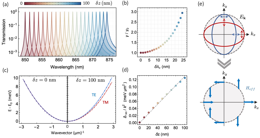
Figure 2.4: Polarization effects in microcavities. (a) Transmission spectra for a Fabry-Perot cavity formed by two x = (0.10, 0.95) DBRs with 20 (24) pairs on the top (bottom) mirror. The cavity spacer optical thickness is increased by an amount \delta z . (b) Scaling of the resonance redshift and cavity linewidth as a function of \delta z . (c) Calculated cavity dispersion relations at \delta z = 0 nm (left panel) and \delta z = 100 nm (right panel) for both linear polarizations (TE-TM). (d) Scaling of the polarization-dependent energy splitting \Delta_{so}/k^2 with \delta z . (e) Schematic representation of an isoenergetic cut in momentum space through the dispersion relation for the TE and TM components (relative to the xz plane) of incident light. Corresponding effective magnetic field ( H_{\text{eff}} ) pattern along the elastic circle E_{\mathbf{k}} = \text{const} . [74].
