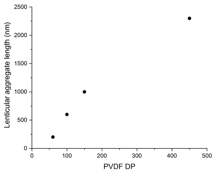
Figure S6. Plot of PVDF degree of polymerization vs. length of lenticular aggregates.
