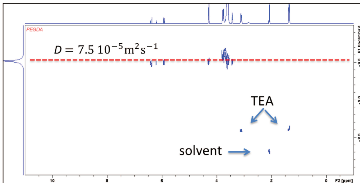
Figure S8. ^1\text{H} DOSY-NMR experiments recorded in (\text{CD}_3)_2\text{SO} at 60 °C of PEGDA homopolymer.
