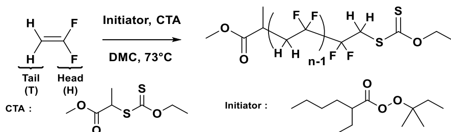
Figure 11. Schematic representation of the RAFT Polymerization of VDF in DMC. 40
