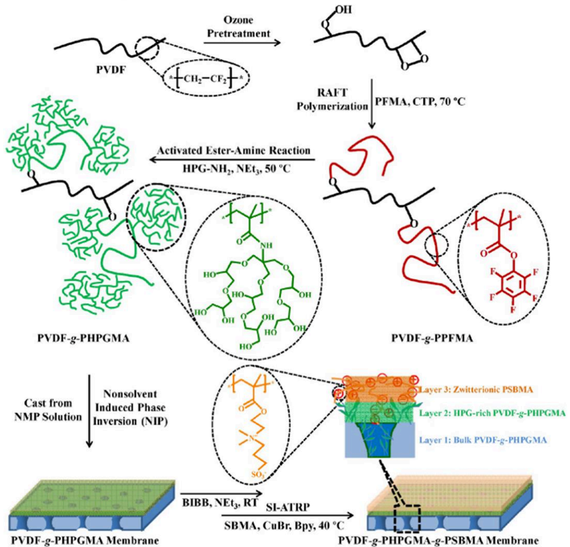
Figure 7. Schematic illustration of the processes of ozone pretreatment and RAFT graft copolymerization of PVDF with PFMA, Activated ester-amine reaction, preparation of PVDF-g-PHPGMA-g-PSBMA membrane via SI-ATRP of SBMA from the PVDF-g-PHPGMA Membrane. PPFMA (pentafluorophenyl methacrylate), CTP (4-cyano-4-(phenylcarbonothioylthio)pentanoic acid), HPG-NH 2 (amino-terminated hyperbranched polyglycerol), NE 3 (trimethylamine), NMP (1-methyl-2-pyrrolidone), NIP (Non-solvent induced phase separation, also referred as NIPS), BIBB (2-bromo-2-methylpropionyl bromide), SBMA (N-(3-sulfopropyl)-N-(methacryloxyethyl)-N,N-dimethylammonium betaine), CuBr (Copper bromide), Bpy (2,2'-bipyridine) 92
