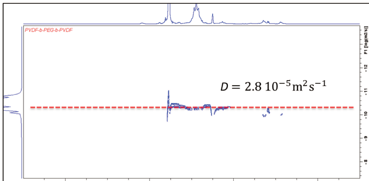
Figure S9. ^1\text{H} DOSY-NMR experiments recorded in (\text{CD}_3)_2\text{SO} at 60 °C of PVDF- b -PEG- b -PVDF triblock copolymer.
