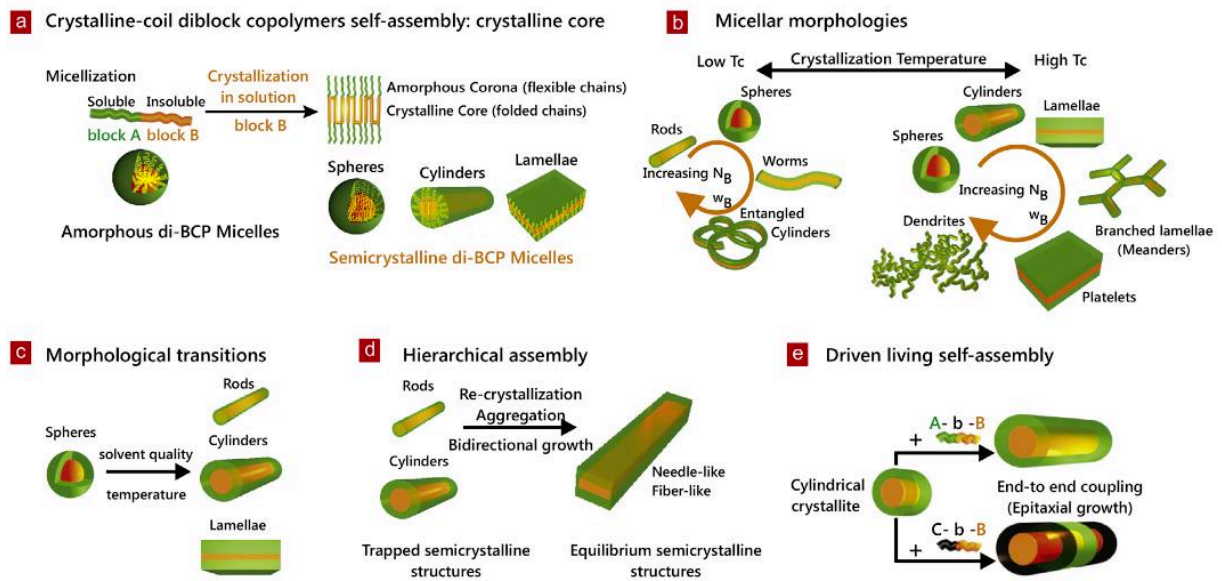
Figure 19. Different self-assembly protocols to prepare micelles from coil-crystallineBCPs: a) Schematic representation of the preparation of semicrystalline BCP micelles from amorphous micelles in solution where the core-forming block undergoes crystallization leading to a folded-chain structure. Typical structures of coil-crystalline BCPs micelles are spheres, cylinders and lamellae. b) Morphologies formed from PB- b -PEO in n -heptane by varying degree of polymerization and crystallization temperature. c) By changing the solubility of the corona-forming block in the solvent (with addition of another solvent, or changing the temperature), the resulting micellar morphology can be further tuned. d) Kinetically trapped semi-crystalline micelles can lead to the formation of equilibrium structures through re-crystallization and/or aggregation of intermediate structures. e) Epitaxial crystallization process by adding crystallizable BCP-unimers (same or different BCP) can lead to a living extension of the micellar structure. 175
