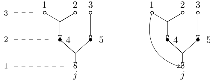
Figure 4.3: A ranked implicative base (left) and an acyclic implicative base that does not admit a rank function (right). Ranks are depicted by dashed lines.
