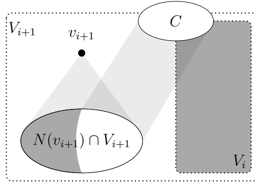
Figure 2.5: The situation of Lemma 2.2.7. The set N[D^*] \cap V_{i+1} is depicted in gray (except v_{i+1} , in the first case of the proof), and the set S = V_{i+1} \setminus (N[D^*] \cup \{v_{i+1}\}) \subseteq N(v_{i+1}) \cap V_{i+1} is in white. Note that C = N(S) \setminus \{v_{i+1}\} may intersect V(G) \setminus V_{i+1} .
