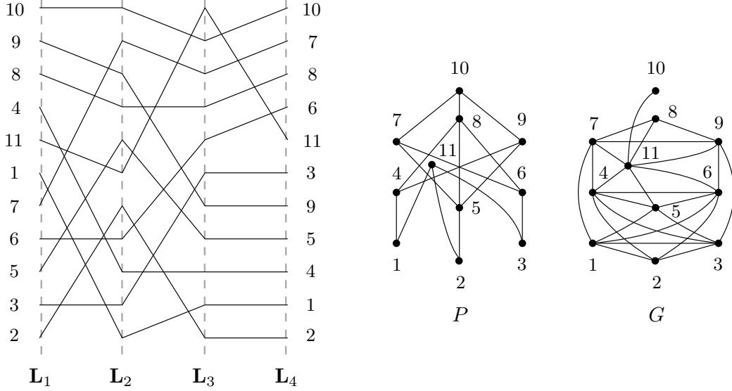
Figure 2.9: A poset P and its incomparability graph G as an intersection graph of curves induced by four linear extensions witnessing the dimension.
