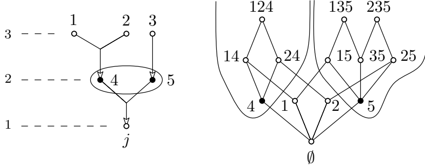
Figure 4.4: The situation of Theorem 4.4.3. On the left a ranked implicational base (X, \Sigma) and its rank function (dashed). On the right the set of closed sets of \Sigma not containing j , ordered by inclusion. Maximal independent sets of \mathcal{E}(\mathcal{H}_j) = \{\{4, 5\}\} are \{4\} and \{5\} . They partition j^{\nearrow} = j^{\nearrow} = \{\{1, 2, 4\}\} \uplus \{\{1, 3, 5\}, \{2, 3, 5\}\} .
