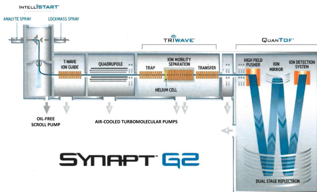
Figure II.17 : Schéma du Synapt G2 HDMS.
