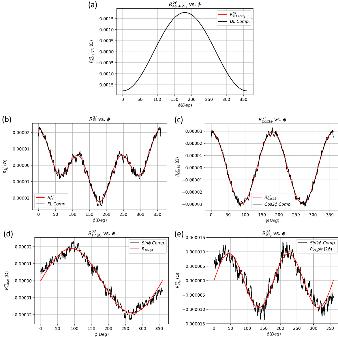
Figure 3.19: Components of the second harmonic Hall resistance considering all the angular symmetries. (a) DL and thermal (b) FL (c) \cos2\phi (d) \sin\phi (e) \sin2\phi components. The black lines are the signals extracted from the measured second harmonic resistance and the red lines are the fits.
