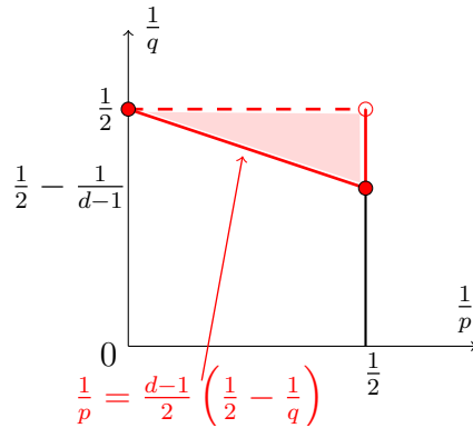
FIGURE 3.3 – Admissibility in dimension d \geq 4 .
