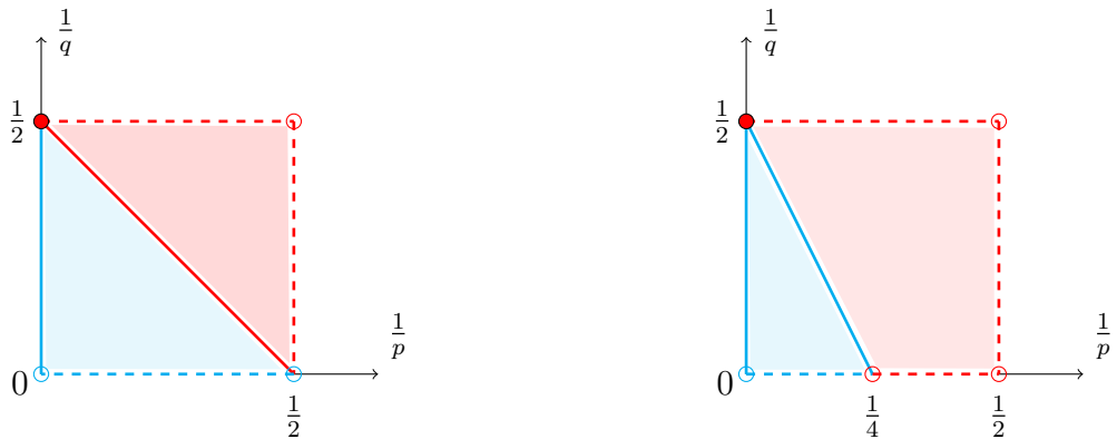
FIGURE 4.4 – Admissibility in dimension d = 3 and d = 2 .
