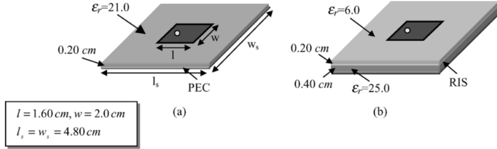
Figure 1.33: (a) Patch antenna over a conventional substrate (b) Patch antenna over a RIS substrate formed by a 4 \times 4 array printed on a dielectric material [19]
