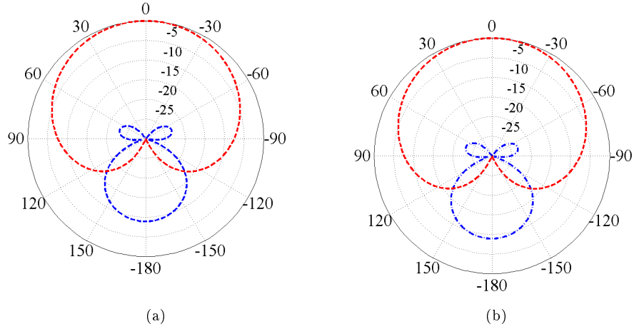
Figure 3.15: Computed normalized radiation patterns in dBic at 1578 MHz in two vertical cut planes: (a) \phi=0^\circ , (b) \phi=90^\circ . RHCP in red, and LHCP in blue
