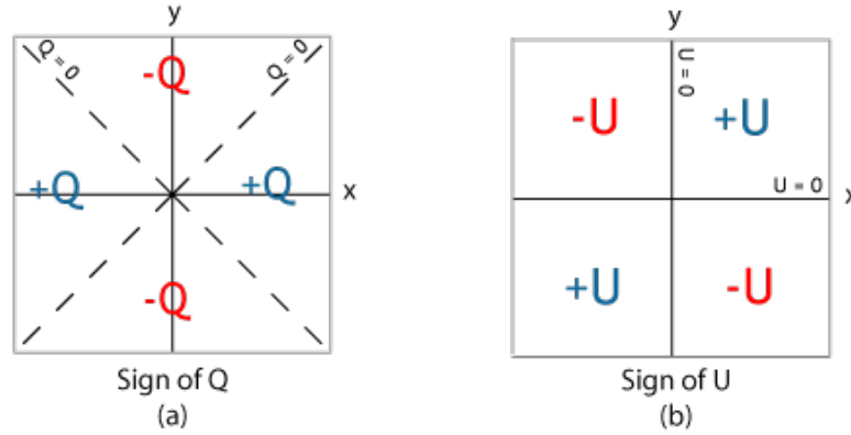
Figure 1.2: Sign of the parameters Q and U according to the orientation of the ellipse in the plane (\vec{x}, \vec{y}) . Credit: Dan Moulton
