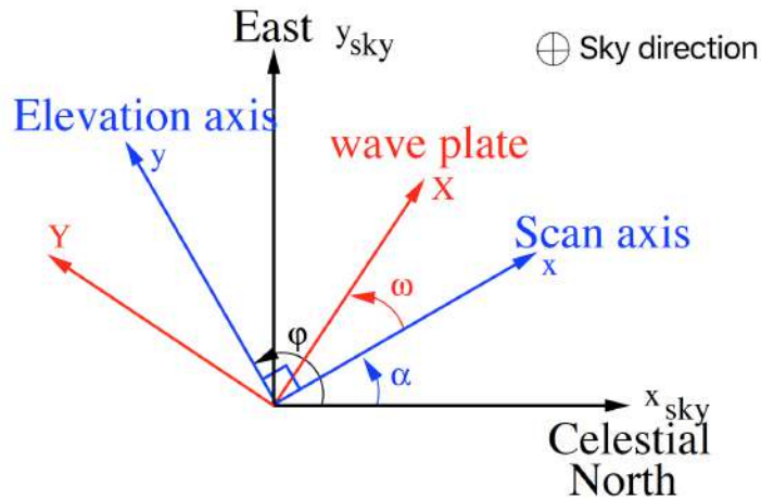
Figure 8.2: Definition of the angles involved in the determination of Stokes parameters. All angles are defined in algebraic value and are positively oriented in the the trigonometric direction defined in the figure, in accordance with the conventions.
