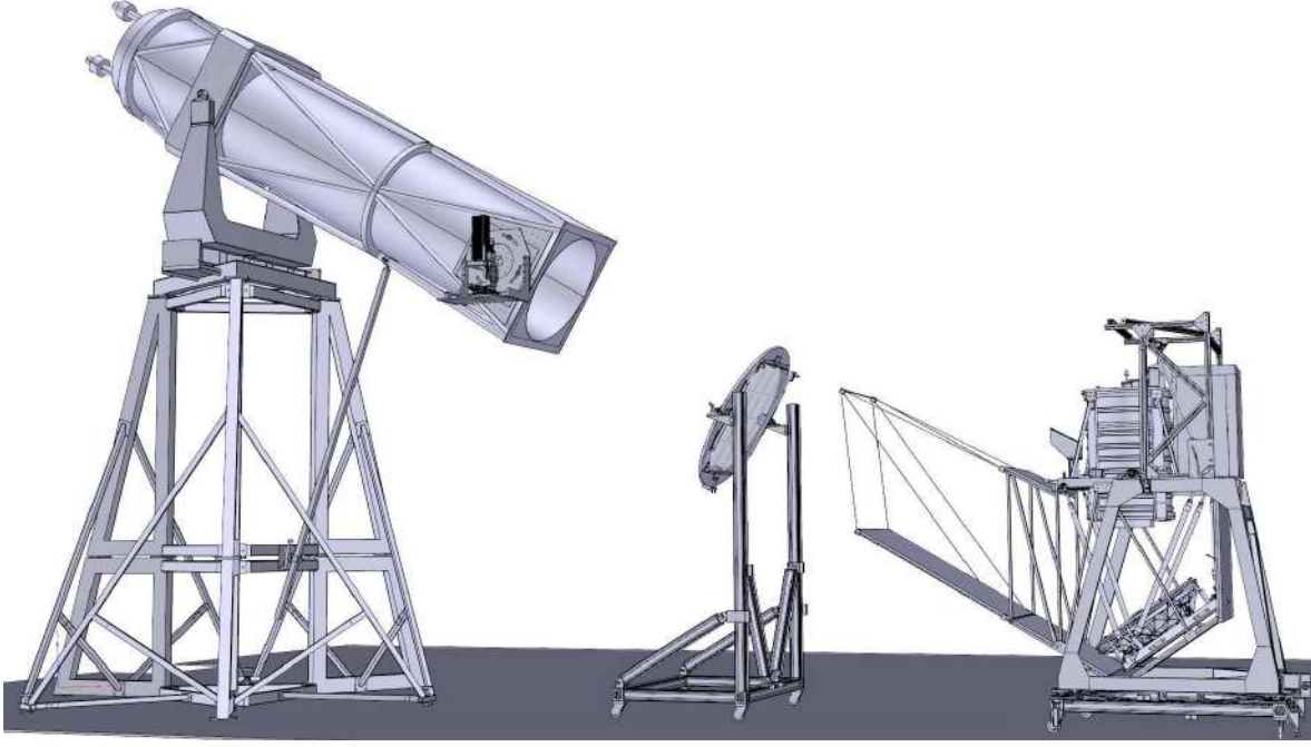
Fig. 15 Optical bench used to characterize polarization properties of the instrument. From right to left, the PILOT pointed load, the large format Archeops polarizer and the IRAP \phi = 1 m collimator.
