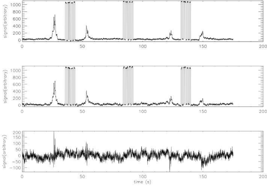
Figure 9.9: Example of a simulated time-line in the 240 \mu\text{m} channel for the average of all PILOT arrays for one observation of the Orion region. The plots show four consecutive scans, separated by calibrations on the ICS, which is visible in the time-lines as a strongly modulated signal. The upper and middle panels show time-lines for the TRANS and REFLEX arrays respectively. The large bumps in the data correspond to strong thermal dust emission in the Orion molecular cloud. The lower panel shows the difference between the two focal planes. The variations of the difference signal are due to the polarization of the simulated astrophysical emission.
