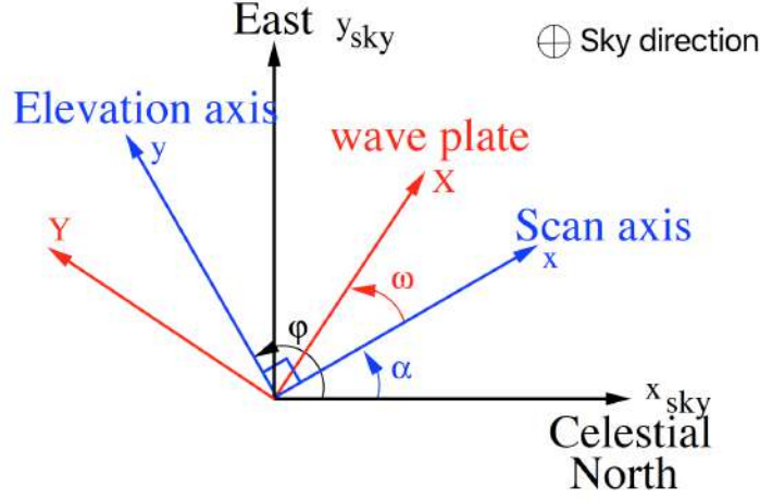
Figure 8.2: Definition of the angles involved in the determination of Stokes parameters. All angles are defined in algebraic value and are positively oriented in the trigonometric direction defined in the figure, in accordance with the conventions.
