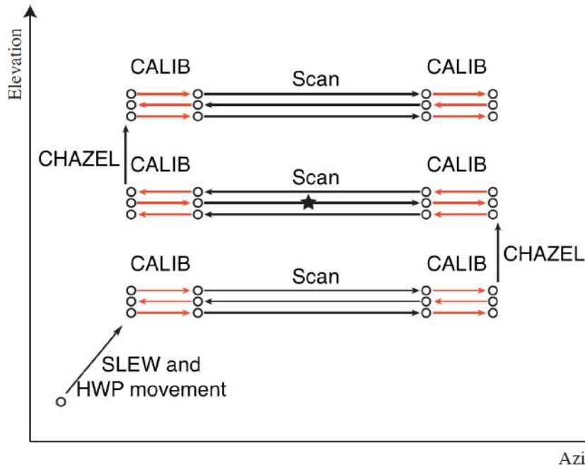
Figure 2.11: Schematic view of the decomposition of an observation sequence in individual gondola sequences. SLEW: passage between the end of a scene and the start of the next scene. SCAN: scans of a portion of a scene. CALIB: calibrations using the ICS. CHAZEL: relative displacements of the pointed load in azimuth and elevation.
