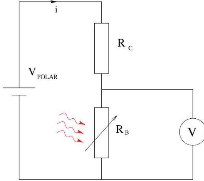
Figure 2.5: Electrical mounting, i.e. a voltage divider bridge, typically used to measure the signal across the thermistor. V_{\text{polar}} is the voltage source, R_C the load resistor and R_B the bolometer. Changes in the electric potential is measured across V . Figure from Billot (2007)
