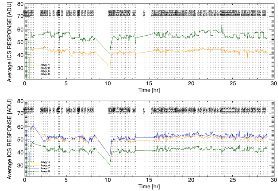
Figure 6.14: Variation of the array-averaged detector response to the ICS for arrays on the TRANS (top) and REFLEX (bottom) focal planes during the second flight. Colours indicate different arrays. The vertical dashed lines indicate boundaries between different observing
