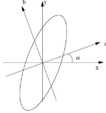
Figure 8.1: Relative orientation convention of the bases (x,y) and (a,b) in which we seek the Stokes parameters of the polarization ellipse represented here
