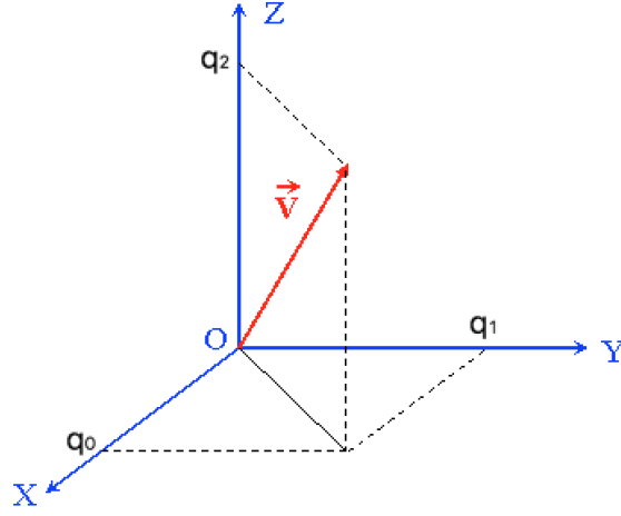
Figure 4.4: Spatial representation of quaternions.
