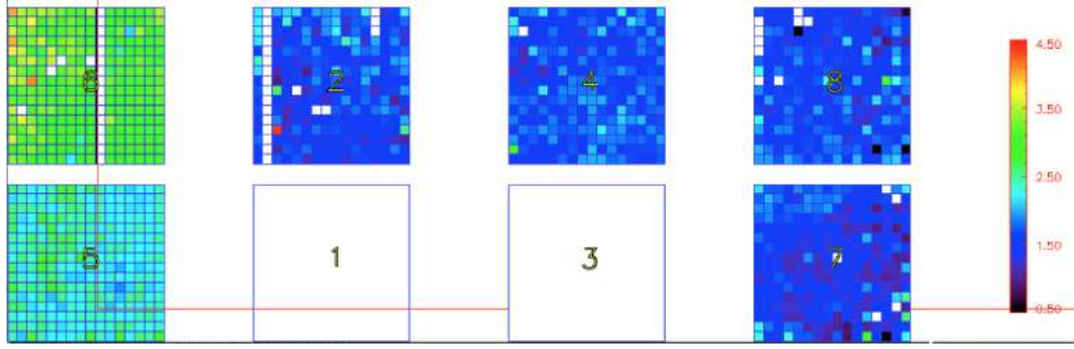
Figure 3.6: Image of the bolometers time constant obtained during IAS tests after correcting timelines for the ICS time constants and data-reading time delay. Values are in sample number. Arrays 1 and 3 were not operational during these tests.
