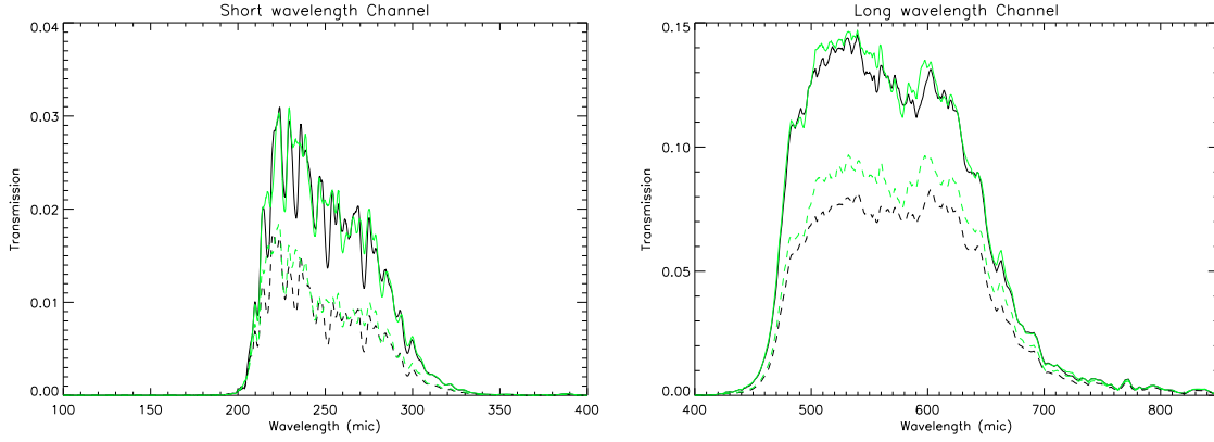
Fig. 10 Instrumental transmission in the 240\mu\text{m} and 550\mu\text{m} channel as predicted using the photometric model, for HWP positions of 0^\circ (black curve) and 45^\circ (green curve), on the transmission and reflection arrays respectively. The transmission values shown include polarizer transmission and detector absorption.
