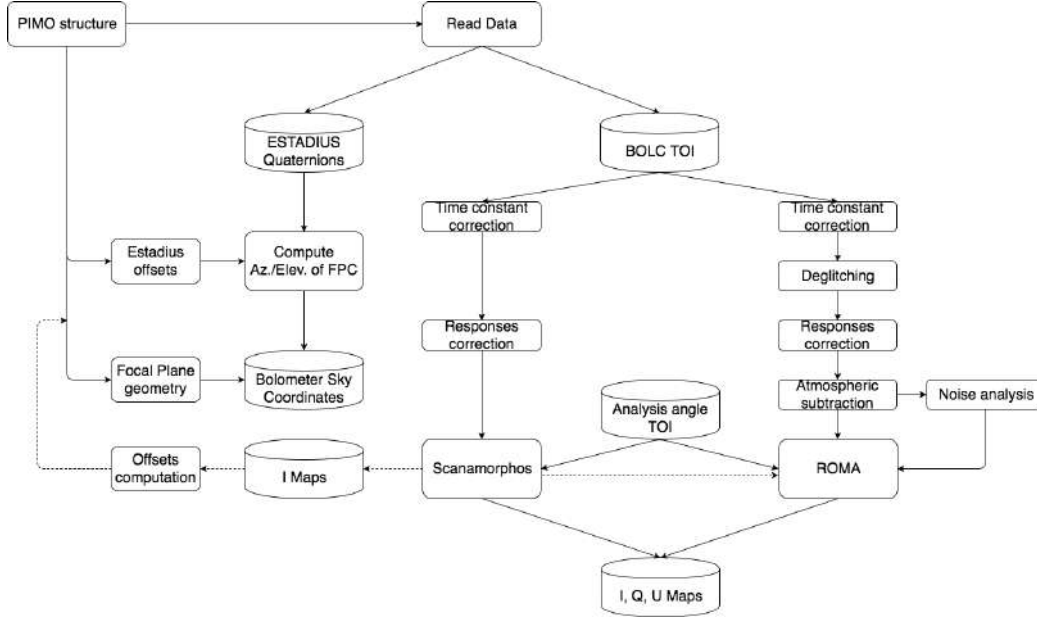
Figure 9.2: Schematic view of the data processing pipeline. The disks represent the data read or generated by the different routines and the rectangle are the data processing routines. The dashed arrows and lines represent processing steps that are added as the iterations proceed.
