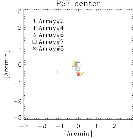
Figure 7.4: PSF center position obtained on Jupiter during the second flight.
