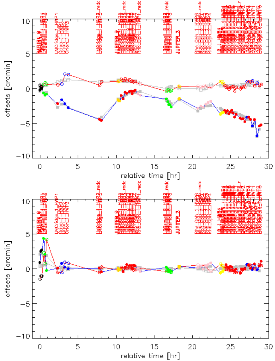
Figure 4.9: Top: Averaged cross-elevation and elevation offsets measured during Flight#2 before applying the model correction. Bottom: Same but after application of the pointing model correction. The red curves correspond to the cross-elevation offset and blue curves to the elevation offsets. The gray curves show the prediction of the current pointing model described in eqs. 4.21 and tab 4.2.
