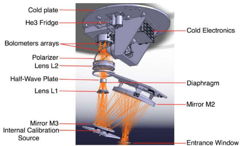
Figure 2.3: Schematic diagram of the PILOT optics
