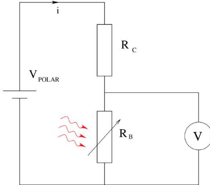
Figure 2.5: Electrical mounting, i.e. a voltage divider bridge, typically used to measure the signal across the thermistor. V_{polar} is the voltage source, R_C the load resistor and R_B the bolometer. Changes in the electric potential is measured across V . Figure from Billot (2007)
