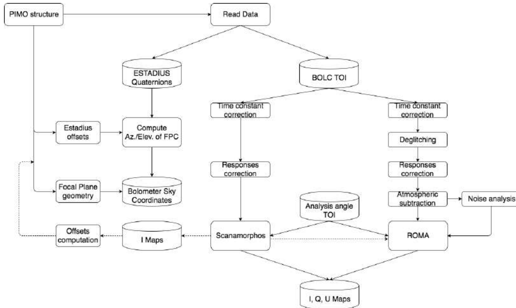
Figure 9.2: Schematic view of the data processing pipeline. The disks represent the data read or generated by the different routines and the rectangles are the data processing routines. The dashed arrows and lines represent processing steps that are added as the iterations proceed.
