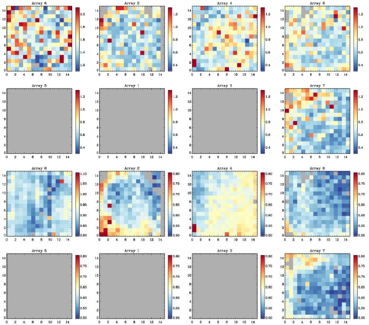
Fig. 4: Top: Focal plane distribution of the bolometer time constants as measured from glitches \tau_{gli} . Bottom: Focal plane distribution of the bolometers time constants \tau_{det} as measured using the ICS downward transitions. The four arrays shown on the left (resp. right) belong to the TRANS (resp. REFLEX) focal planes, such that arrays #6 and #4 (or arrays #2 and #8) are optical conjugates. In this representation, elevation increases towards the top-left and cross-elevation increases towards the top-right corner of each focal plane. The same convention and array numbering is used for all figures of the paper.
