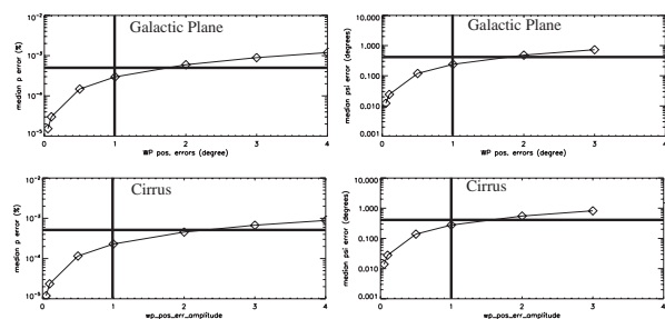
Fig. 14 Error on the polarization degree (left) and polarization angle (right) as a function of the angular positional error of the HWP for a standard cirrus observation of the Galactic plane (upper panel) and of a diffuse cirrus cloud (lower panel). The criterion used to set the requirement on this parameter is indicated by the thick horizontal line.
