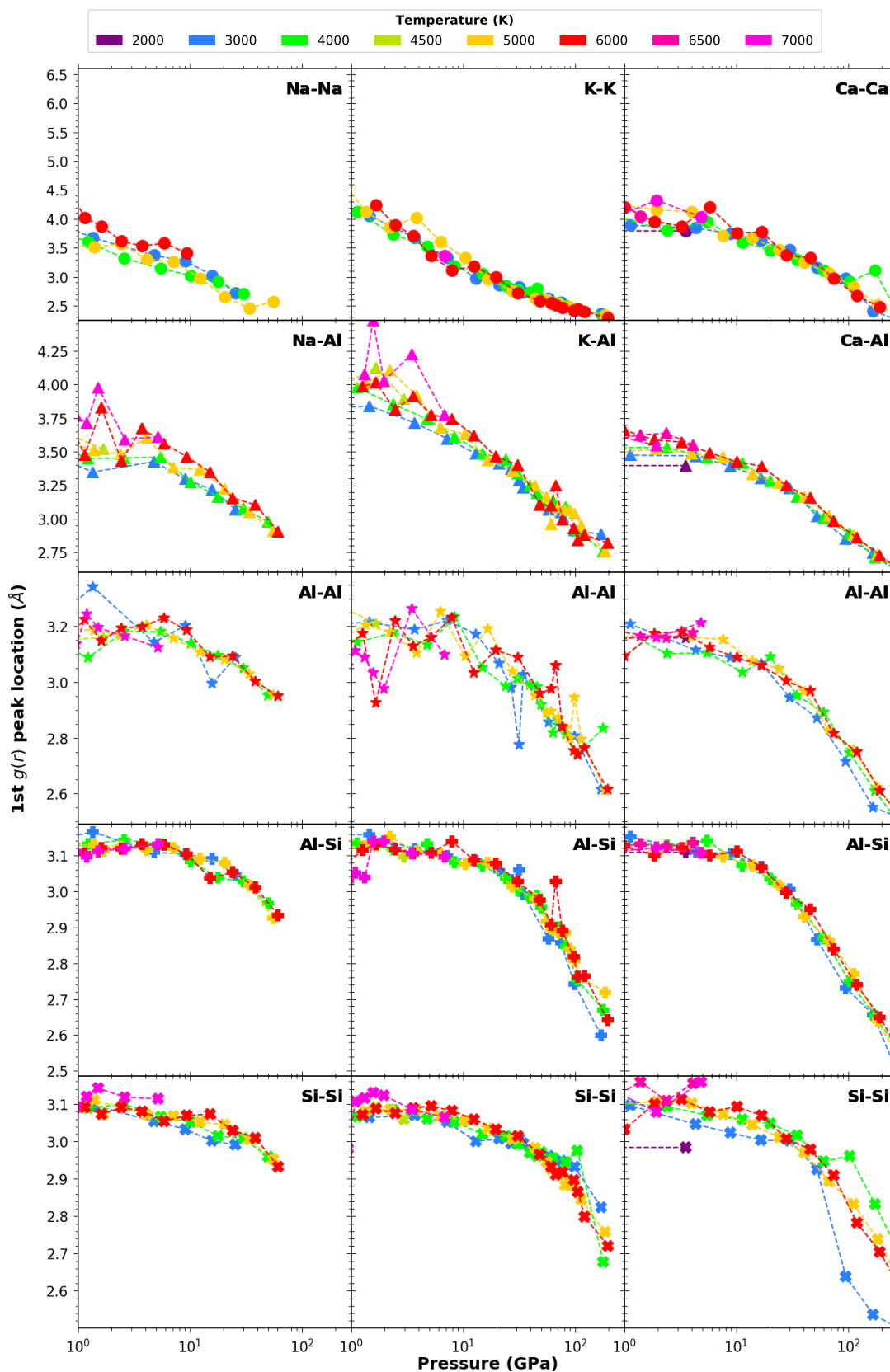
Figure 3.8 – Position of the first g(r) peak for each feldspar end-member (columns) as a function of pressure and temperature (colors) for five cation pairs. The same figure as a function of density instead of pressure is presented figure A.5.
