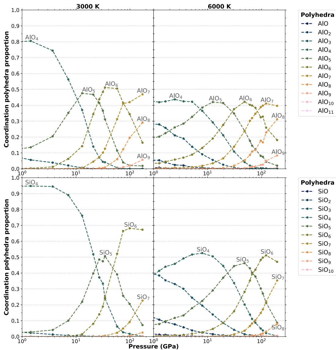
Figure 3.12 – Relative proportion of \text{SiO}_n and \text{AlO}_n coordination species in \text{KAlSi}_3\text{O}_8 for 3000 K and 6000 K as a function of pressure. The same figure as a function of density is available in annex, figure A.8.
