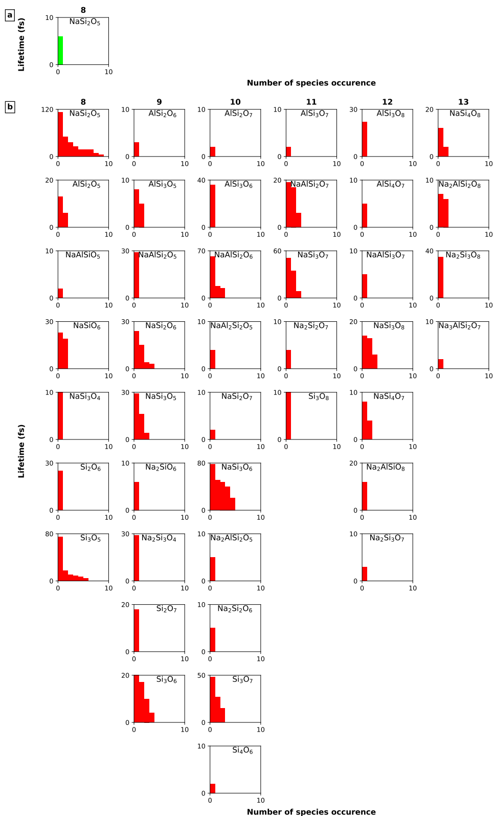
Figure A.17 – Lifetime of each individual volatile species with 8 to 13 atoms in their formula in NaAlSi 3 O 8 fluids at 1.0 g cm -3 and (a) 4000 K, (b) 6000 K. The species with less than 8 atoms in their formula are available in figure 4.8.
