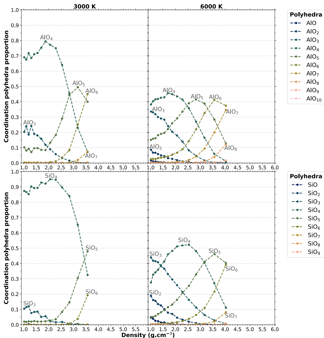
Figure A.7 – Relative proportion of \text{SiO}_n and \text{AlO}_n coordination species in \text{NaAlSi}_3\text{O}_8 for 3000 K and 6000 K as a function of density. The same figure as a function of pressure is displayed figure 3.11.
