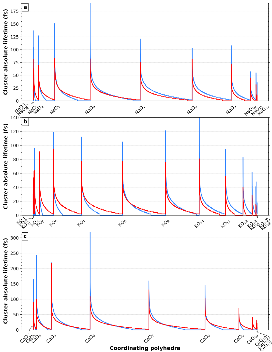
Figure 3.19 – Same as Fig. 3.15 for NaO n , KO n and CaO n coordinating polyhedra.
