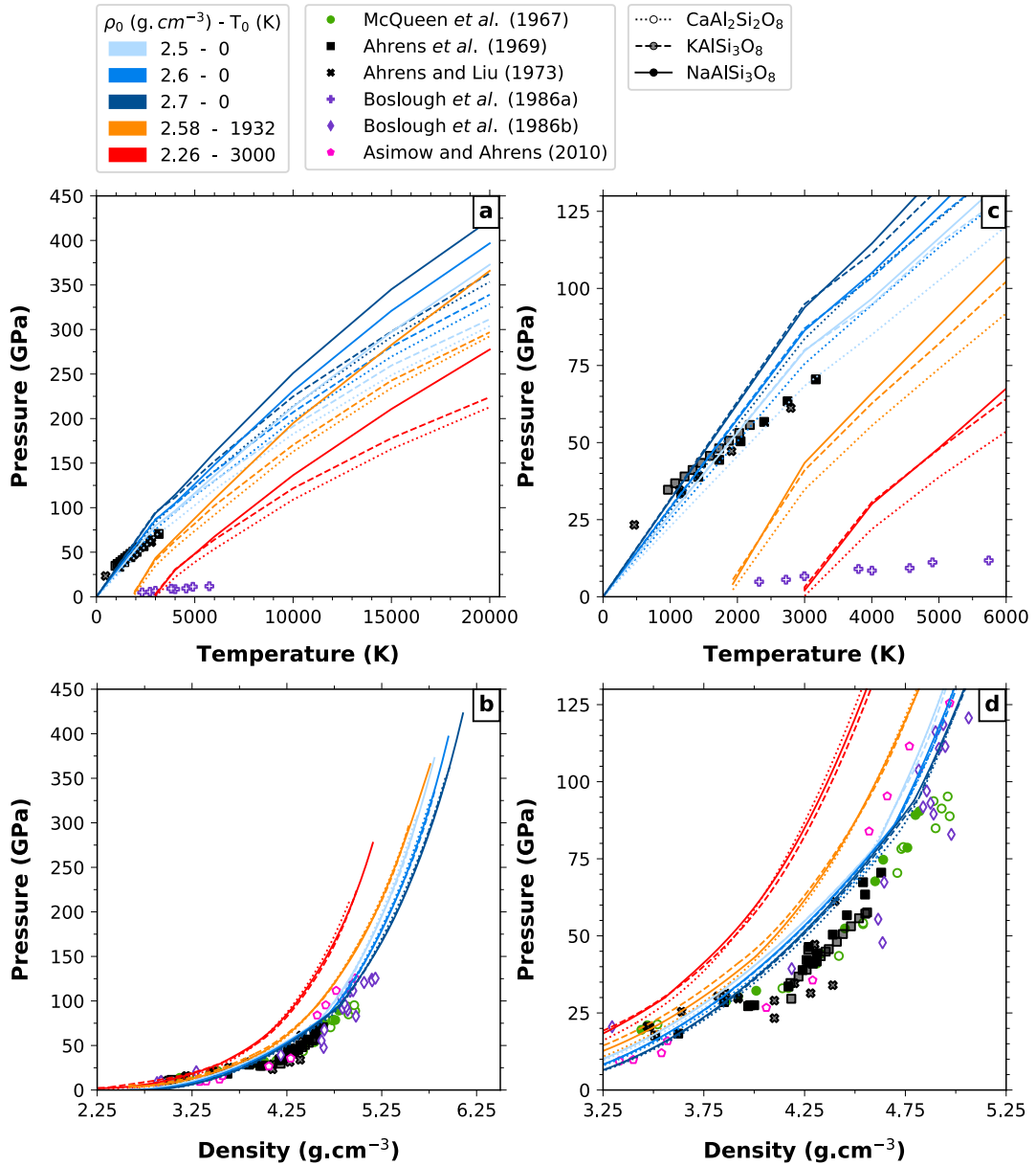
Figure 6.10 – Hugoniot curves for each initial temperature and density of the crust (colors) on several projections: (a) pressure-temperature, (b) pressure-density and their associated zoom on the low pressure range (c) and (d). Data from experiments on feldspars are indicated by the colored markers. The feldspars composition is represented by the line styles for the Hugoniot curves and by the markers filling for the experimental data: solid symbols - NaAlSi 3 O 8 , half transparent symbols - KAlSi 3 O 8 , open symbols - CaAl 2 Si 2 O 8 . A cubic interpolation is used to smooth the Hugoniot curves in the pressure-density projection. The same figure for the last projection (temperature-density) is available in annex, figure A.30.
