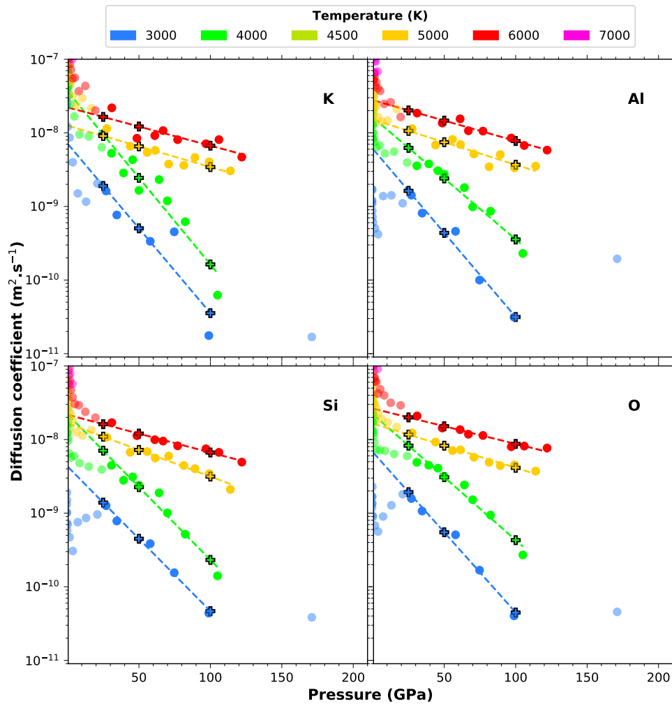
Figure A.23 – Self-diffusion coefficients in \text{KAlSi}_3\text{O}_8 as a function of pressure and Arrhenius fit in the 25–150 GPa range. Colors indicate temperatures. Crosses indicate the diffusion values estimated from the fit at 25, 50 and 100 GPa.
