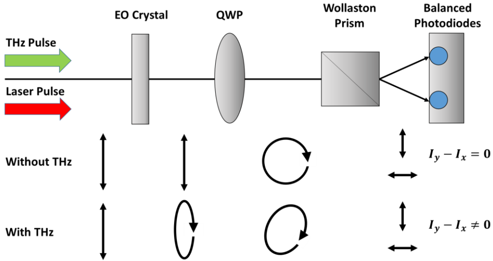
Figure 2.6: Electro-optic sampling
