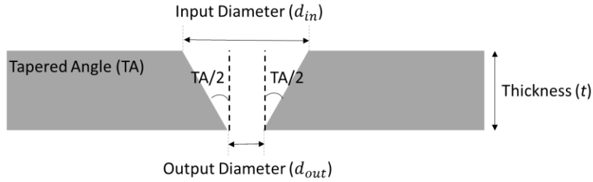
Figure 4.4: Diagram showing the conically tapered aperture
