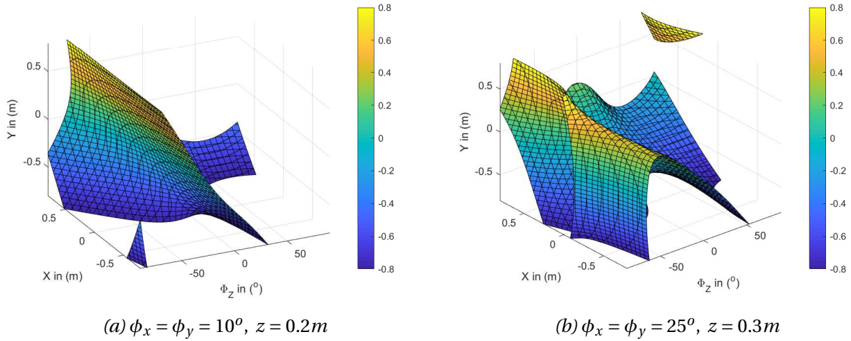
Figure 3.22: Singularity locus in 3D Cartesian space.
