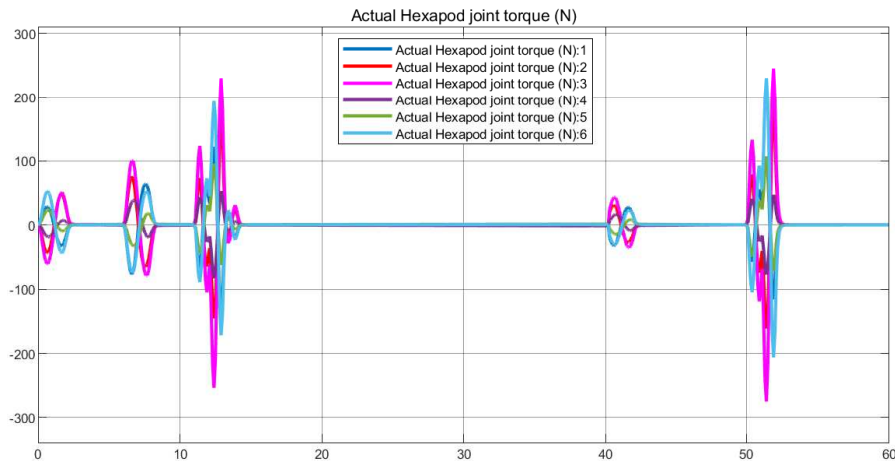
Figure 5.21: Hexapod control input for PSO-based SMC
