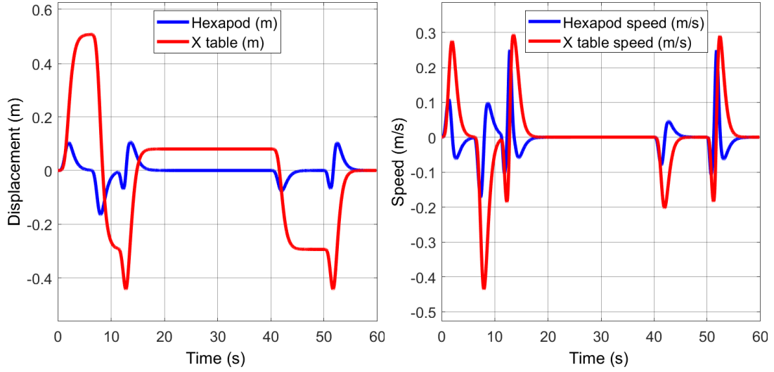
Figure 4.26: Hexapod and X Table displacements and speeds
