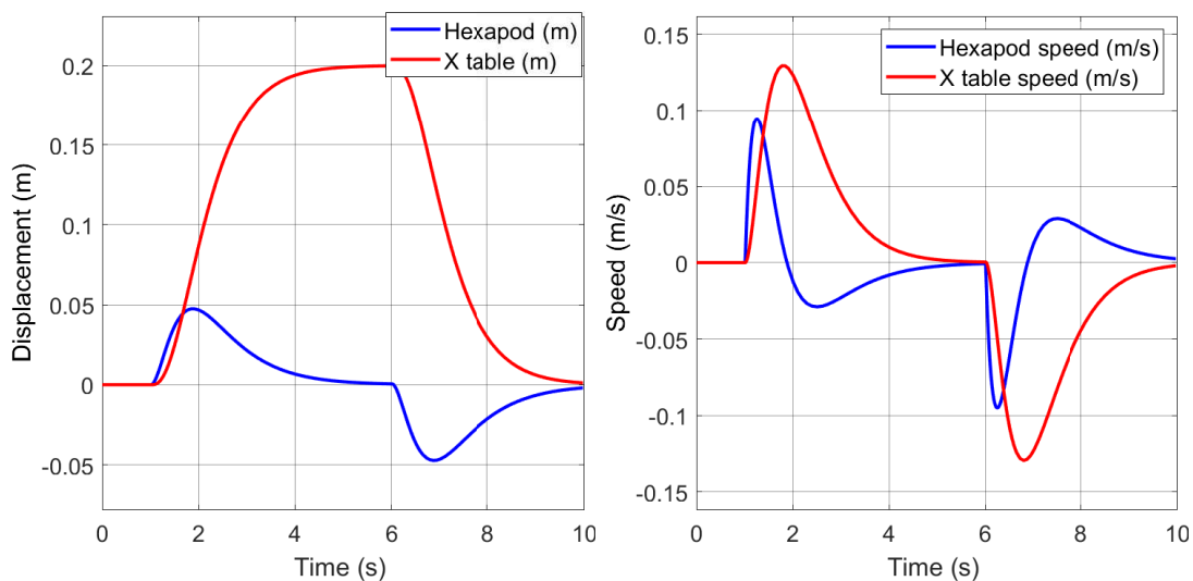
Figure 4.22: Hexapod and X Table displacements and speeds
