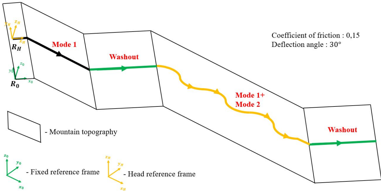
Figure 4.12: Predefined trajectory
