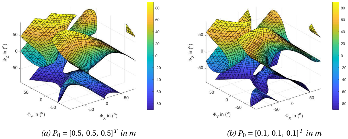
Figure 3.21: Singularity loci in 3D Cartesian space with constant positions.
