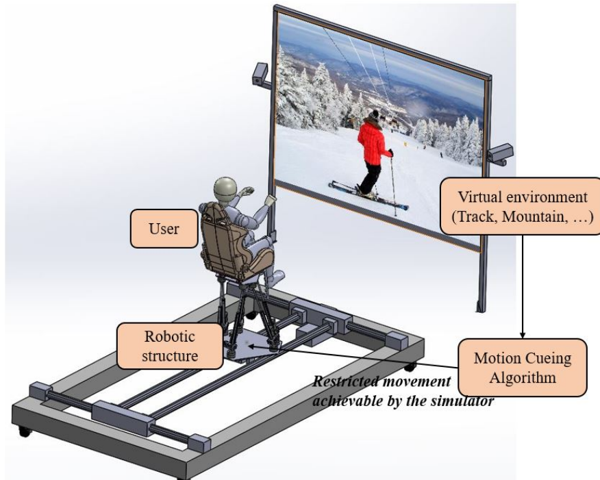
Figure B.1: General ski simulator components
