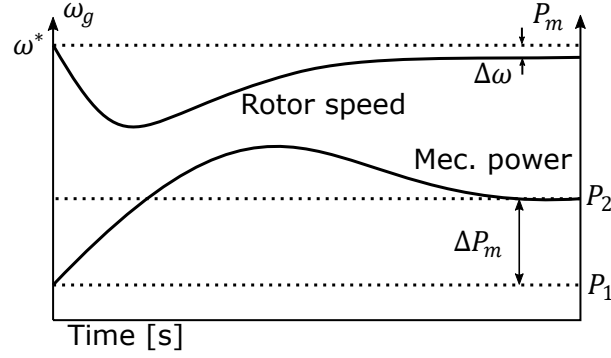
Figure 5.6: Frequency response in the droop control mode.
