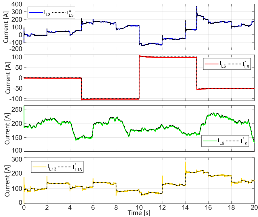
Figure 4.45: The controlled currents I_{L3} , I_{L6} , I_{L9} and I_{L12} .
