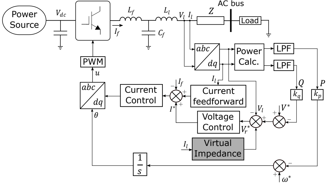
Figure 2.5: Power converter control of a Microgrid applying virtual output impedance loop.
