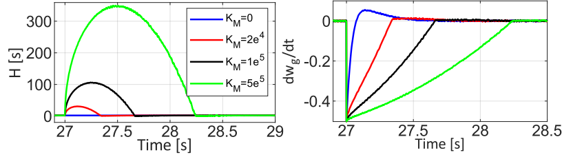
Figure 5.48: Inertia coefficient on the left and angular acceleration on the right over different values of K_M .
