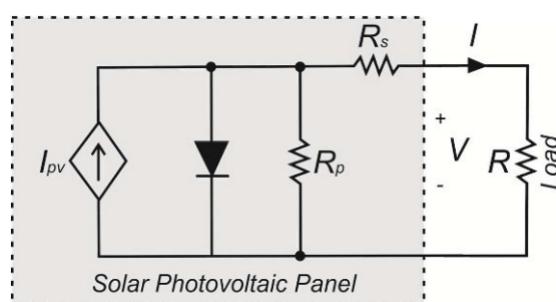
Figure 3.1: Simplified model of photovoltaic panel.
