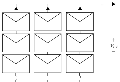
Figure 3.5: Parallel and series arrangement of PV arrays.
