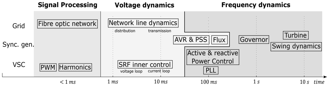
Figure 5.12: Time-scale separation of power system dynamics considering conventional synchronous generators and power converters integration.
