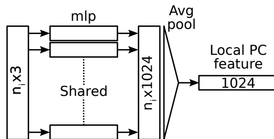
(c) Local feature module. For each local point cloud, a feature is computed with an MLP network. The problem of the unordered and unsorted structure is solved with an average pooling layer. The output is the feature of the local point cloud. The local module is shared by all the local point cloud of a same scale.
