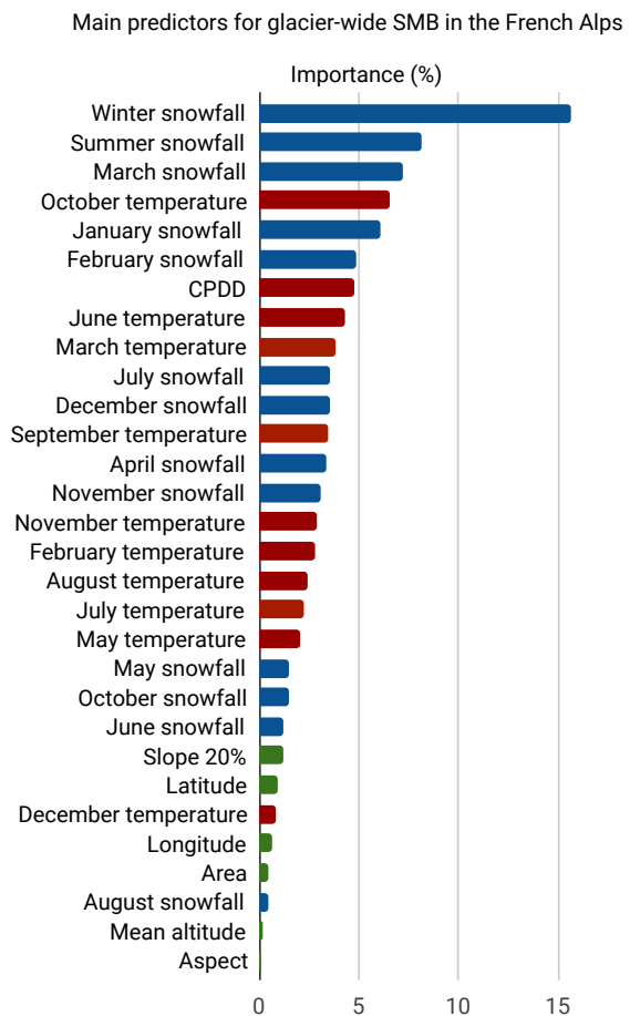
Figure 2.5: Contribution to the total variance of the 30 top topo-climatic predictors out of 55 predictors using Lasso. Green bars indicate predictors including topographical features, blue ones including accumulation-related features, and red ones including ablation-related features
