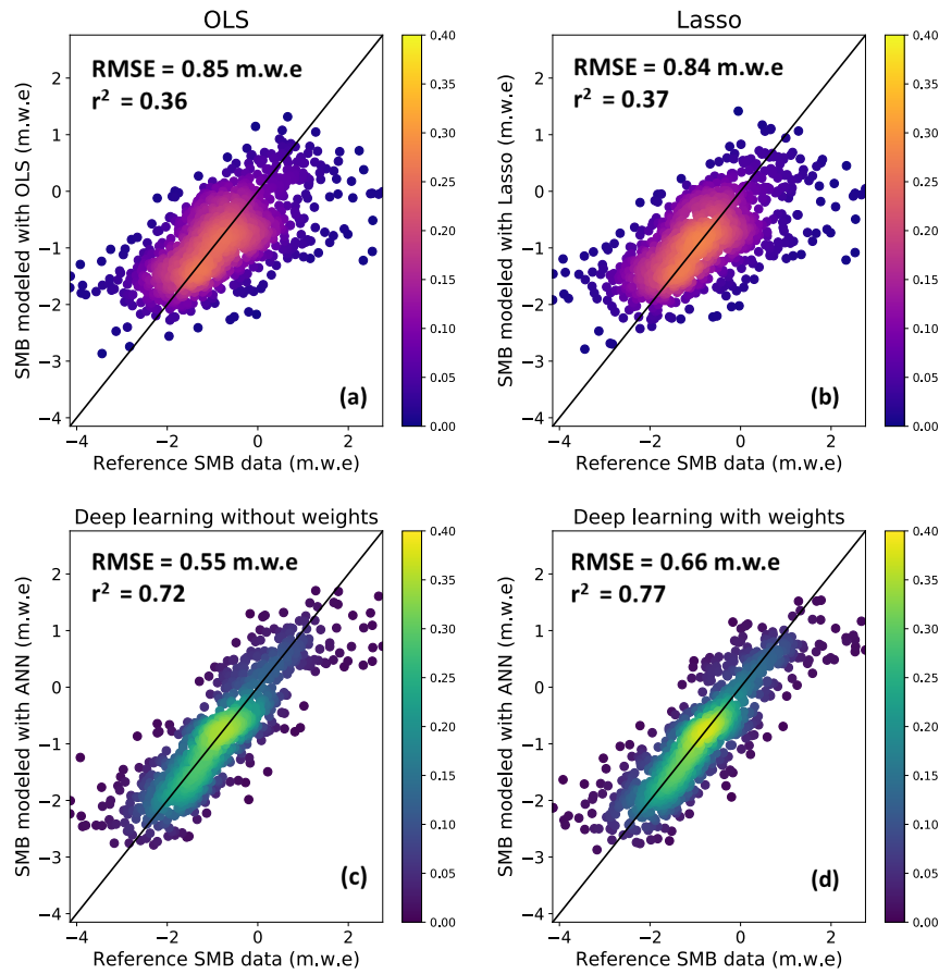
Figure 2.9: Evaluation of modelled annual glacier-wide SMB against the ground truth SMB data (both in m.w.e. a^{-1} ) using Leave-One-Year-Out cross-validation. The colour (purple-orange for linear; blue-green for nonlinear) indicates frequency based on the probability density function. The black line indicates the reference one-to-one line. a) Scatter plot of the OLS model results; b) Scatter plot of the Lasso linear model results; Scatter plots of the deep artificial neural network nonlinear models without (c) and with sample weights (d).
