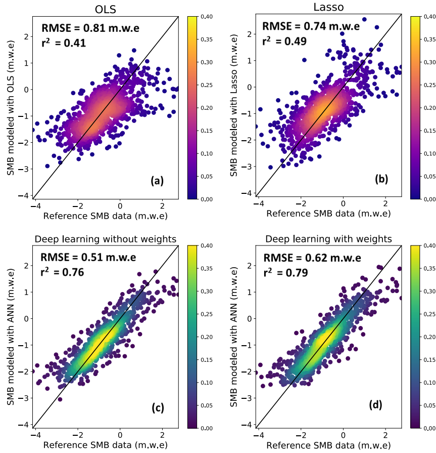
Figure 2.6: Evaluation of modelled annual glacier-wide SMB against the ground truth SMB data (both in m.w.e. \alpha^{-1} ) using Leave-One-Glacier-Out cross-validation. The colour (purple-orange for linear; blue-green for nonlinear) indicates frequency based on the probability density function. The black line indicates the reference one-to-one line. a) Scatter plot of the OLS model results; b) Scatter plot of the Lasso linear model results; Scatter plots of the deep artificial neural network nonlinear models without (c) and with sample weights (d)
