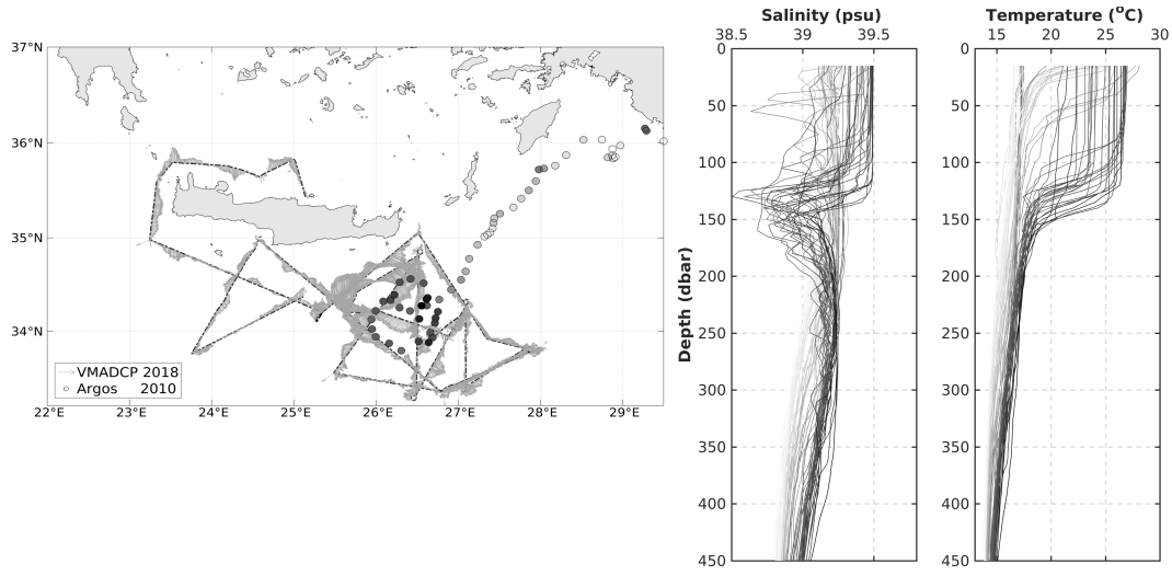
Figure 1.5: (a) VMADCP measurements during PROTEVS-PERLE campaign leg 2 held in 2018 in the Levantine basin. (b) The trajectory of an Argos float drifted in the Northern Levantine from February to December 2010 where it was captured in the Ierapetra eddy in 2010 c) Temperature and Salinity measurements from Argos profile along its trajectory in winter 2010.
