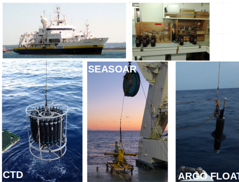
Figure 1.4: Monitoring the ocean vertical extend during field campaigns. Few of the different measurement equipments used are illustrated.
