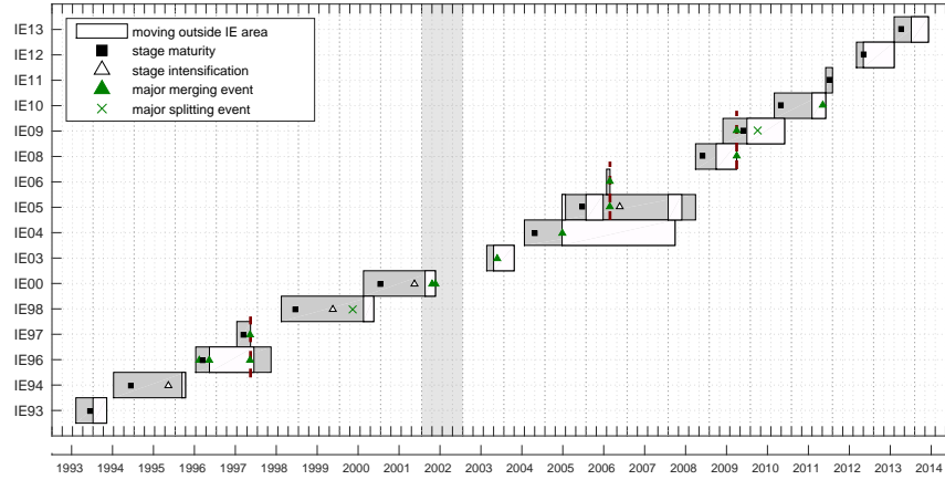
Figure 2.9: Chronology of the various dynamical events (formation, maturity (black square), intensification (open triangle), mergings (green triangle) or splittings (green crosses) ) for all the IEs detected between 1993 and 2015. The gray (white) areas indicate the position of each IE centers inside (outside) the mean IE area depicted in Figure 2.3 and Figure 2.8. The vertical dashed red lines indicate mergings between IEs.
