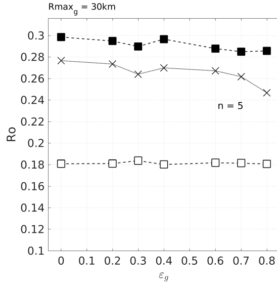
Figure 3.10: Evolution of the vortex Rossby numbers for geostrophic (open square) and cyclogeostrophic (filled square) elliptical anticyclones as a function of their ellipticity \varepsilon = 1 - b/a , where a and b are respectively the semi-major and semi-minor axis. The elliptical velocity fields were obtained from the deformation (Eqn.(10) - Eqn.(13)) of a circular Gaussian velocity profile having a characteristic radius R_{max} = 30 \text{ km} and a maximum azimuthal speed V_{max} = 0.9 \text{ m.s}^{-1} . The vortex Rossby numbers of the elliptical eddies obtained by the iterative scheme Eqn.(6) applied to the geostrophic solutions are plotted with crosses.
