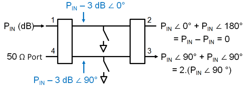
Figure 101: Operating principle of the SPDT switch in RX state
