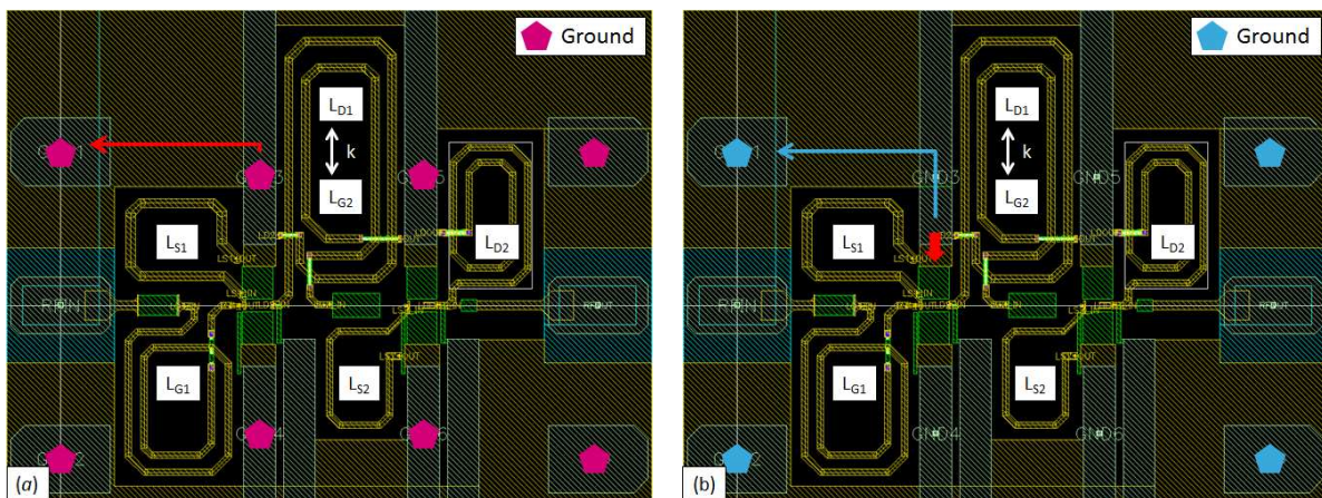
Figure 118: Layout top view including the simulation virtual ground pads: (a) First simulation; (b) Retro-simulation
