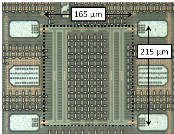
Figure 106: Micrograph of the asymmetrical SPDT switch
