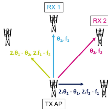
Figure 24: Undesired beams due to the intermodulation products
