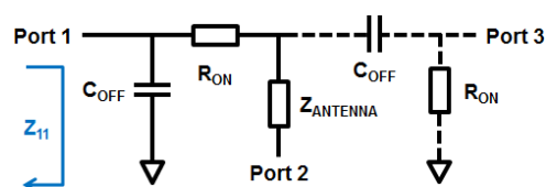
Figure 86: Series-shunt SPDT switch equivalent schematic
