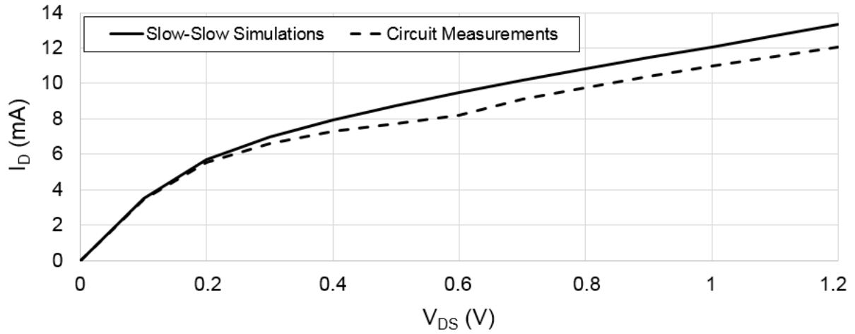
Figure 49: Simulated and measured I_D (V_{DS}) of a 40 \mu\text{m} GO1 FB NMOS device, at V_{GS} = 0.8 \text{ V}
