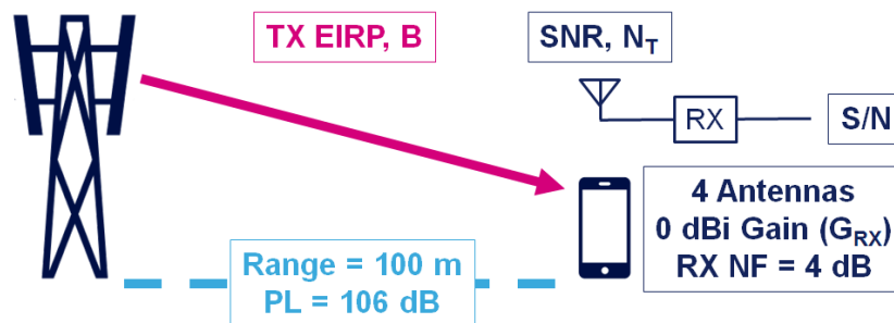
Figure 18: Wireless link in the chosen use case
