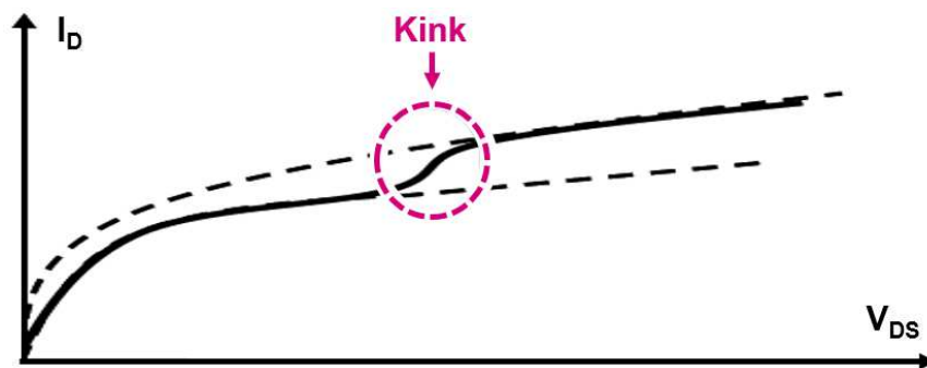
Figure 35: The I(V) characteristic of a PD-SOI transistor with kink effect, from [3]
