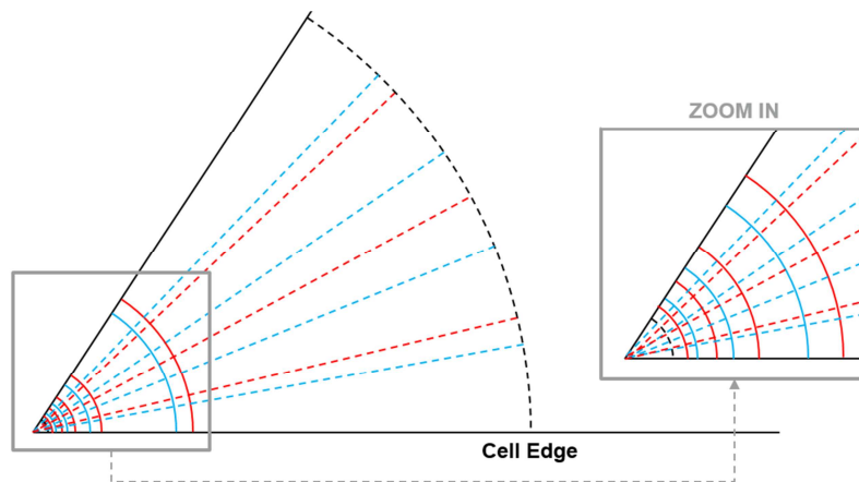
Figure 20: Beam projection on the ground for 10 x 10 (red), and 12 x 8 (blue) arrays
