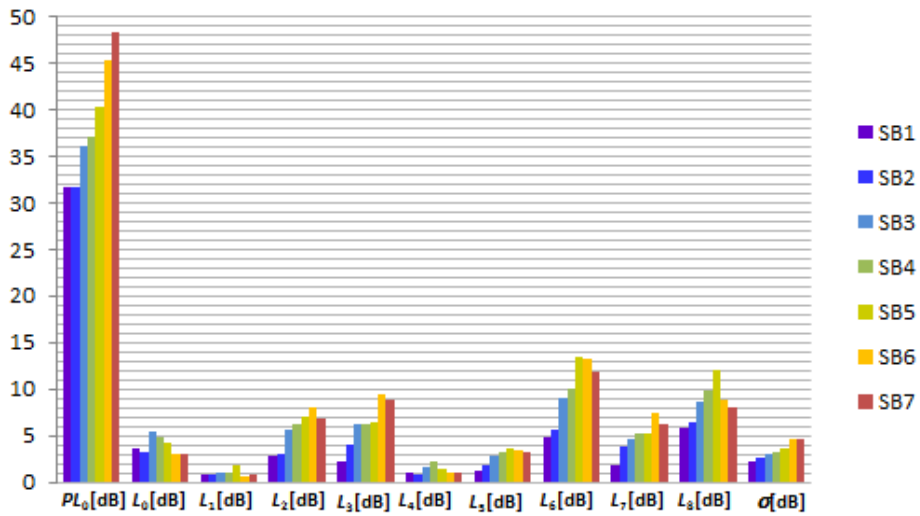
Figure 3.6. Parameters of the D-MWM
