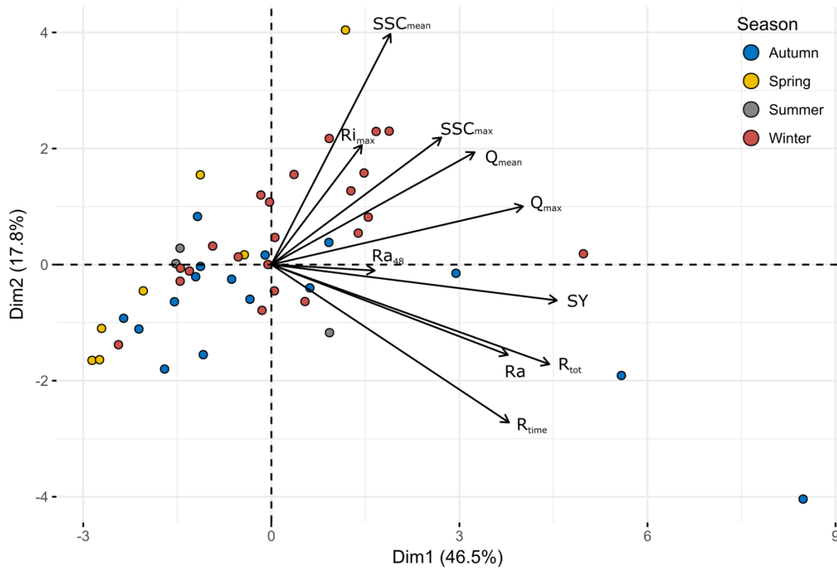
Fig. 25 : Bi-plot of PCA results on dimensions 1-2 for the 48 events and their hydro-sedimentary parameters: (i) duration of the rainfall event ( R_{time} , min), (ii) rainfall amount ( R_a , mm), (iii) max 6-min rainfall intensity ( R_{i_{max}} , \text{mm h}^{-1} ), (iv) 48h-antecedent rainfall ( R_{a_{48}} , mm), (v) mean flow and peak flow ( Q_{mean} , Q_{max} , \text{m}^3 \text{h}^{-1} ), (vi) mean and maximum SSC concentration ( SSC_{mean} , SSC_{max} , \text{g l}^{-1} ), (viii) sediment yield ( SY , kg), and (ix) total runoff ( R_{tot} , \text{m}^3 ).
