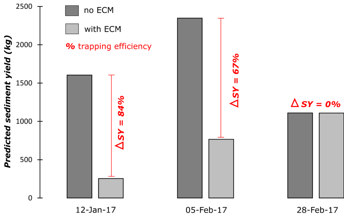
Fig. 39 : Results of the sediment yield model predictions (kg) with/without erosion control measure on the Pommeroye catchment for the three rainfall events.
