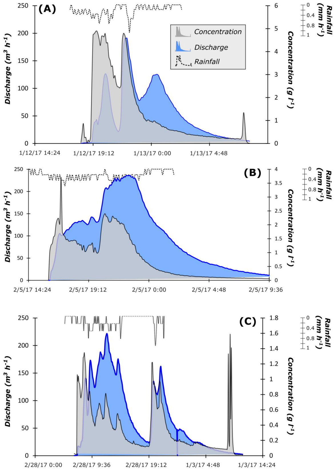
Fig. 33 : Flow discharge ( m^3 h^{-1} ), sediment concentration ( g L^{-1} ) and rainfall ( mm h^{-1} ) for three events recorded at the monitoring station at the outlet of the Pommeroye catchment: (A) January 12, 2017, (B) February 5, 2017, and (C) February 28, 2017.
