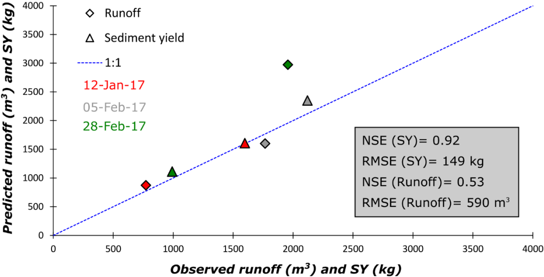
Fig. 36 : Results of the model predictions and comparison to the observed sediment yield (kg) and runoff (m 3 ). The 1:1 curve indicates that predicted data closed to the dotted line fits closely to the observed data.
