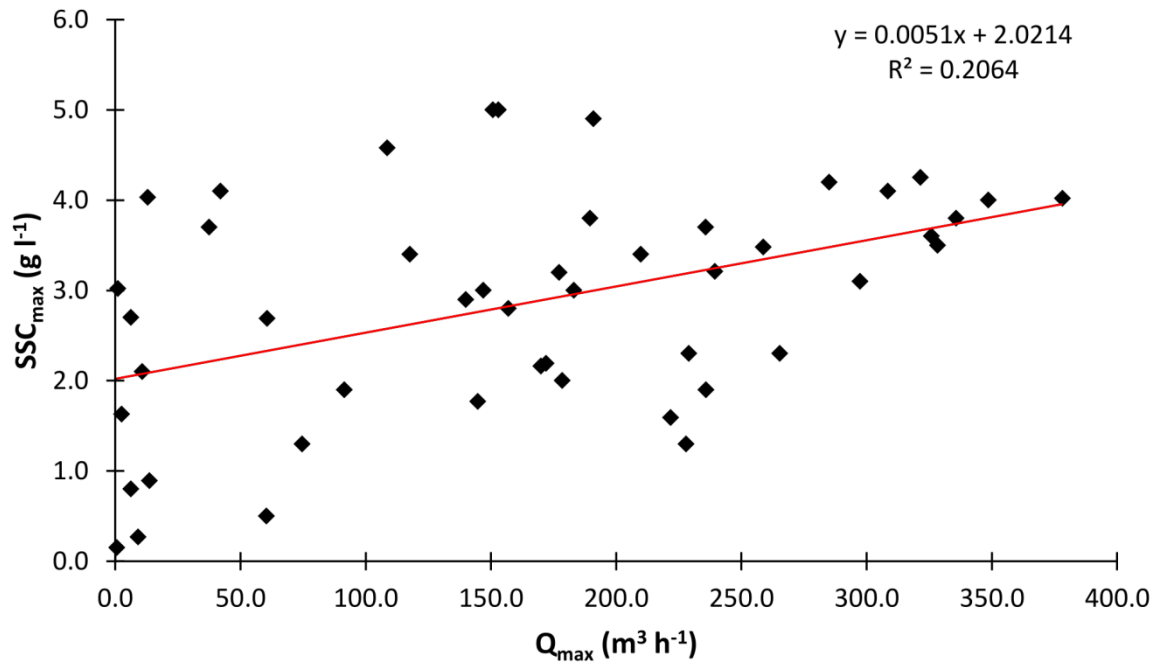
Fig. 20 : Relationship between the maximum suspended sediment concentration ( \text{g l}^{-1} ) and the maximum flow ( \text{m}^3 \text{h}^{-1} ) after 2 years of monitoring in the Pommeroye catchment.
