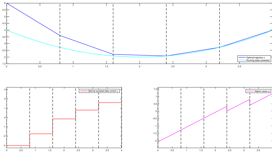
Figure 3.4: Example 1 with N = 5 .
