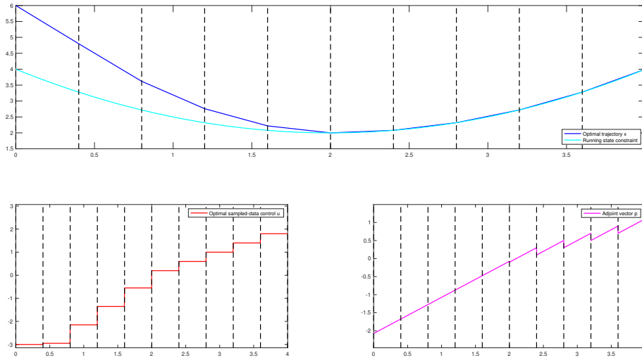
Figure 3.5: Example 1 with N = 10 .
