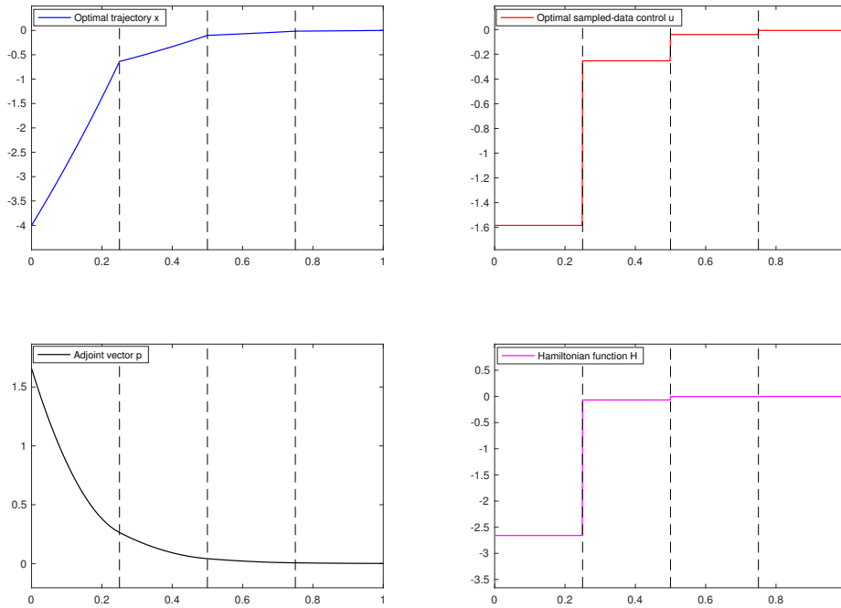
Figure 2.3: The case N = 4 of Problem (\text{OSCP}_{\text{alq}}) with fixed uniform partition.
