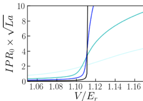
Figure 4.7: Plots of the quantity IPR_0 \times \sqrt{La} as a function of the potential amplitude V for the balanced bichromatic lattice and different system lengths. Darker lines correspond to increasing system sizes, L/a = 200 (light blue), 1000 (blue), 5000 (dark blue), 10000 (black).
