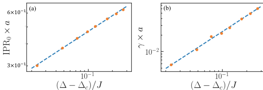
Figure 4.14: The ground state IPR and Lyapunov exponent \gamma for the AA model near the transition point \Delta_c (data points plotted as yellow balls). Here, both of the two plots are in log-log scale. In both cases, with a linear fit (blue dashed line), we find the slopes \nu \simeq 0.33 \pm 0.015 for (a) and \beta \simeq 0.96 \pm 0.04 for (b).
