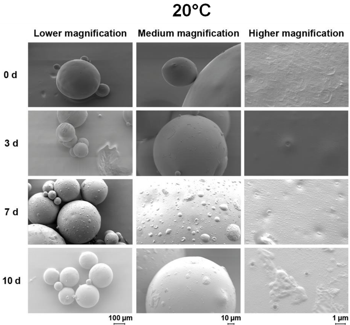
Figure III-23: SEM pictures of surfaces (lower, medium and higher magnification) of diprophylline-loaded PLGA microparticles before and after exposure to phosphate buffer pH 7.4 (treated as for drug release studies from ensembles of microparticles) at 20 °C (80 rpm). The exposure times are indicated on the left hand side. Note that the microparticles were freeze-dried after exposure to the release medium.
