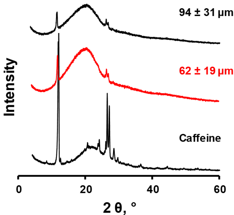
Figure III-16: X-ray diffraction patterns of ensembles of caffeine-loaded PLGA microparticles (mean diameters +/- standard deviations are indicated), and of caffeine raw material (as received) for reasons of comparison.
