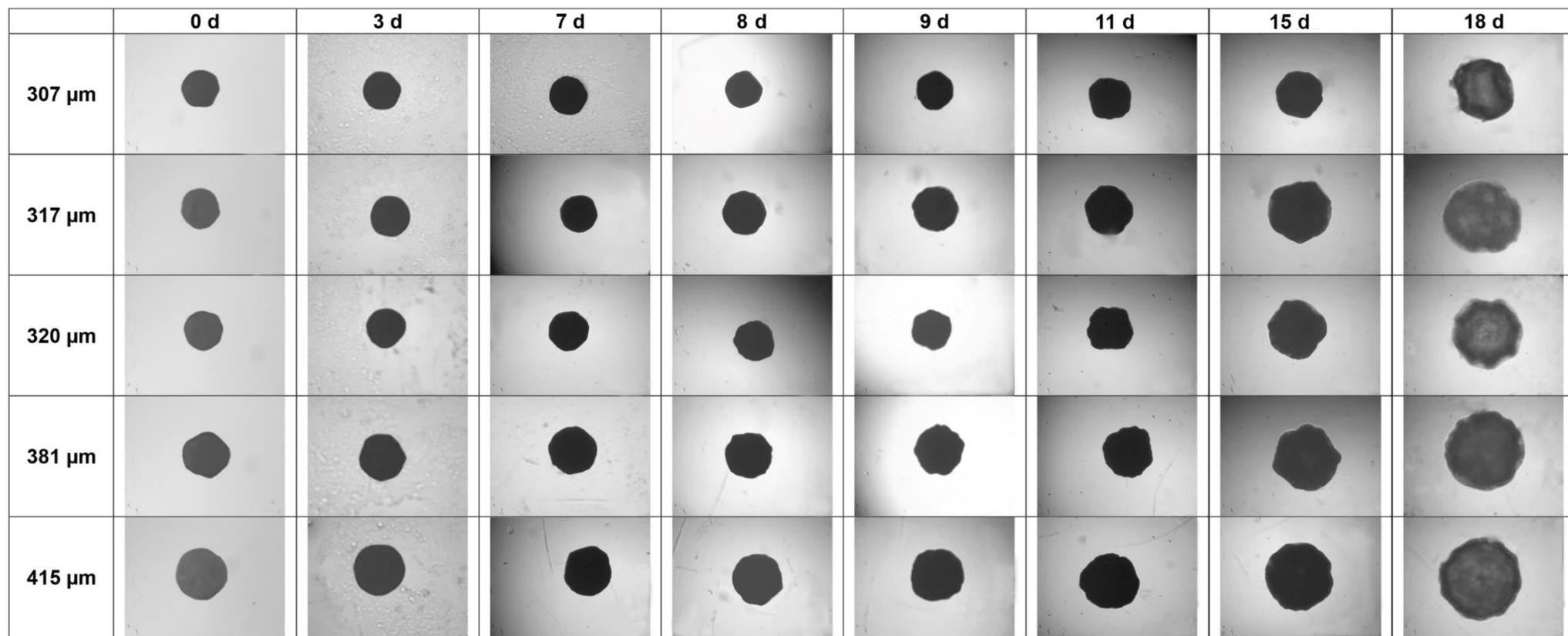
Figure III-17: Optical microscopy pictures of single caffeine-loaded PLGA microparticles before and after exposure to phosphate buffer pH 7.4 for different time periods (indicated at the top). The initial particle size is given on the left-hand side.
