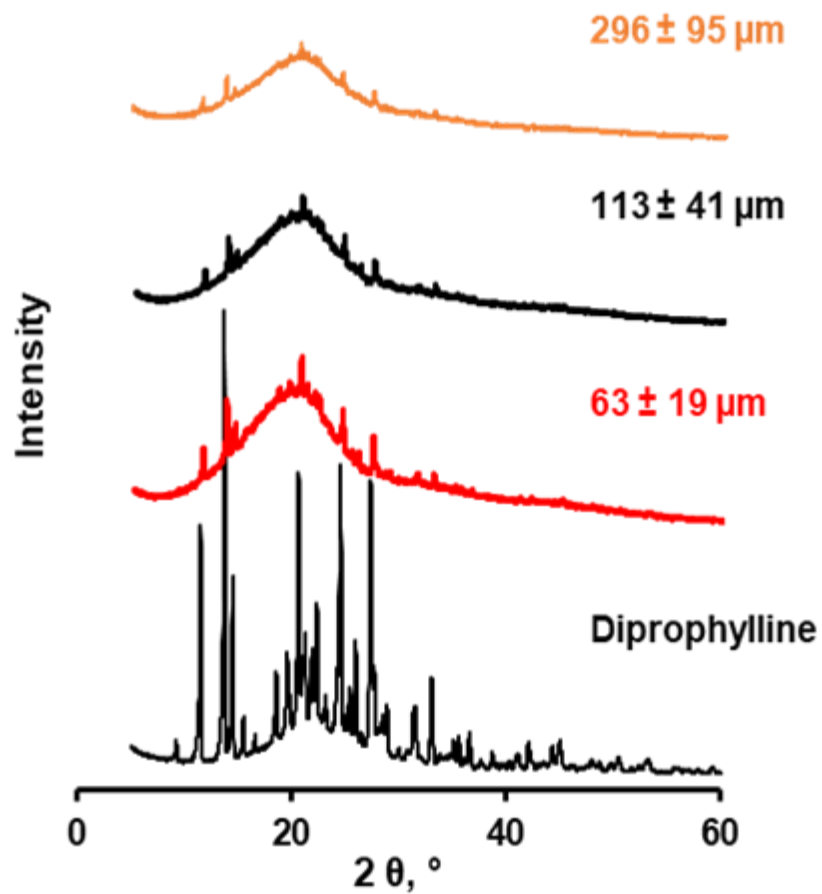
Figure III-20: X-ray diffraction patterns of ensembles of diprophylline-loaded PLGA microparticles (mean particle sizes +/- standard deviations are indicated in the diagram). For reasons of comparison, also the diffraction patterns of diprophylline powder as received) is shown.
