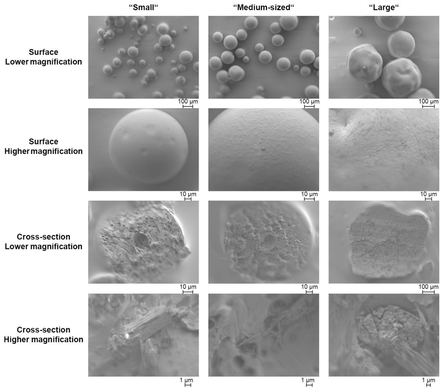
Figure II-15: SEM pictures of surfaces (lower and higher magnification) and cross-sections (lower and higher magnification) of caffeine-loaded microparticles before exposure to the release medium.
