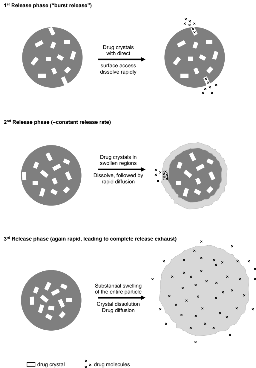
Figure III-9: Schematic illustration of the involved mass transport phenomena controlling diprophylline from the investigated PLGA microparticles during the 1st, 2nd and 3rd release phase. Non-swollen (only slightly hydrated) PLGA is marked in dark grey, swollen PLGA in light grey. Details are given in the text. Please note that the schemes are simplifications, e.g. with respect to the homogeneity of polymer swelling. Also, each microparticle has a specific, individual inner structure (e.g. location of the trapped drug crystals) and might contribute to 1 or more drug release phases.
