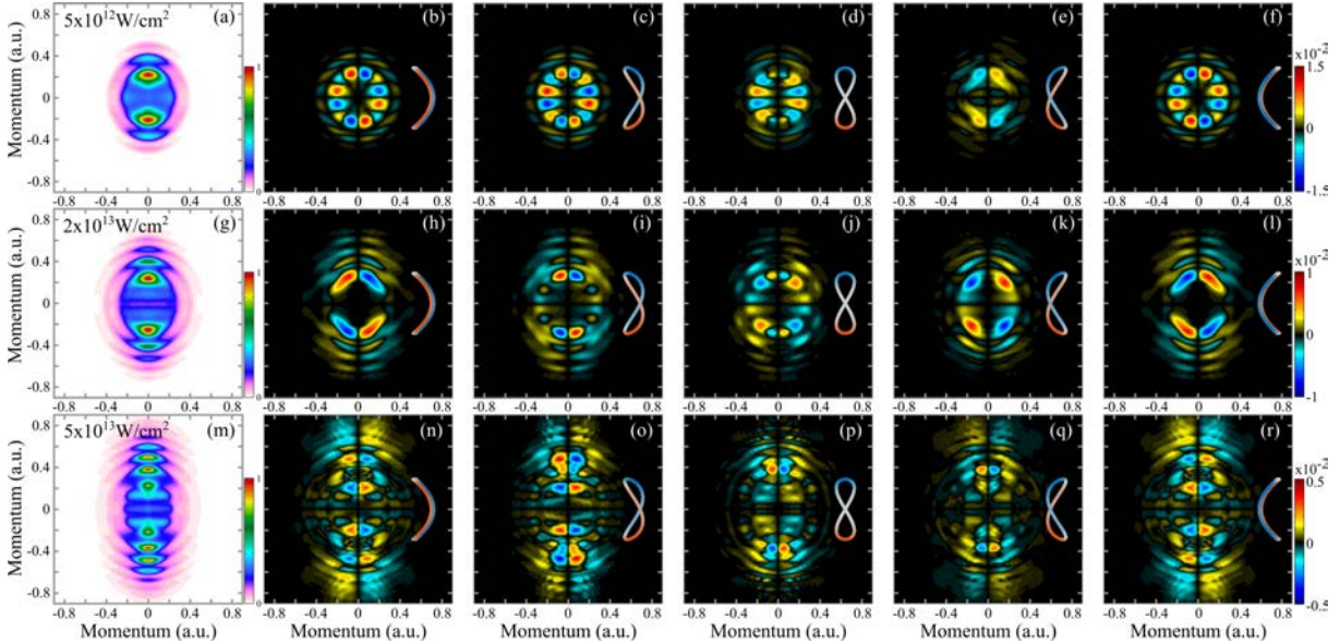
Figure 4.18 – TDSE calculations of photoionization of a toy model chiral molecule by the tailored orthogonal two-color field. (a,g,m) Projections in the (x, z) plane of the symmetric part of the photoelectron spectrum, at 5 \times 10^{12} \text{ W.cm}^{-2} (a), 2 \times 10^{13} \text{ W.cm}^{-2} (g) and 5 \times 10^{13} \text{ W.cm}^{-2} (m). (b-f),(h-l),(n-r) Corresponding projections of the ESCARGOT signal, defined as the antisymmetric part of the photoelectron distribution with respect to the propagation axis z and fundamental laser polarization axis x . The relative phase between the two components of the laser field are \varphi_{\omega/2\omega} = 0, \pi/4, \pi/2, 3\pi/4 and \pi from left to right. The shape of the two-color field, colored according to the instantaneous chirality, is shown next to each calculation.
