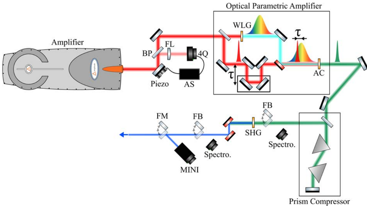
Figure 2.9 – Setup of the optical parametric amplification. The principle of the OPA is schematized and dwells on the generation of chirped white light. A fraction of the fundamental beam is used to amplify a narrow part of the spectrum, which can be chosen by tuning the relative delay \tau . The tunable pulses are then compressed in a prism compressor and undergo second harmonic generation. The pulses can be characterized both in spectrum and duration by a spectrometer and the MINI autocorrelator module. BP = Brewster plate, FL = focusing lens, 4Q = 4-quadrants, AS = active stabilization feedback, WLG = white light generation, AC = amplification crystal, FB = foldable blocker, FM = foldable mirror.
