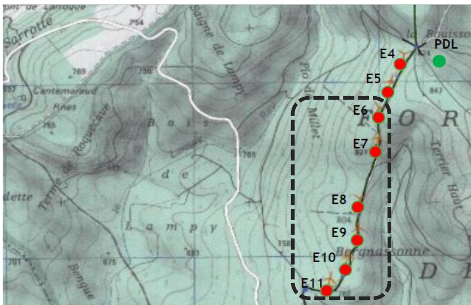
Figure 4.4b Park lay-out for Farm-S in South - France (Courtesy: Valemo) Note: Valemo only operates Turbines E6-E11
