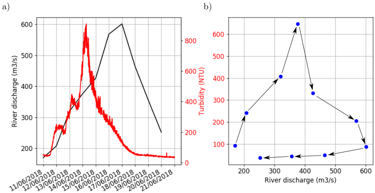
Figure 3.10: a) Turbidity (NTU) in red, and river flow ( \text{m}^3.\text{s}^{-1} ) in black, along the freshet period, b) Turbidity (NTU) in function of river flow ( \text{m}^3.\text{s}^{-1} ), based on data collected at Saint Vincent de Paul.
