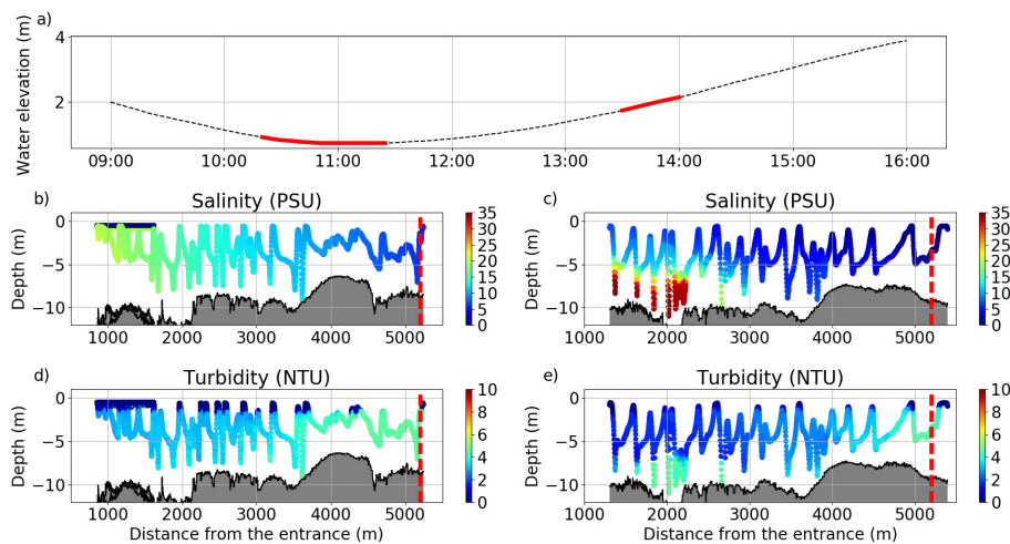
Figure 2.4: Longitudinal and vertical structure across the lower estuary from Minibat measurement during LD-ST17 experiment. (a): Water elevation with measurement periods highlighted in red. (b) and (c): salinity data for falling and rising tide. (d) and (e): turbidity data for falling and rising tide. The bed of the estuary is represented in grey. The red dashed line represents the SF2 station location.
