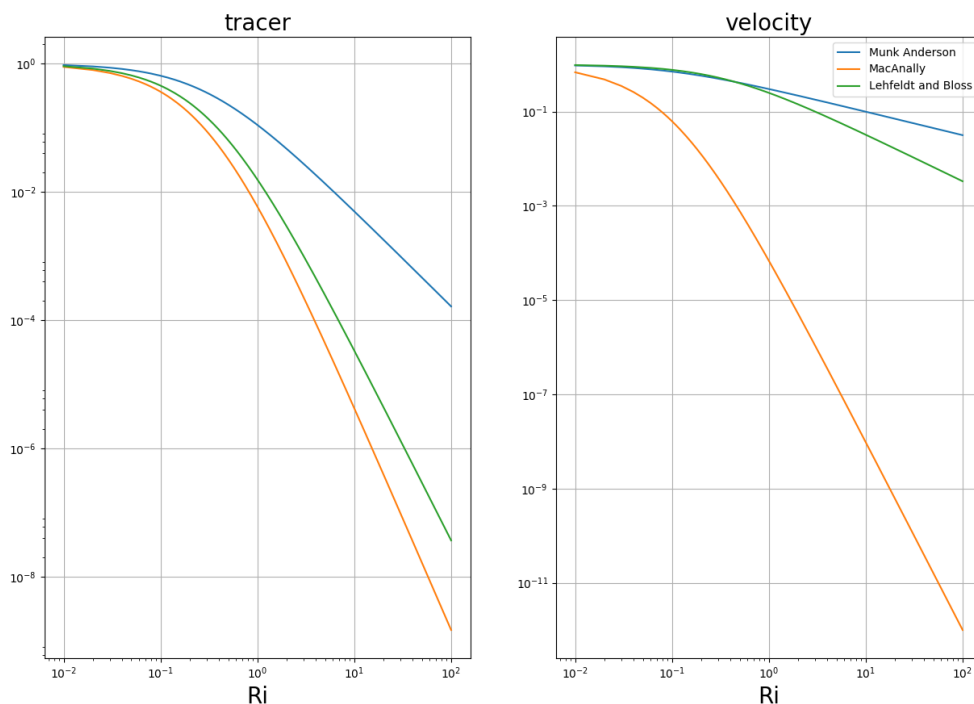
Figure 1.1: Representation of three different damping functions for tracer (on the left) and velocity (on the right) : Munk Anderson (blue line), MacAnally (orange line), and Lehfeldt &amp; Bloss (green line).
