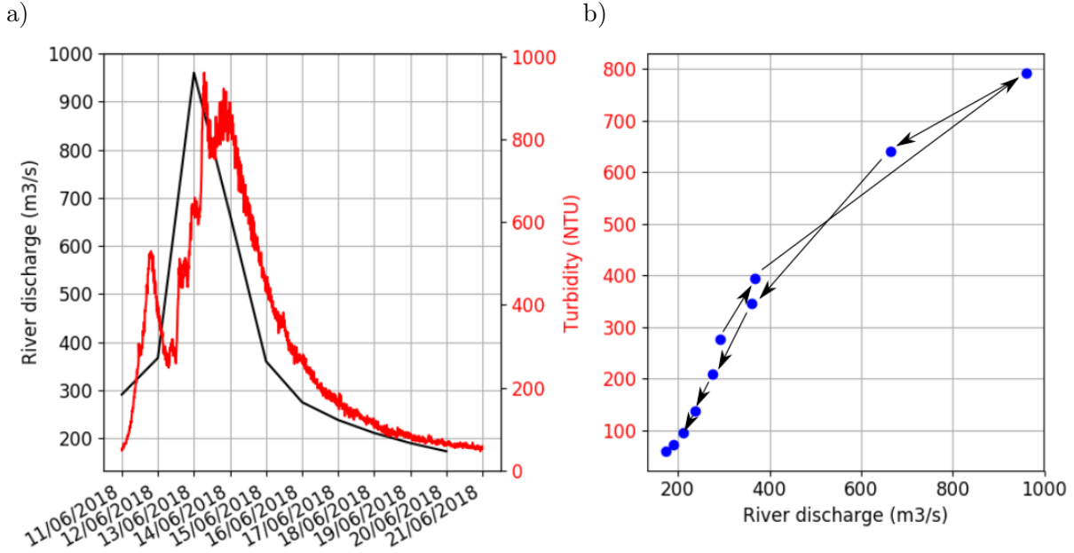
Figure 3.9: a) Turbidity (NTU) in red, and river flow ( \text{m}^3.\text{s}^{-1} ) in black, along the freshet period, b) Turbidity (NTU) in function of river flow ( \text{m}^3.\text{s}^{-1} ), based on data collected at Labatut.
