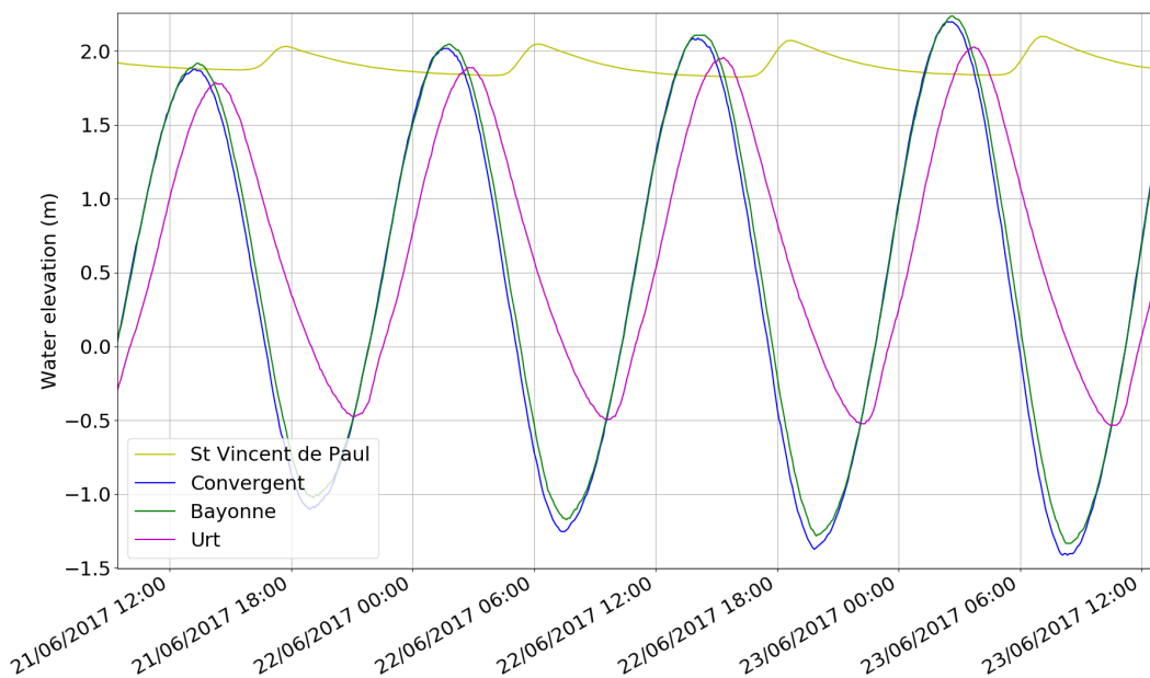
Figure 2.1: Water elevation collected at Convergent (i.e. at the estuary mouth, blue line), at Bayonne (i.e. at 6km from the estuary mouth, green line), at Urt (i.e. at about 20 km from the estuary mouth) and at St Vincent de Paul (i.e. at about 70 km from the estuary mouth), on spring tides.
