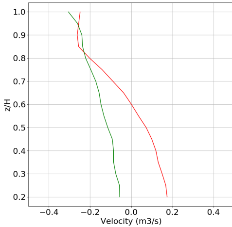
Figure 2.10: a) Tidally averaged velocity profiles for neap (full red line) and spring (full green line) tides with low river discharge, b) Tidally averaged velocity profiles for three different river flow conditions : 391 \text{ m}^3 \cdot \text{s}^{-1} (pink line), 128 \text{ m}^3 \cdot \text{s}^{-1} (black line), and 89 \text{ m}^3 \cdot \text{s}^{-1} (blue line).
