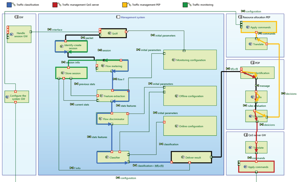
Figure 3.13: System architecture.
