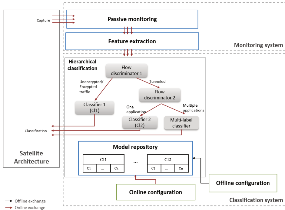
Figure 3.4: Classification framework
