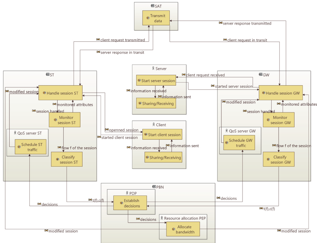
Figure 3.8: Operational context.
