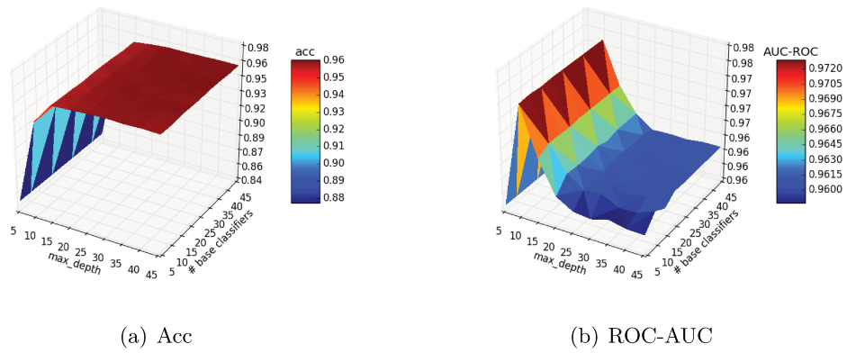
Figure C.4: Acc and ROC-AUC of the dynamic ensemble varying the number of base classifiers and the maximum depth of the DTs
