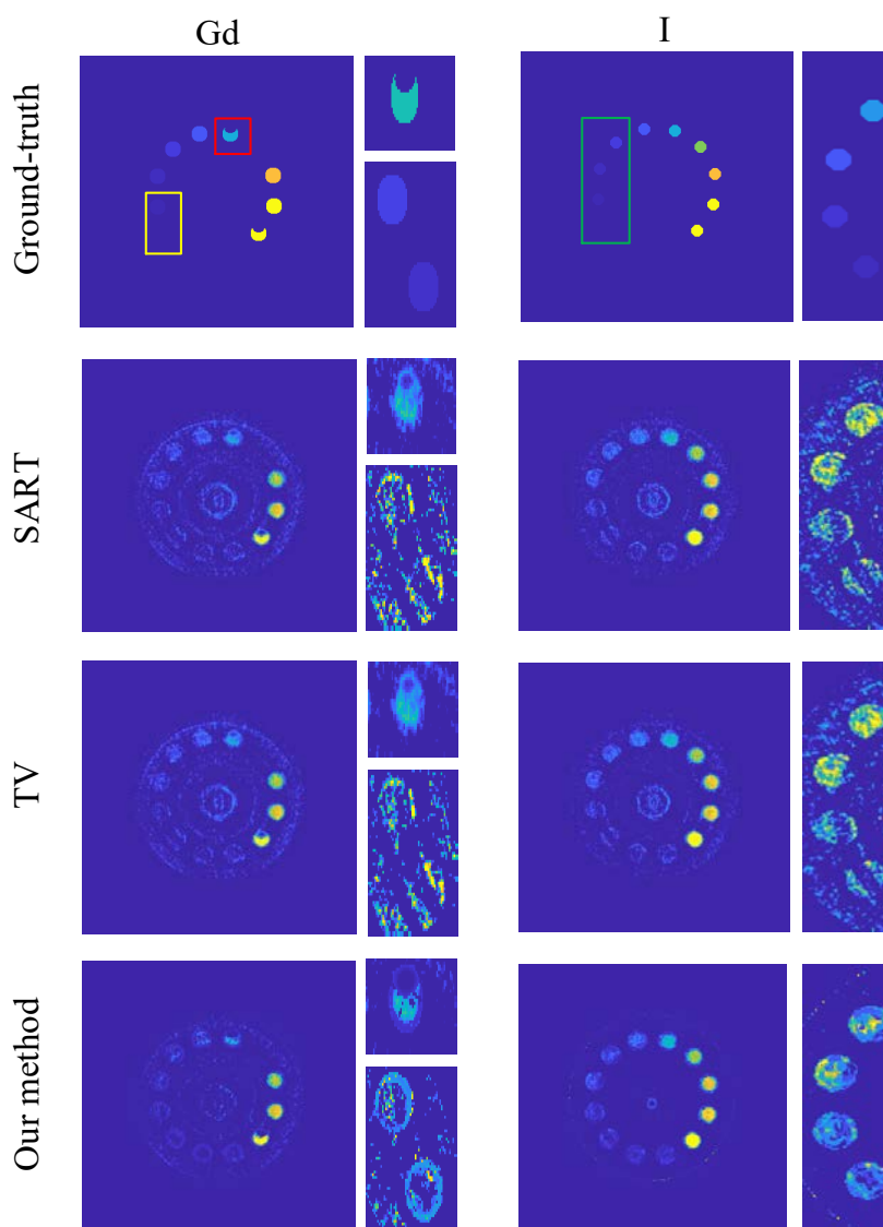
Figure 4.10 Decomposition results for physical phantom with Gd and I, respectively. The right column for each image is the region with low concentrations (yellow and green rectangle) and of special shape (the red rectangle) in the blown-up form. The images for the same region for all the methods are displayed in the same scale.
