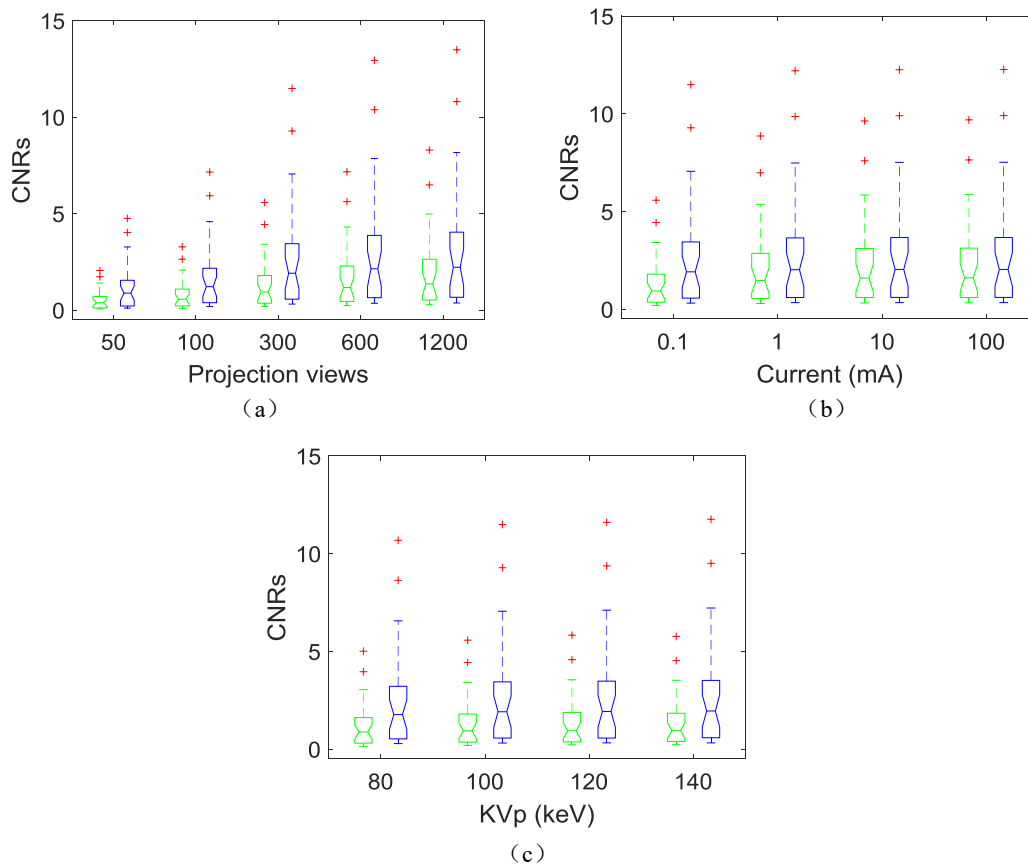
Figure 3.6 Comparison between conventional CT and aCT in terms of CNRs for: (a) different projection views; (b) different source currents; (c) different source voltages.
