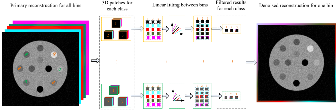
Figure 4.4 Framework of the proposed method by one energy bin mapping operation.
