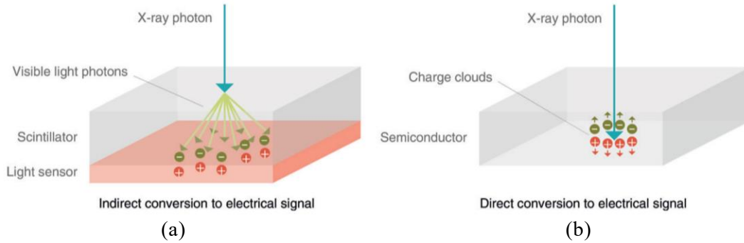
Figure 1.8 Comparison of EID and PCD (Figure form (Willemink et al. 2018)).
