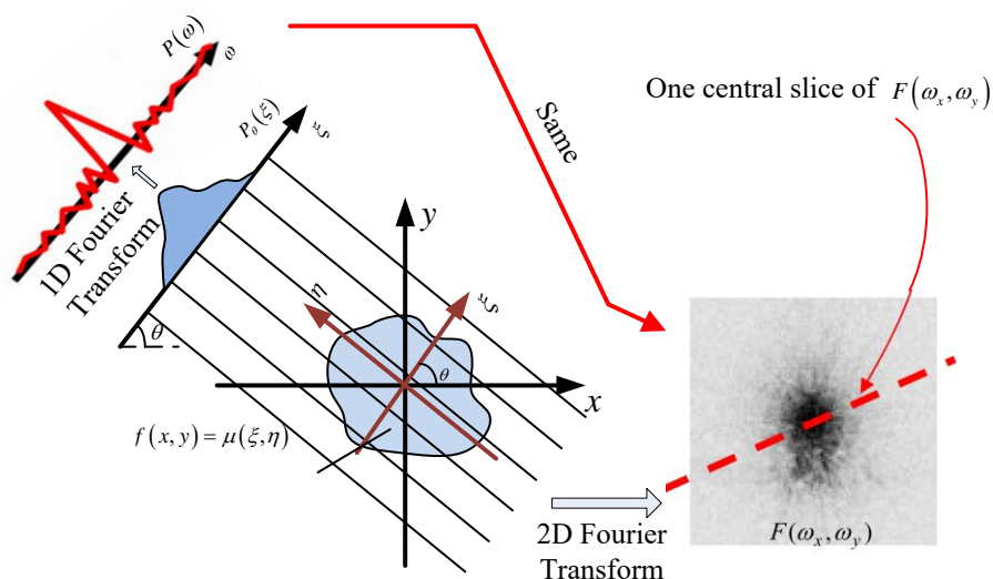
Figure 2.2 Fourier slice theorem.
