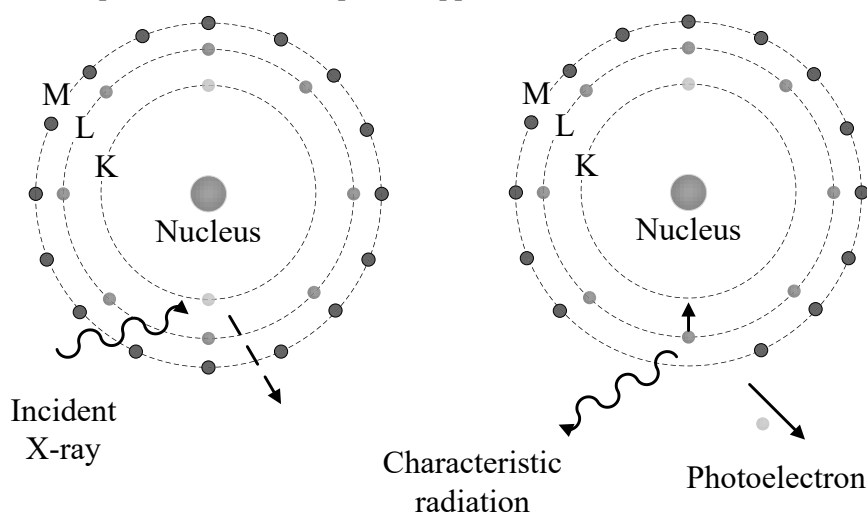
Figure 1.5 The first two stages of the photoelectric absorption. The incident X-ray interacts with the electrons in the inner shell of the atom. The energy is absorbed and ejects the photoelectron. The electron in the outer shell will transferred to fill in the vacancy in inner shell. Almost all of the energy of the incident X-ray is transferred to the ejected photoelectron (Figure inspired by (M 2008)).
