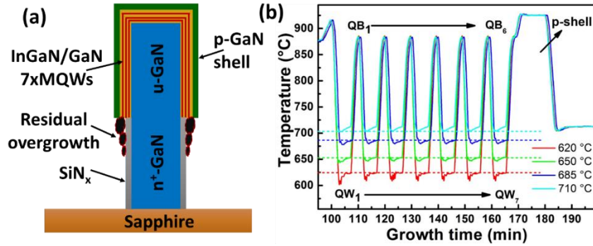
Figure 3.3: (a) Schematics of the core–shell MQWs grown on GaN wire sidewalls. (b) Growth temperature evolution as a function of growth time showing the decreasing temperature for InGaN quantum wells, keeping constant the growth temperature of the GaN barriers. ( Ref. 17 )
