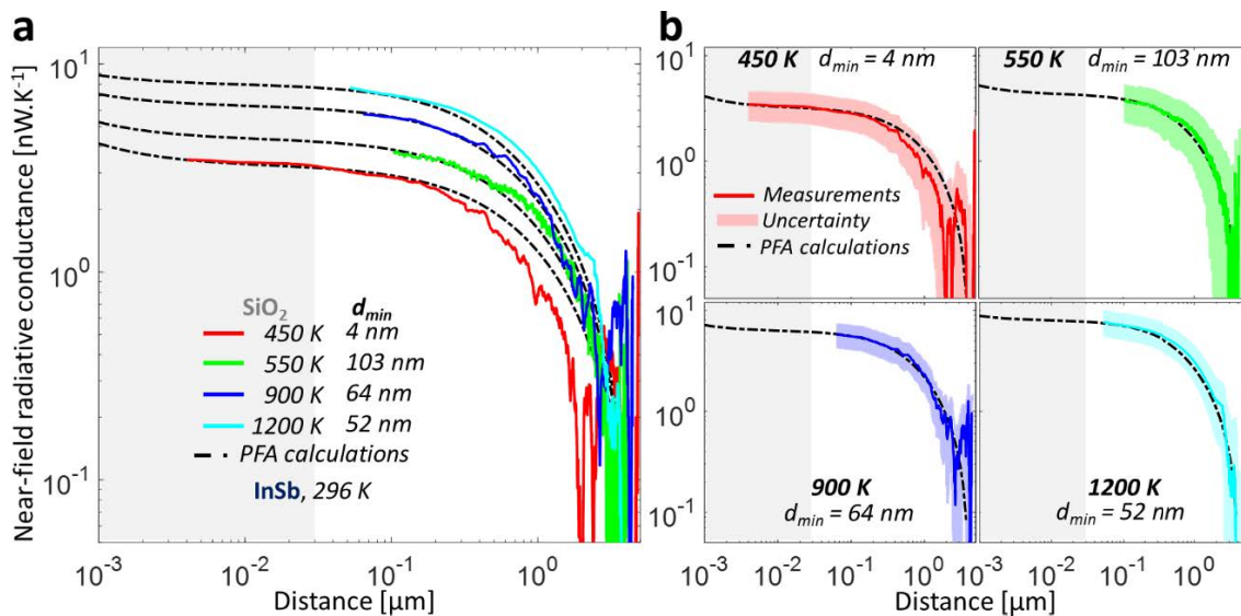
Figure IV.14: Near-field radiative conductance between a hot \text{SiO}_2 sphere and a room temperature InSb bulk flat substrate, as a function of distance and emitter temperature with adjusted minimum distances.
