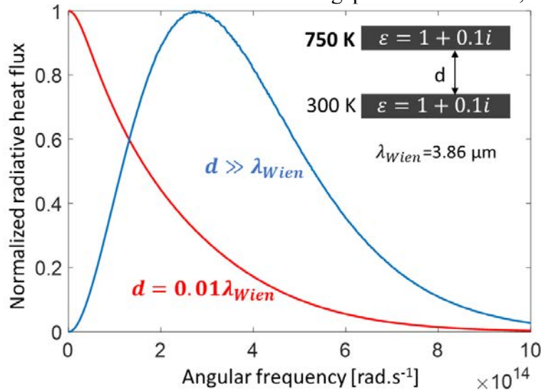
Figure V.12: Normalized radiative heat flux exchanged between two bodies at 750 and 300 K as a function of angular frequency
