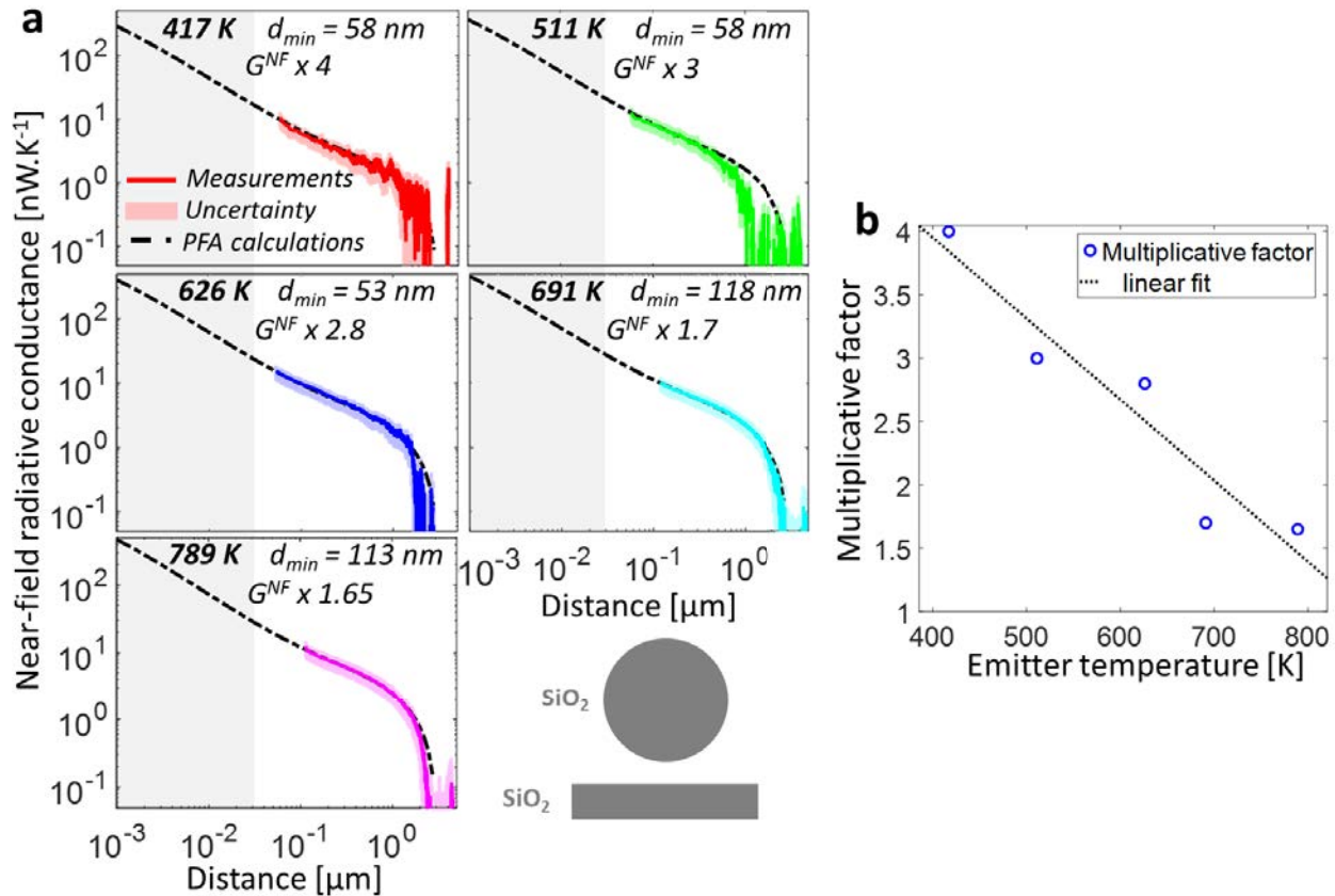
Figure IV.7: Experimental measurements for the SiO 2 -SiO 2 configuration fitted to PFA calculations.
