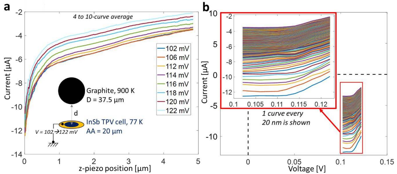
Figure VI.11: I - V curves determination as a function of z -piezo position, using approaches at different voltages
