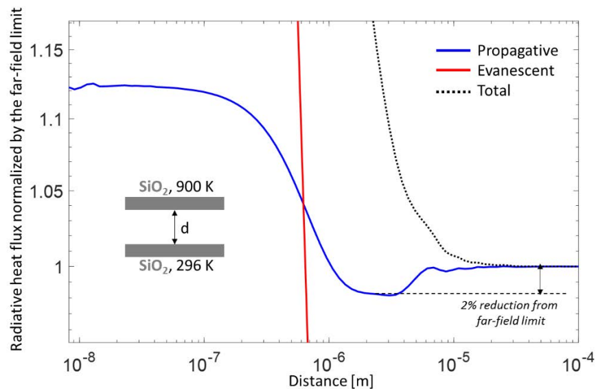
Figure I.6: Propagative and evanescent wave contribution to radiative heat transfer, normalized by the far-field limit, between two \text{SiO}_2 semi-infinite plates at 900 K and room temperature
