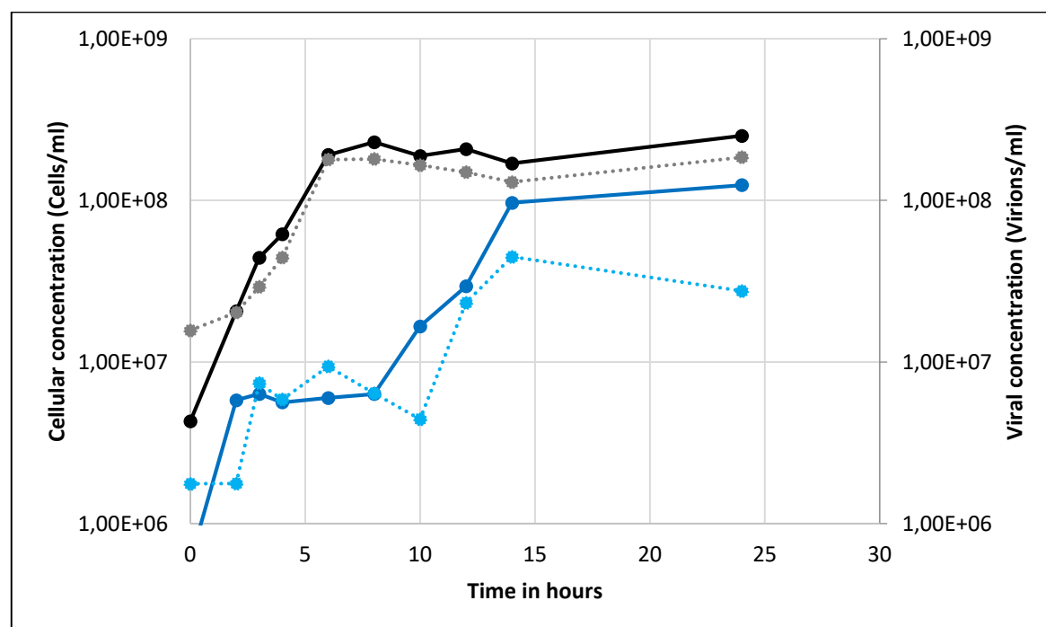
Fig. S2: MFV1 induction assays performed with BES on M. fervens and checked by flow cytometry. Typical growth curve of the host M. fervens is shown as filed circles on continuous black line. The production of MFV1 particles is shown as filed circles on dotted grey line. The growth curve under stress condition of the host M. fervens is shown as filed circles on continuous blue line. The production of MFV1 particles under stress condition is shown as filed circles on dotted blue line.
