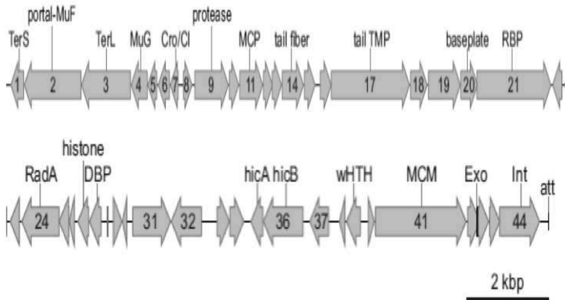
Figure 5: Genome organization of MFV1 genome. Arrows in grey with number (1 to 44) indicate predicted ORFs. The scale bar represents 2000 bp.
