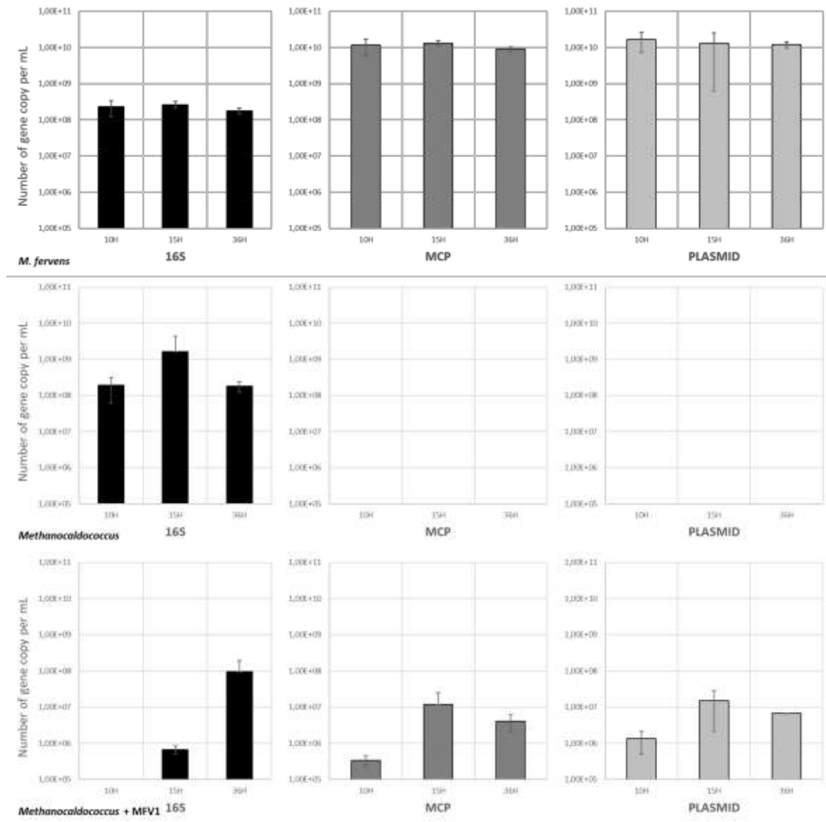
Figure 4: QPCR assays to assess changes in copy number of chromosomal, viral and plasmid DNA target genes of M. fervens , a pool of Methanocaldococcus strains, a pool of Methanocaldococcus strains infected with MFV1. The evolution of the number of 16S copy is shown with black bars. The evolution of the number of MCP (Major Capsid Plasmid) is shown with dark grey bars. The evolution of the number of plasmid gene is shown with light grey bars.
