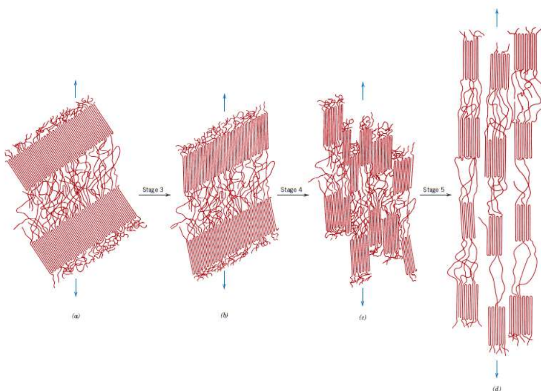
Fig. 1-8: Stages in the plastic deformation of a semicrystalline polymer. (a) Two adjacent chain-folded lamellae and interlamellar amorphous material after elastic deformation; (b) Tilting of lamellar chain folds. (c) Separation of crystalline block segments. (d) Orientation of block segments and tie chains with the tensile axis in the final plastic deformation stage, (William D. Callister 2007)
