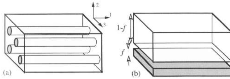
Fig. 2-39: Schematization of a ply with continuous long fibers (a) and representation of bonded slabs of fiber and matrix materials (b) (Hull and Clyne 1996)
