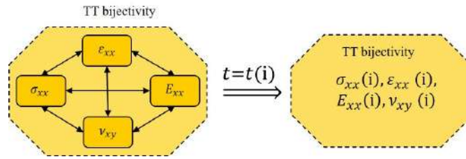
Fig. 3-34: Tensile test bijectivity property between stress, strain, secant modulus and Poisson's coefficient
