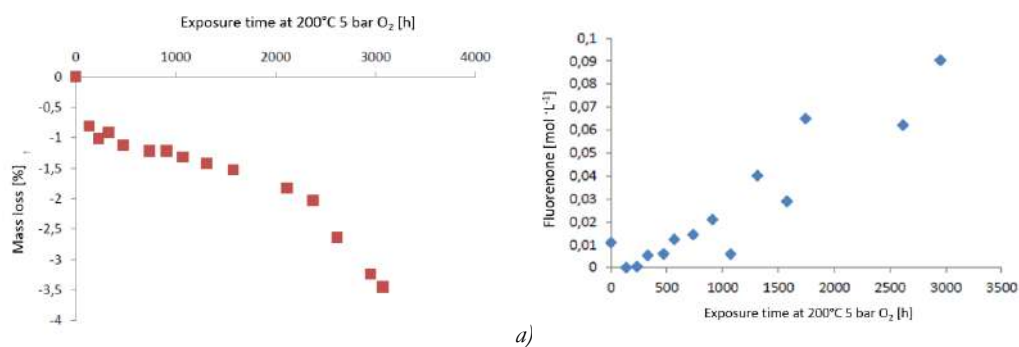
Fig. 1-15: Mass loss (a) and fluorenone concentration (b) evolution with the exposure time at 200°C under 5 bar of O 2 (Roland and Fayolle 2020)
