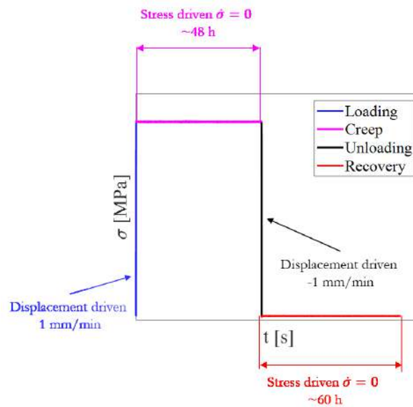
Fig. 2-9: Creep-recovery test protocol
