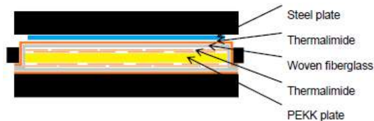
Fig. 2-2: PEKK plates environment for crystallization from the melt (Tanguy Choupin 2018)
