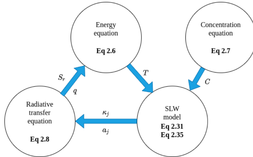
Figure 3.5: Implantation of SLW model in the Code Saturne
