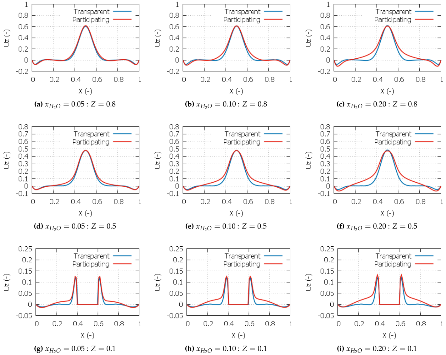
Figure 4.29: Profiles of vertical velocities \frac{w}{U_{ref}} at different Z -crosslines in the median plane ( Y = 0.5 ) at different concentration of water vapor.
