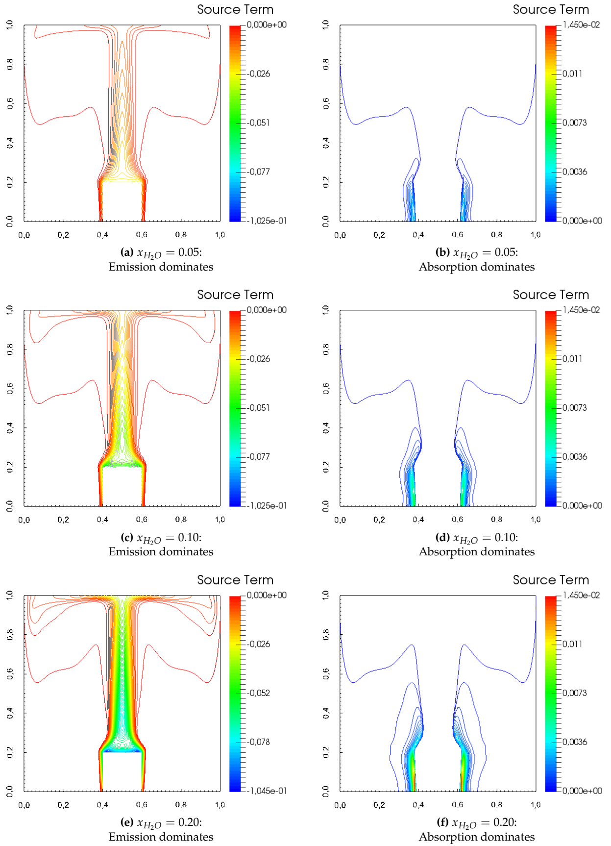
Figure 5.61: Distribution of radiative source term in the median plane ( Y = 0.5 ) at different mole fractions of water vapor. Sources are normalized by 4\sigma T_{ref}^4/L .
