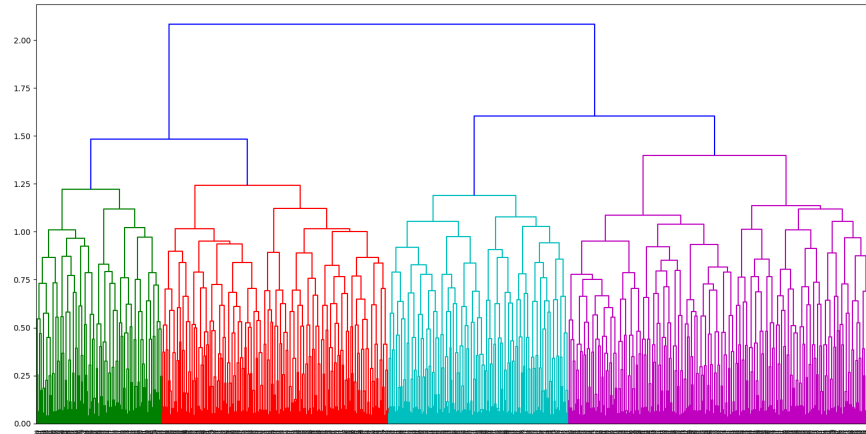
FIGURE 8 – Dendrogramme Clients
