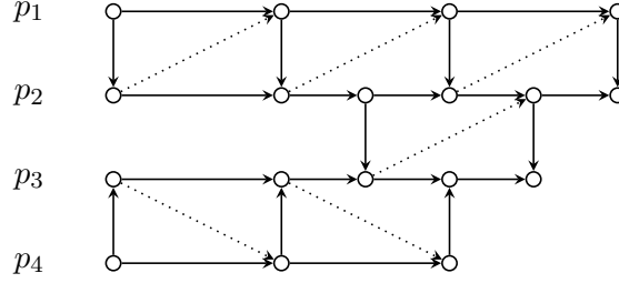
Figure 6.1: The relation rev_B for B = 1 .
