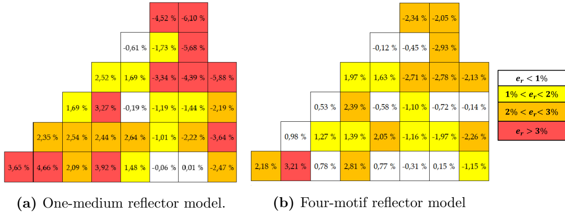
Figure 5.10. Effects of reflector modeling in the two-step scheme. Assembly power errors.
