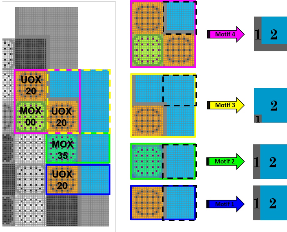
Figure 5.8. Reflector homogenization. Four-motif model.
