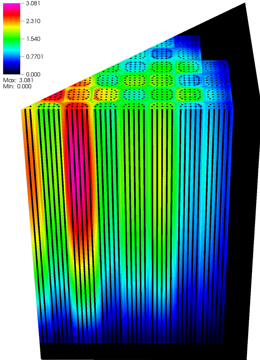
Figure 6.2. 3D Reference power distribution normalized such that the average power per pin-cell equals one. For a better representation, the core geometry has been cut at the height z = 260\text{cm} .
