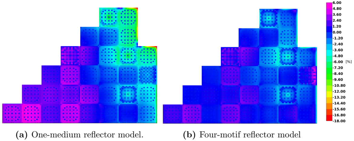
Figure 5.9. Effects of reflector modeling in the two-step scheme. Pin power errors.
