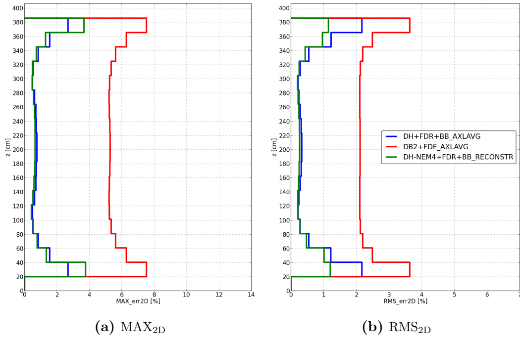
Figure 6.6. MAX and RMS of the relative error of the average power per pin and per axial layer for problem 1. The latter has been computed by averaging along the axial layer the solution of DH+FDR+BB and DB2+FDF, while using the local transport solution in DH-NEM+FDR+BB. (The legend is used once for both figures).
