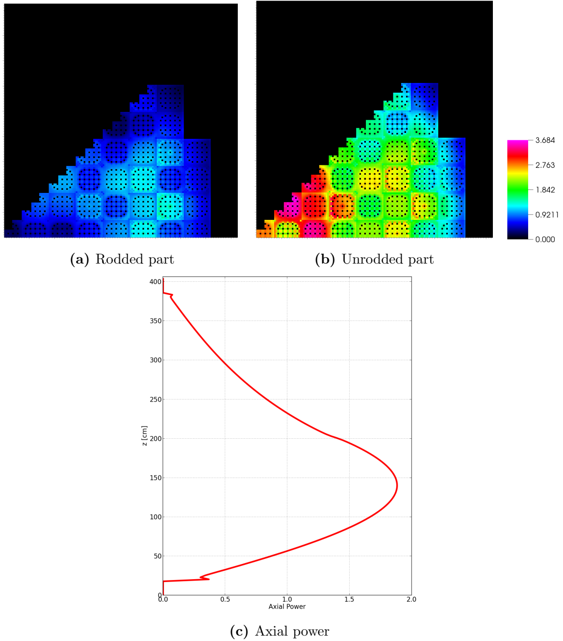
Figure 6.8. Radial power distribution on the (a) top (rodded) and (b) bottom (unrodded) parts of the core. The two radial planes are located at a height of 260cm and 140cm respectively for the top and bottom core parts. (c) Radially integrated reference power distribution such that the average power per unit cell equals one.
