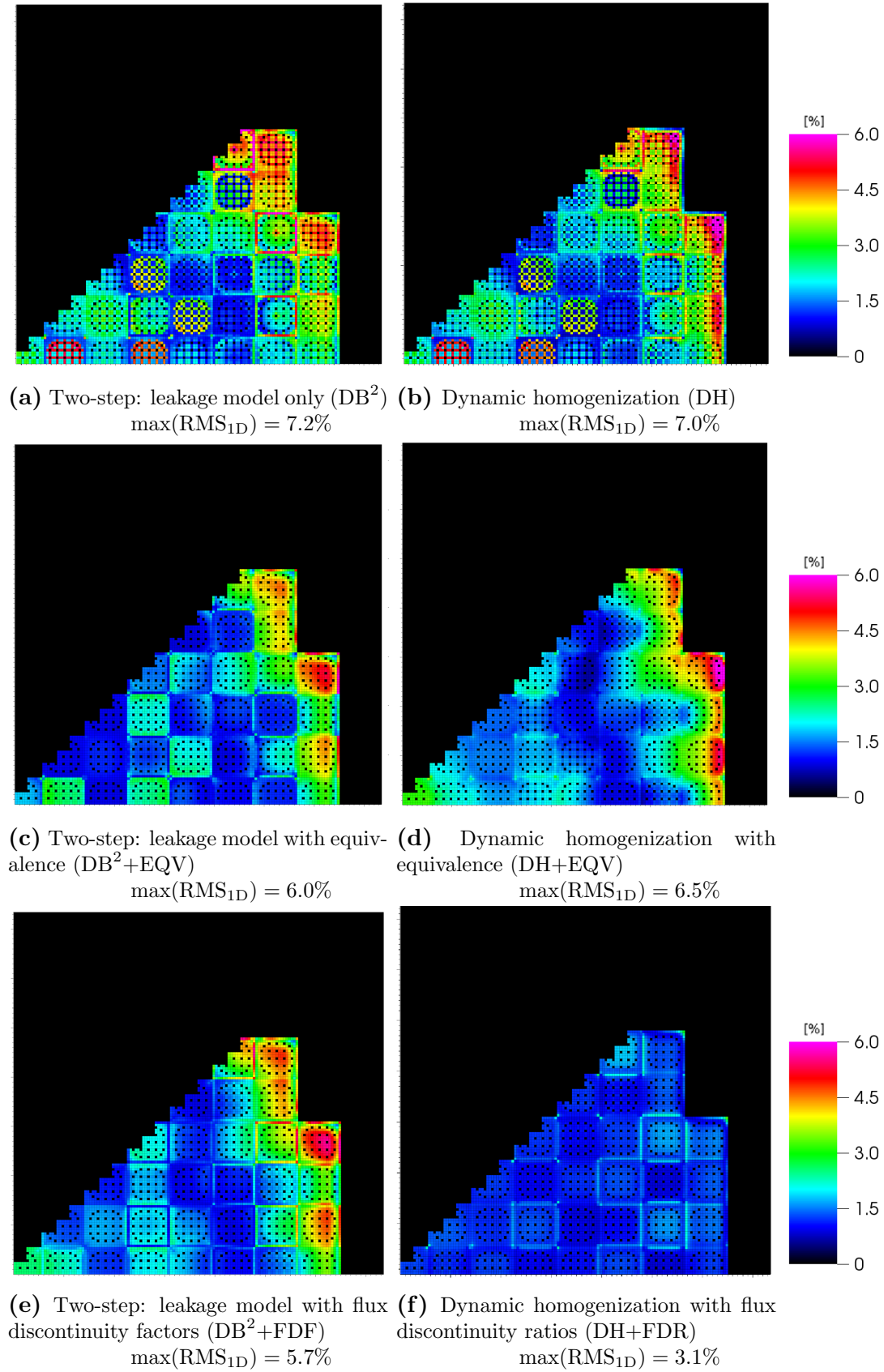
Figure 6.3. Root mean square of axial power errors per pin ( RMS_{1D} ) for problem 1, as defined in Equation (6.25). For each case we have given the maximum value.
