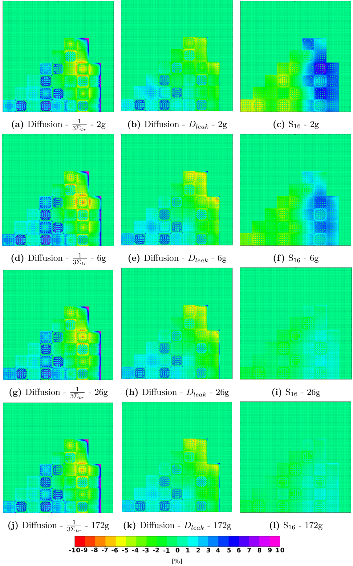
Figure 5.6. Pin power relative error of the DH solution with pin-by-pin flux-volume homogenization.
