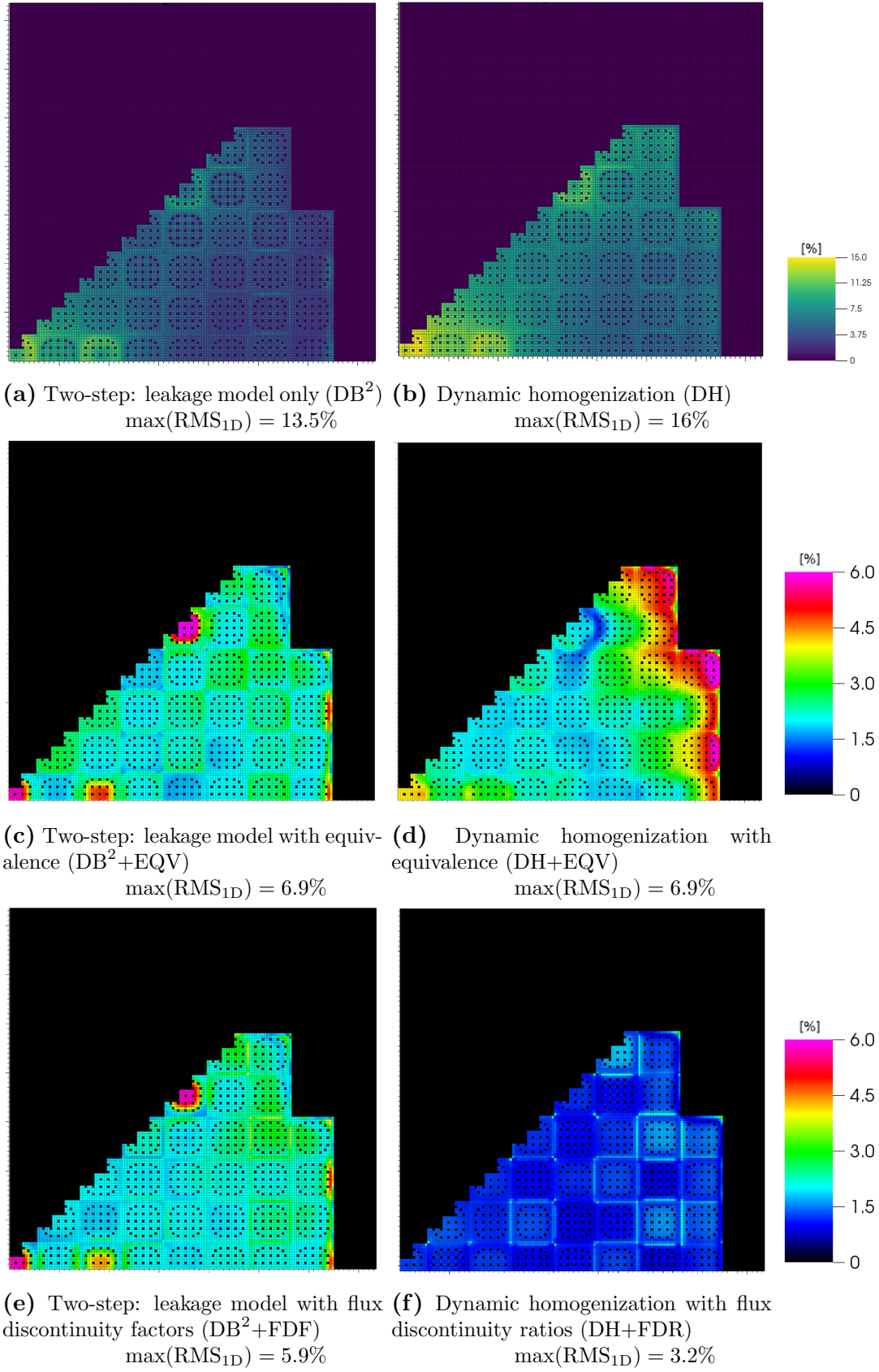
Figure 6.11. Root mean square of axial power errors per pin ( RMS_{1D} ) for problem 2, as defined in Equation (6.25). For each case we have given the maximum value.
