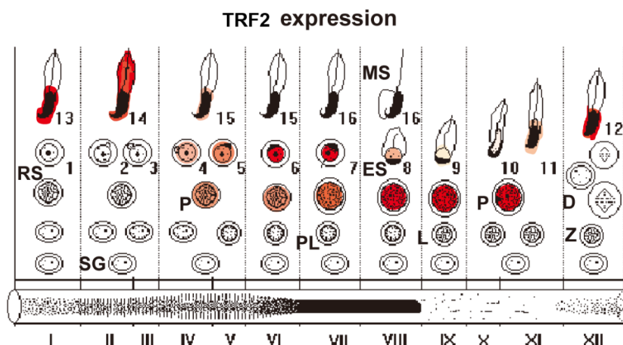
Figure 3-4: Dynamic expression of TRF2 during spermatogenesis. SG, spermatogonia; PL, preleptotene; L, leptotene; Z, zygotene; P, pachytene; D, diakinetic; RS, round spermatids; ES, elongating spermatids; MS, mature spermatozoa. Adapted from (Martianov et al., 2002a).
