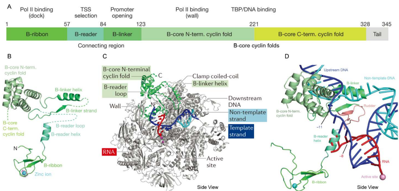
Figure 2-8: Structure of the yeast Pol II-TFIIB complex. (A) TFIIB domain organization. (B) Ribbon model of TFIIB. (C) Ribbon model of Pol II-TFIIB complex. (D) Clash of RNA stand with the B-reader. Adapted from (Kostrewa et al., 2009; Sainsbury et al., 2015)
