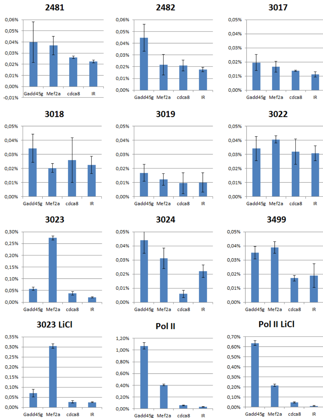
Figure 1-5: TBP2 antibody validation by ChIP. Pol II ChIP was performed as a positive control. '3023 LiCl' means that an additional harsh wash with LiCl buffer was performed during the ChIP.
