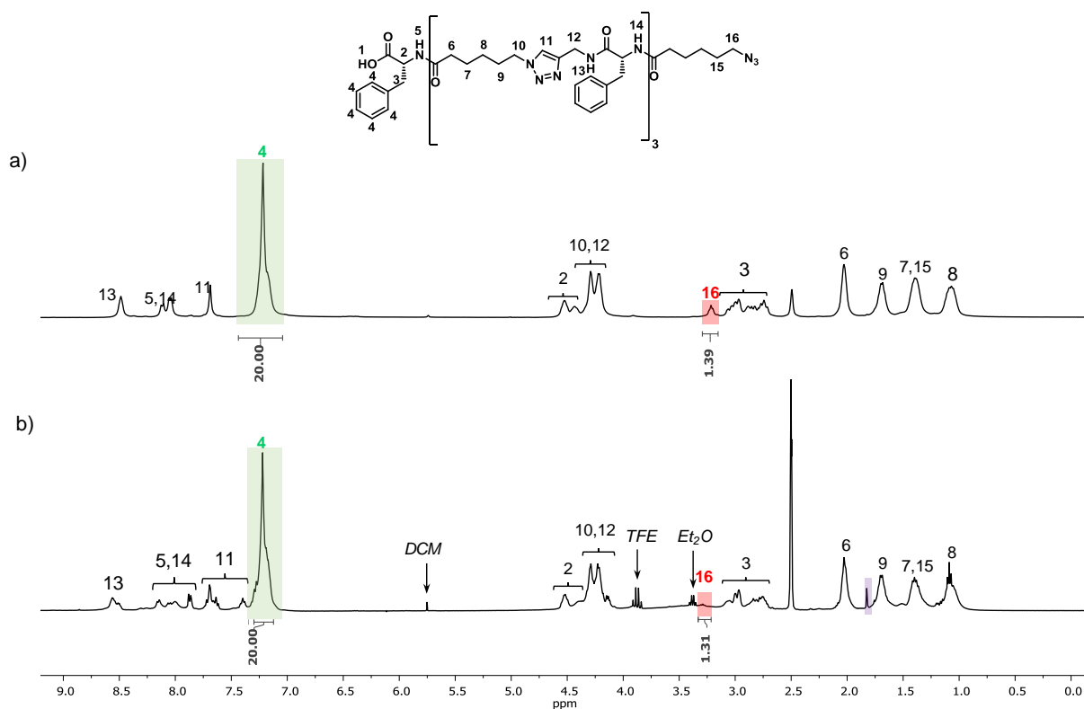
Figure II.9: ^1\text{H} NMR spectra in \text{DMSO-d}_6 of \text{Fh}\cdot\text{Fh}\cdot\text{Fh}\cdot\text{Fh} synthesized (a) using normal conditions and (b) while performing pre-activation of the carboxylic acids (unidentified peaks in purple).
