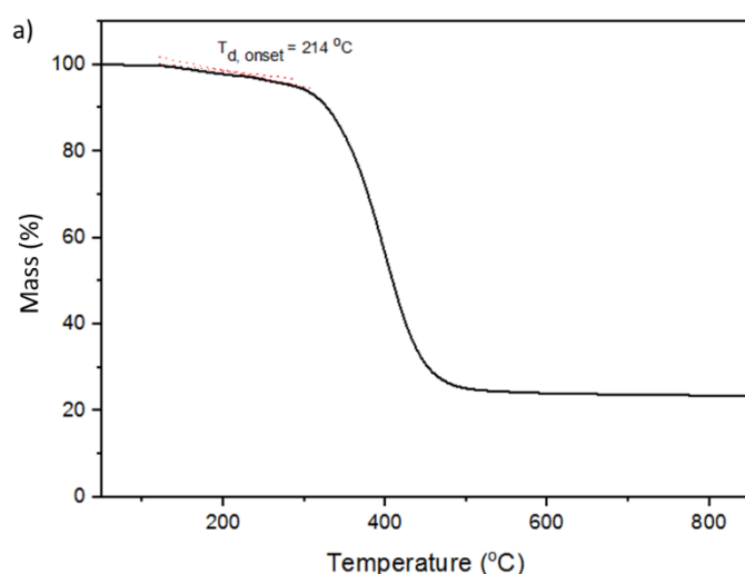
Figure III.2: TGA analyses: a) thermogram of FFFFh•FFFFh•FFFFh•FFFFh ( N_2 , flow rate: 10 \text{ cm}^3 \cdot \text{min}^{-1} , heating rate: 50 \text{ }^\circ\text{C} \cdot \text{min}^{-1} ) and b) T_{d, \text{onset}} values for the molecules used for adsorption studies (* from Seleem et al. [III.8]).
