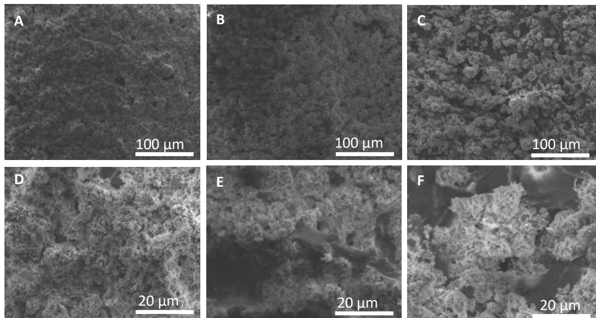
Figure 3-13. SEM images of coated surfaces. A. Latex r4 at 400x magnification ; B. CNF-AKD r20 at 400x magnification; C. CNF-APMS r10 at 400x magnification; D. Latex r4 at 2000x magnification; E. CNF-AKD r20 at 2000x magnification ; F. CNF-APMS r10 at 2000x magnification
