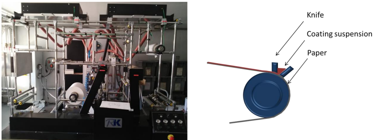
Figure 3-15. Picture of the pilot coater used in the experiment and schematic representation on the coating module.
