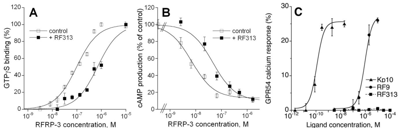
Fig. 2. Assessment of in vitro pharmacological properties of RF313 and RF9 on NPFF1R and Kiss1R. A: Stimulation of [ 35 S]-GTP \gamma S binding by RFRP-3 on membranes from CHO cells expressing human NPFF1 receptors. RF313 (10 \mu M) shifted the EC 50 values for RFRP-3 from 98 \pm 10 to 695 \pm 95 nM. Data are expressed as percentages of maximal [ 35 S]-GTP \gamma S binding and are mean \pm S.E. values for two separate experiments in triplicate. B: Reversal of RFRP-3-induced inhibition of forskolin-induced cAMP accumulation in CHO-hNPFF1R cells. RF313 (10 \mu M) shifted the EC 50 values for RFRP-3 from 6.9 \pm 1.1 to 47 \pm 12 nM. Data are expressed as percentages of maximal cAMP levels and represent mean \pm S.E.M values for four separate experiments in triplicate. C: Effect of Kp-10, RF9 and RF313 on calcium mobilization in Kiss1R expressing cells. Peak response amplitudes were normalized to basal and maximal (digitonin-permeabilized cells) fluorescence levels. Data points are from a representative experiment performed in duplicate. EC 50 \pm S.E. values for Kp-10 ( 0.1 \pm 0.025 nM) and RF9 ( 1.3 \pm 0.5 nM) are from two experiments performed in triplicate.
