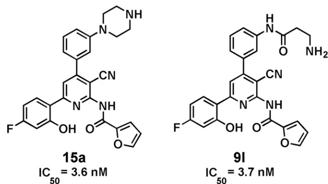
Fig. 5. Non-peptidic Kiss1R antagonists. IC_{50} values for compounds 15a (Kobayashi et al., 2010b) and 91 (Kobayashi et al., 2010a) were defined as the concentrations that displaced half specific [ 125 I]-Kp14 binding on membranes of Kiss1R-expressing CHO cells.
